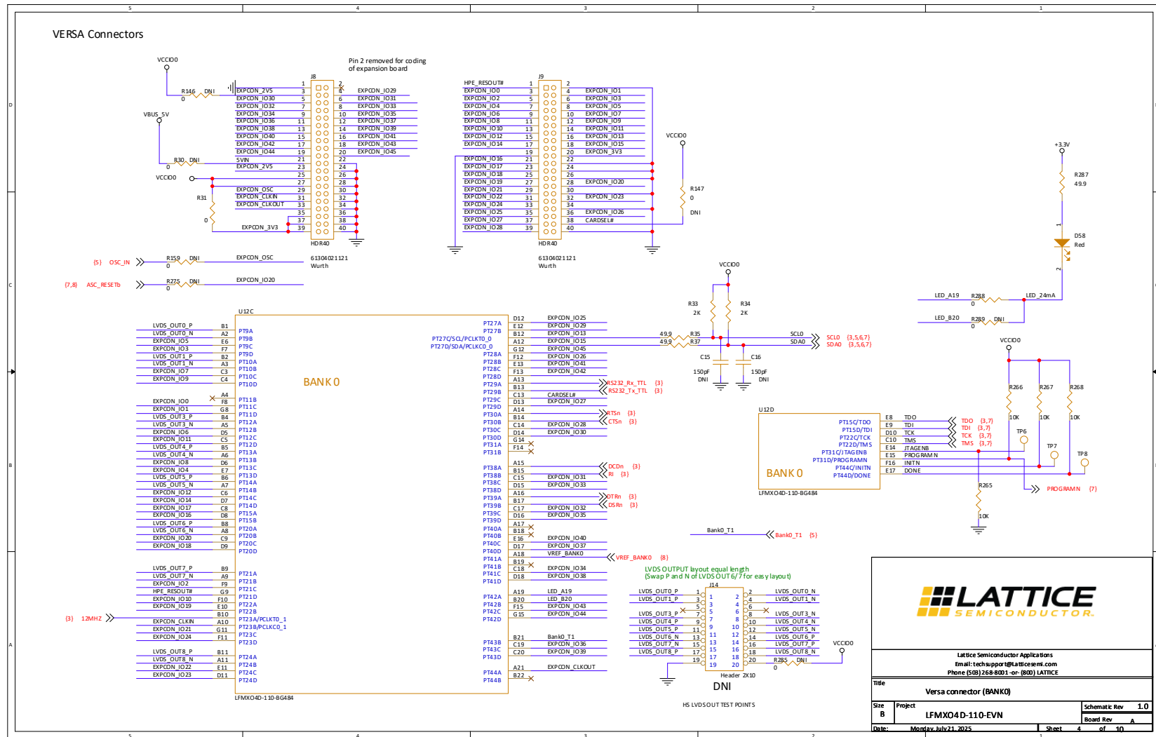
Figure A.4. VERSA Headers (BANK0)
