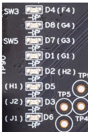
Figure 7.4. Board LEDs
