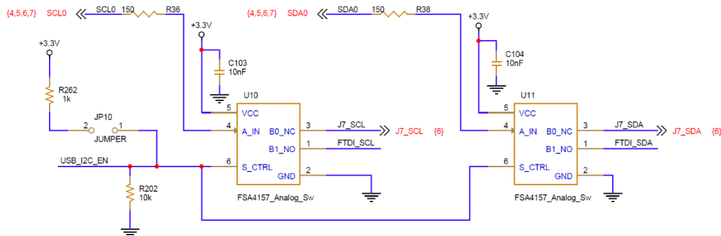
Figure 6.2. I2C MUX Circuits
