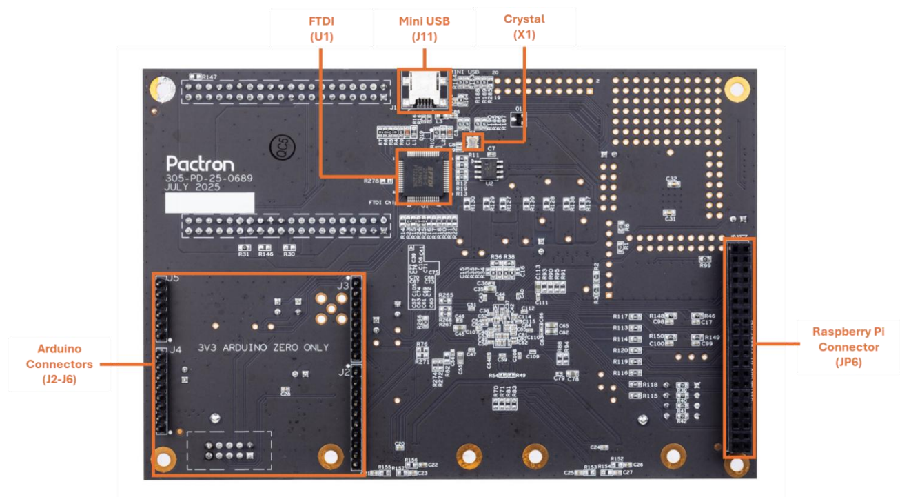
Figure 1.2. Bottom View of MachXO4 RoT Development Board
