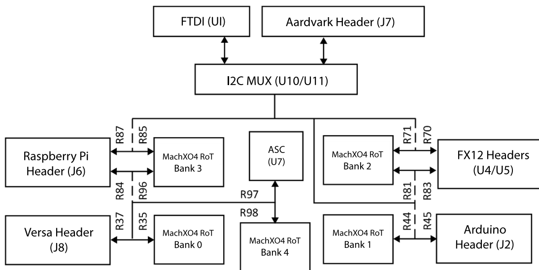
Figure 6.1. I2C Topology
