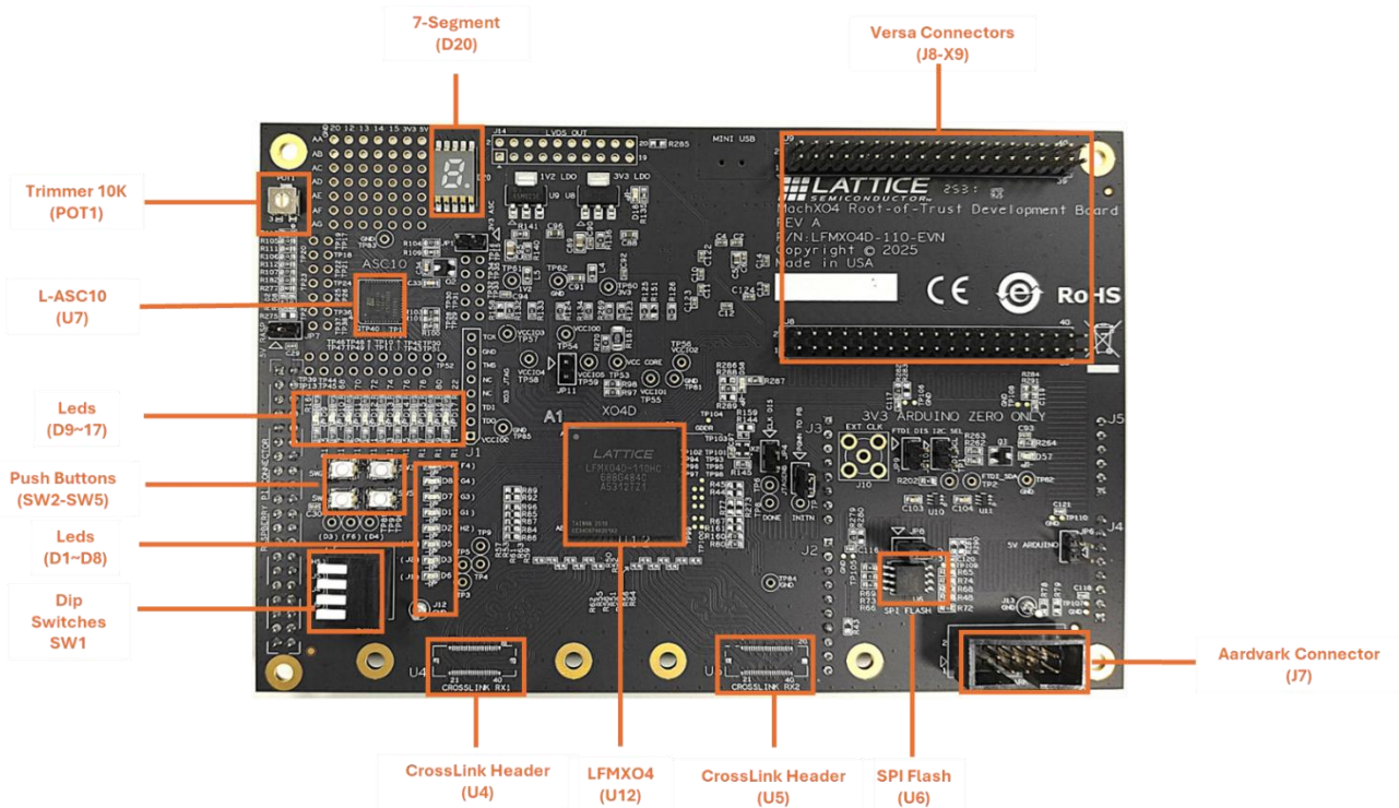
Figure 1.1. Top View of MachXO4 RoT Development Board
