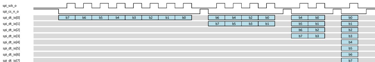
Figure 2.13. Byte Transfer across Different I/O Widths
