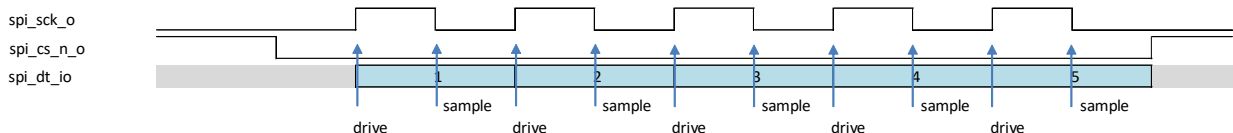
Figure 2.10. SPI Transfer Mode 1 (cpol = 0, cpha = 1)
