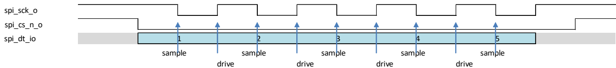
Figure 2.11. SPI Transfer Mode 2 (cpol = 1, cpha = 0)
