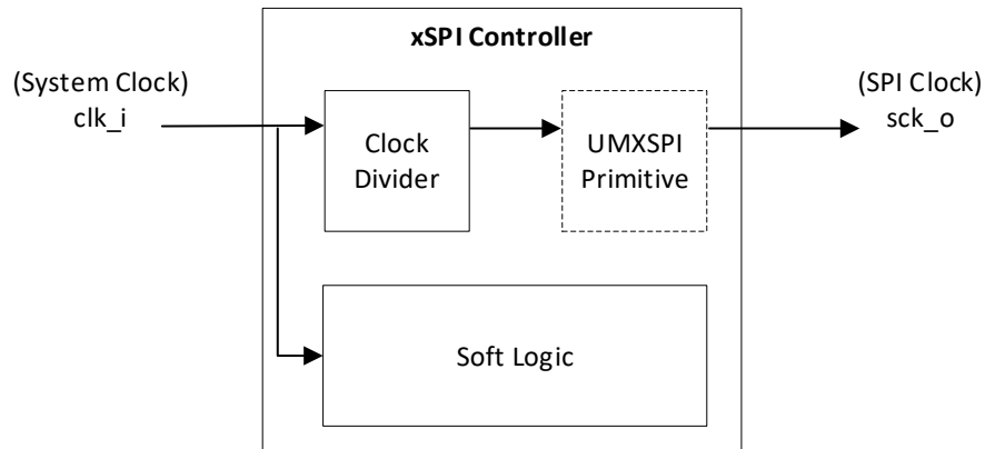
Figure 2.2. xSPI Controller IP (External SPI) Clock Domain Block Diagram
