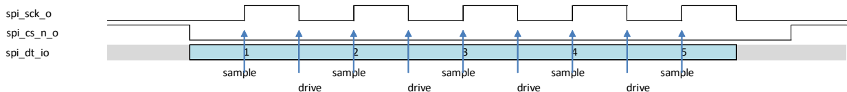
Figure 2.9. SPI Transfer Mode 0 (cpol = 0, cpha = 0)
