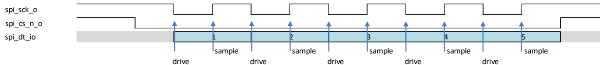
Figure 2.12. SPI Transfer Mode 3 (cpol = 1, cpha = 1)
