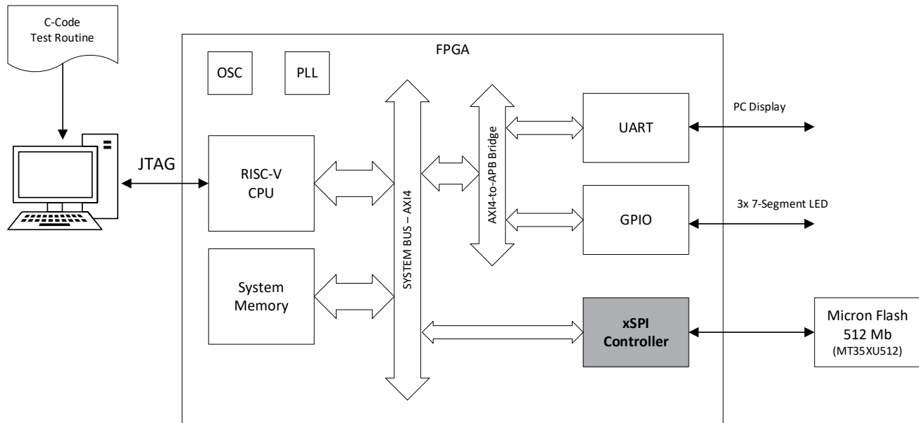
Figure 6.1. xSPI Controller Example Design Block Diagram
