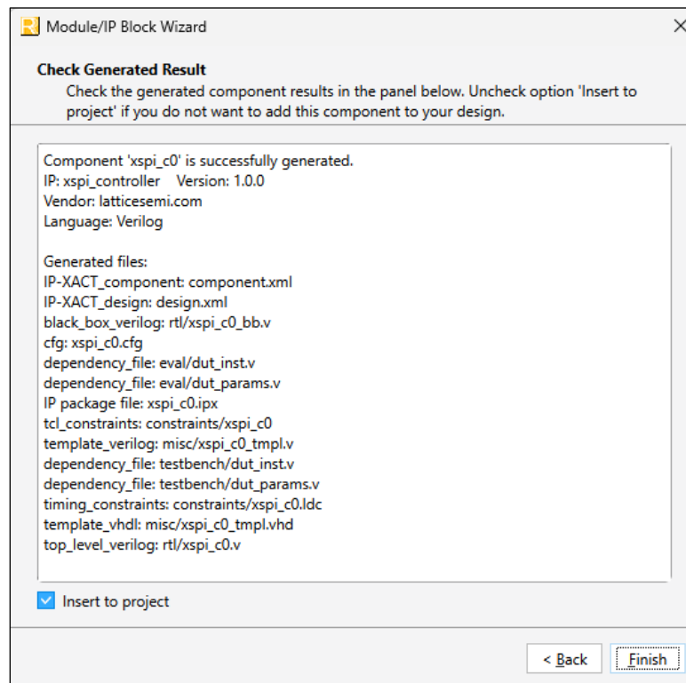
Figure 7.5. Check Generated Result
