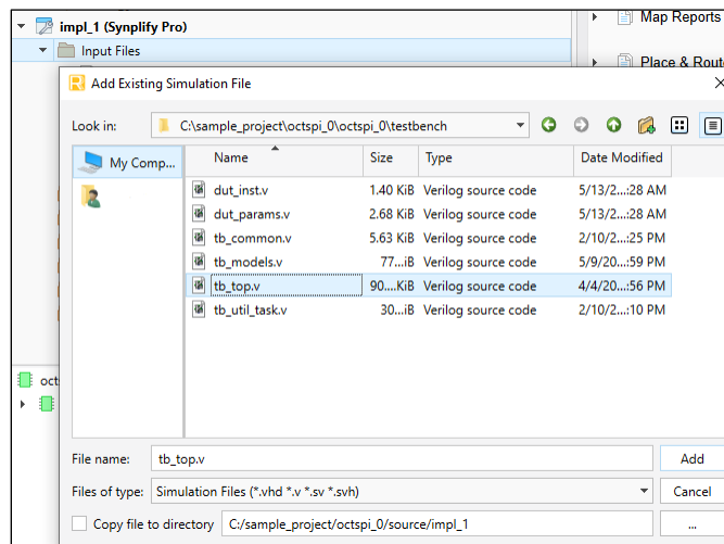
Figure 7.7. Adding Existing Simulation File (View 2)
