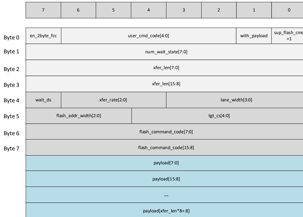
Figure 2.6. Supported Flash Command Packet with 2DW Header
