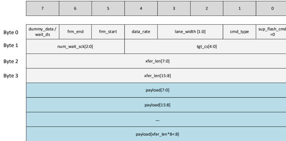
Figure 2.5. Generic SPI Command Packet
