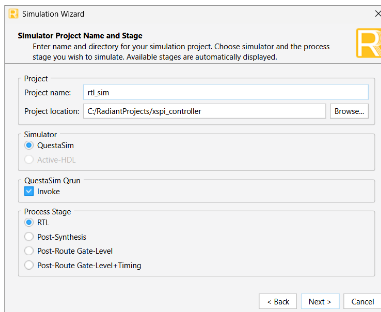
Figure 7.9. Simulation Wizard (View 2)
