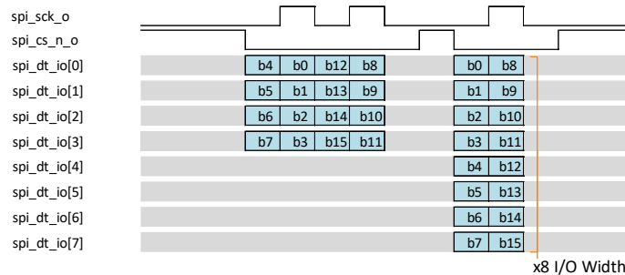
Figure 2.14. Byte Transfer in DTR Mode across x4 and x8 I/O Widths
