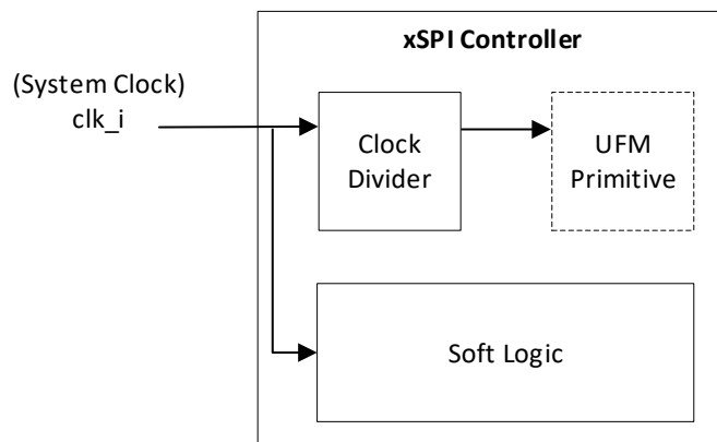
Figure 2.3. xSPI Controller IP (Internal Flash) Clock Domain Block Diagram
