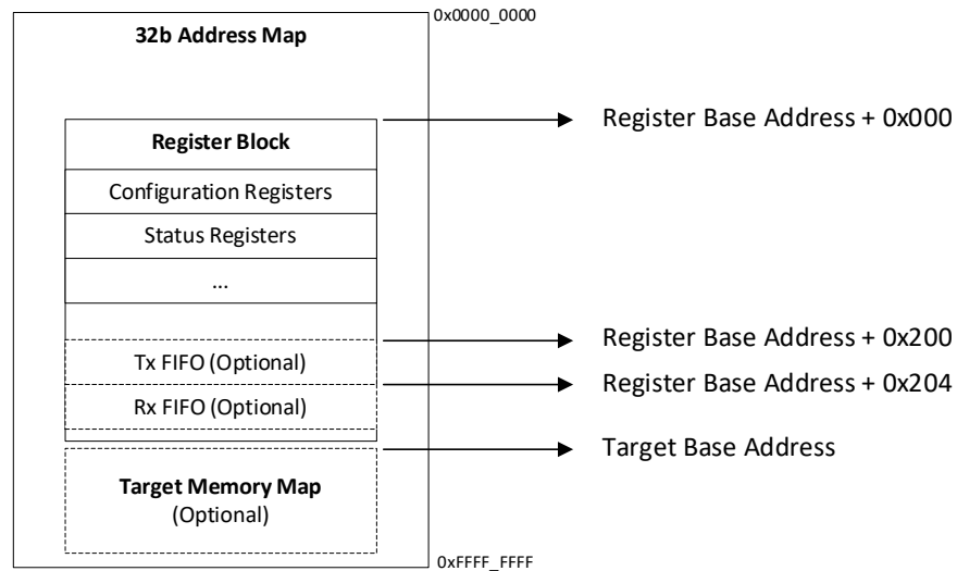
Figure 2.4. xSPI Controller Address Space Mapping
