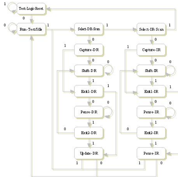
Figure 49: Shift Registers
