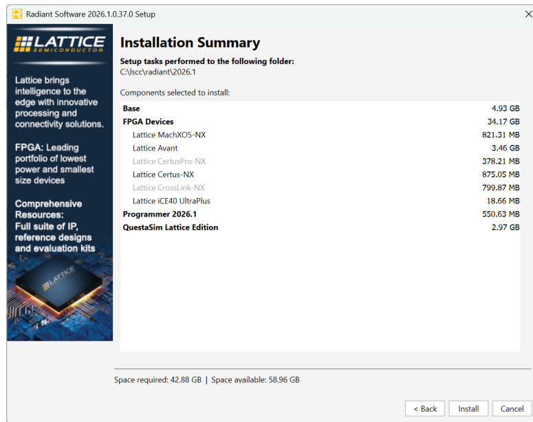
Figure 8: Installation Summary
