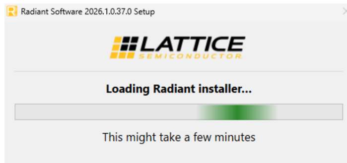
Figure 2: Setup Loader
