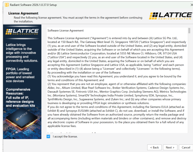
Figure 6: License Agreement
