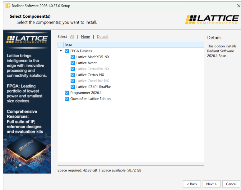
Figure 5: Select Component(s)
