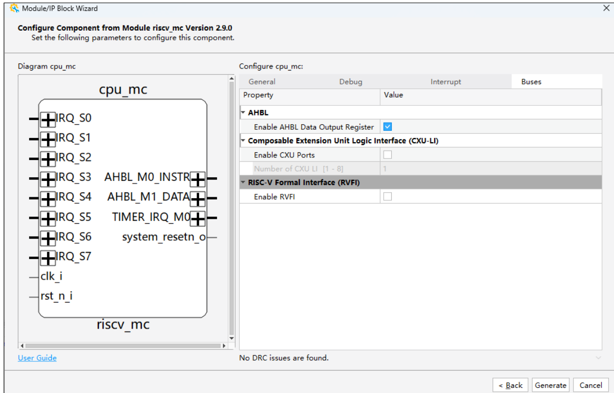
Figure 2.15. Buses Tab
