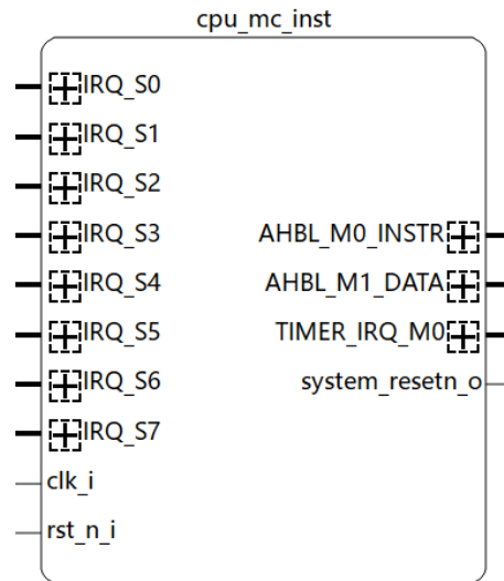
Figure 3.5. Generated Instance
