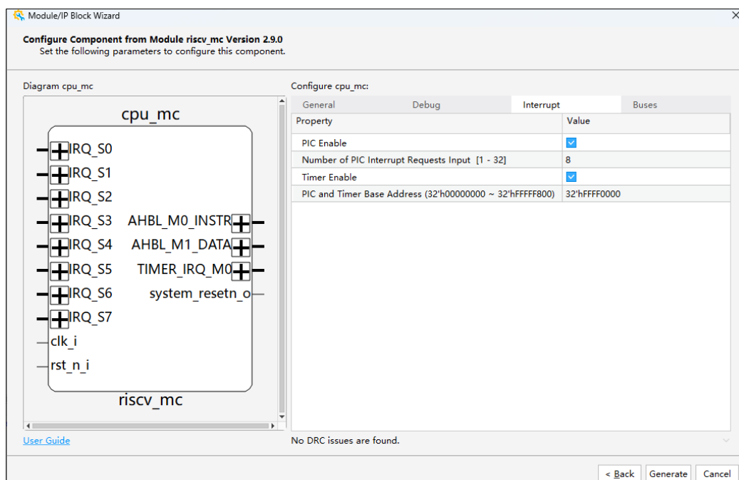
Figure 2.12. Interrupt Tab
