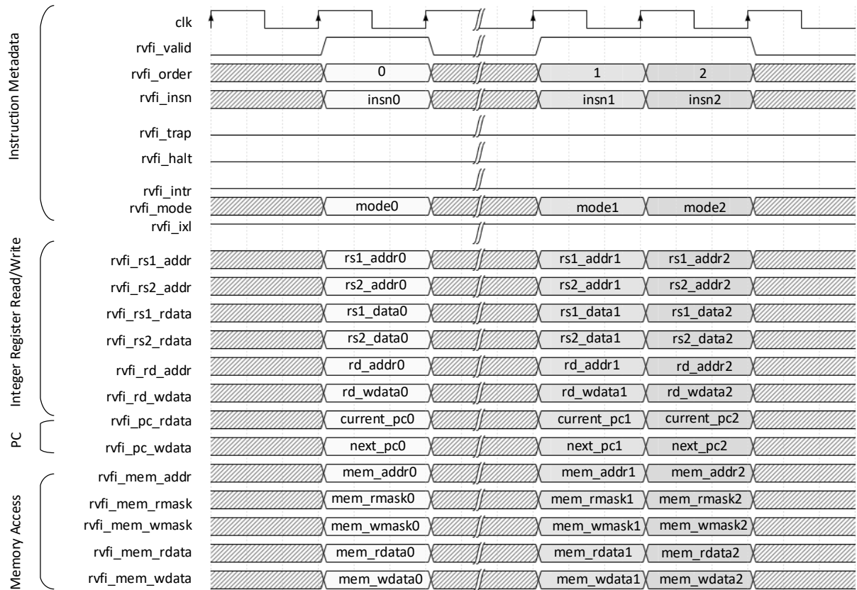
Figure 2.16. RVFI Interface
