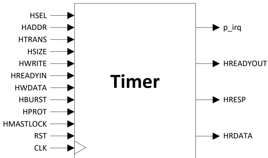
Figure 2.14. Timer Block Diagram
