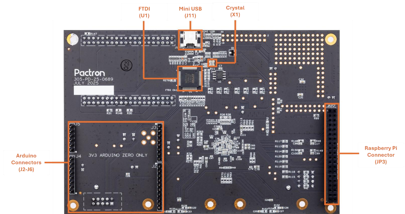
Figure 1.2. Bottom View of MachXO4 Development Board
