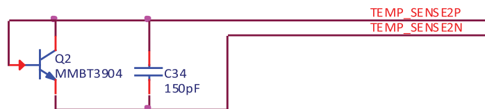
Figure 8.5. NPN Temperature Sensor Circuit
