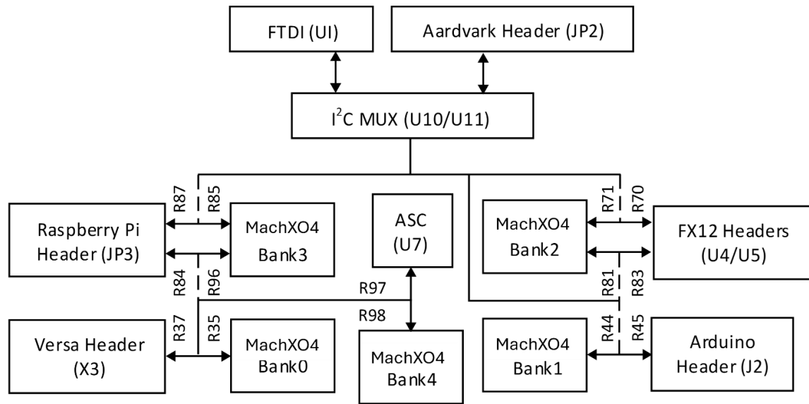
Figure 6.1. I2C Topology
