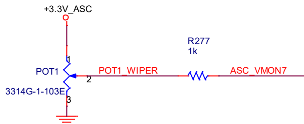
Figure 8.1. POT Circuit Design for VMON7
