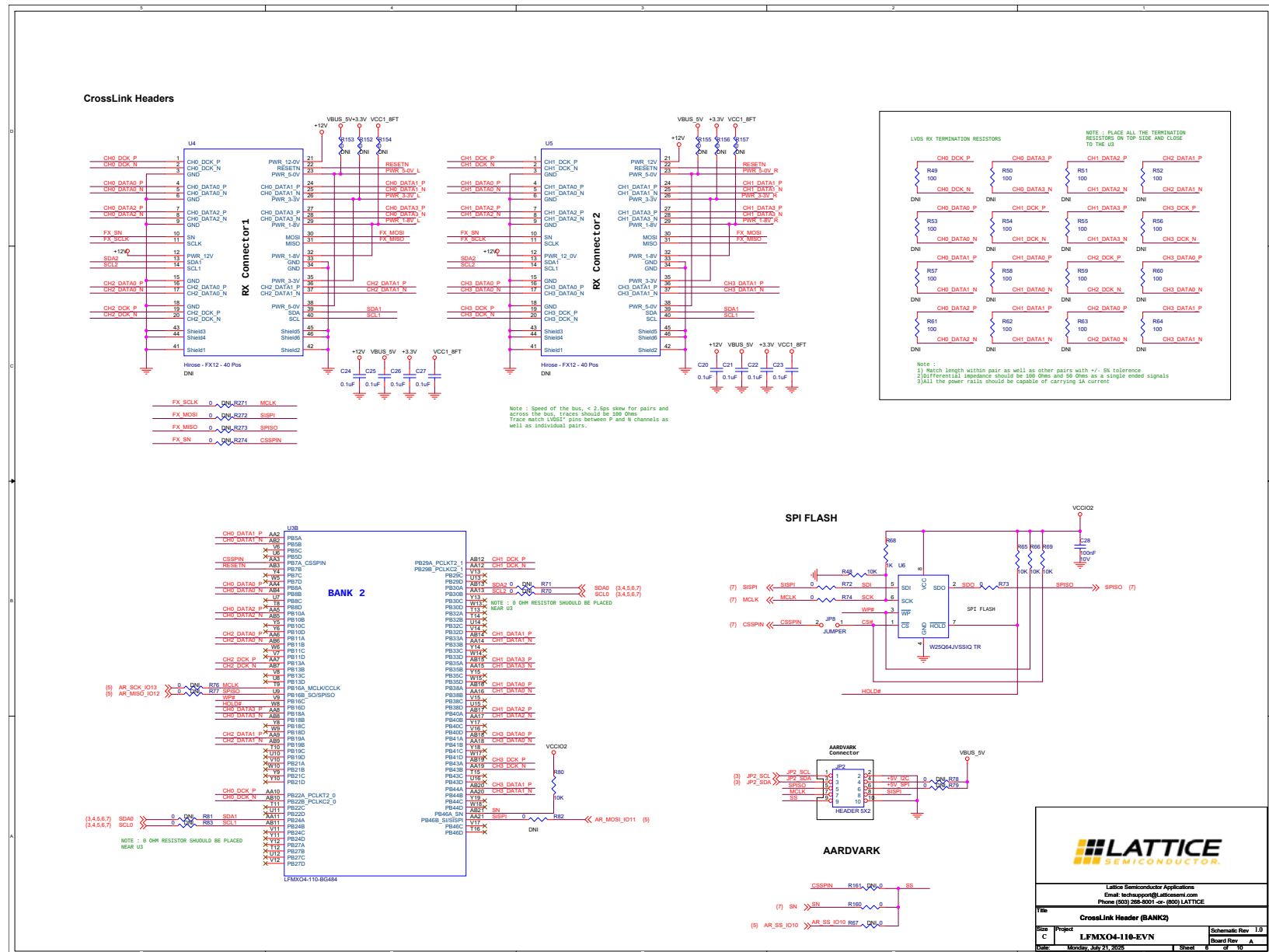
Figure A.6. CrossLink Headers (BANK 2)
