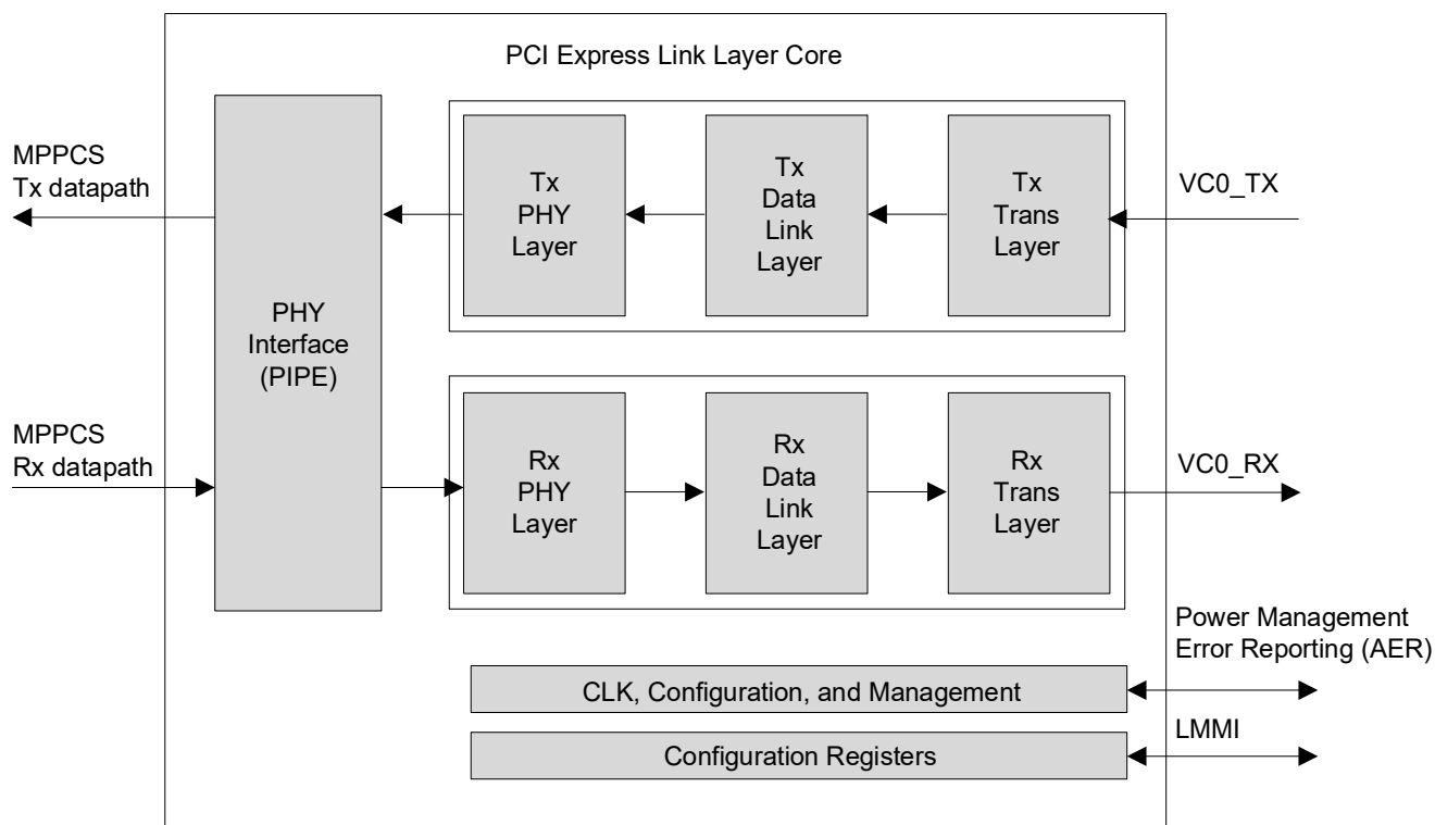
Figure 3.11. PCI Express Link Layer Functional Diagram
