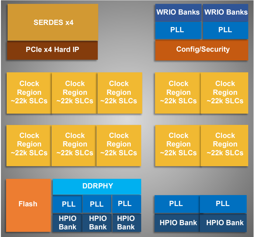
Figure 3.5. High-level Device Floorplan (LN2-MH-20 Device)
