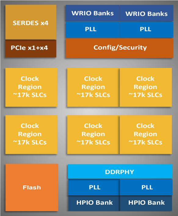
Figure 3.7. High-level Device Floorplan (LN2-MH-10 Device)
