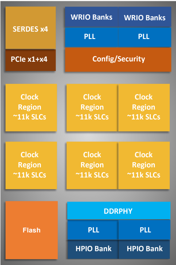
Figure 3.8. High-level Device Floorplan (LN2-MH-06 Device)
