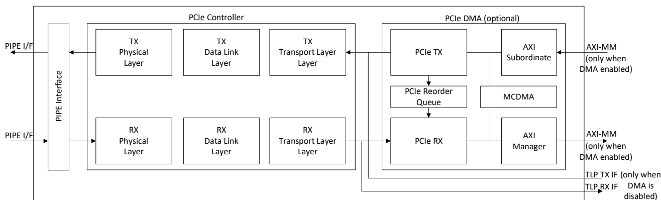
Figure 3.10. PCI Express Hard IP Architecture
