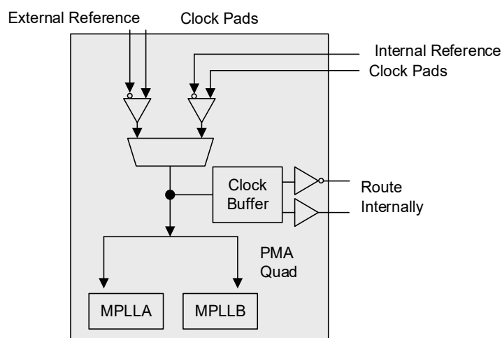
Figure 3.12. Lattice Nexus 2 SERDES Reference Clock Architecture
