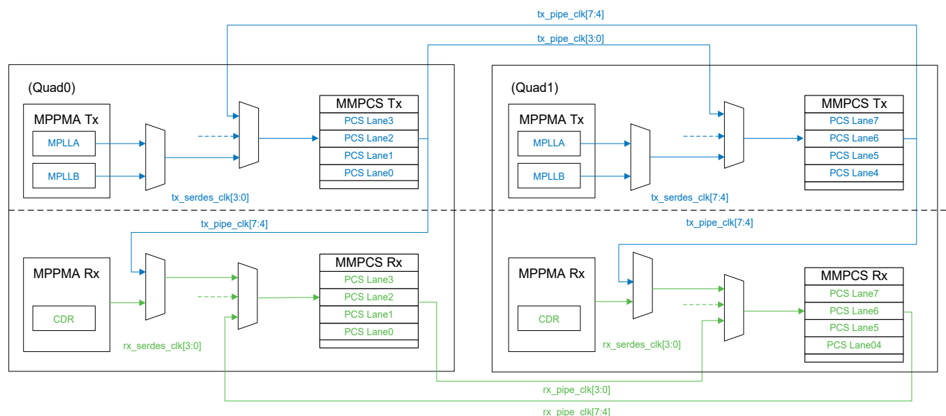
Figure 5.2. Clock Scheme across Two Quads (LN2-CT-16/LN2-CT-20 and LN2-MH-16/LN2-MH-20 Devices)
