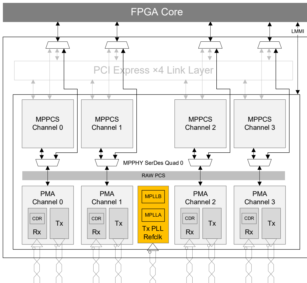
Figure 3.15. MPPCS Bypass Mode
