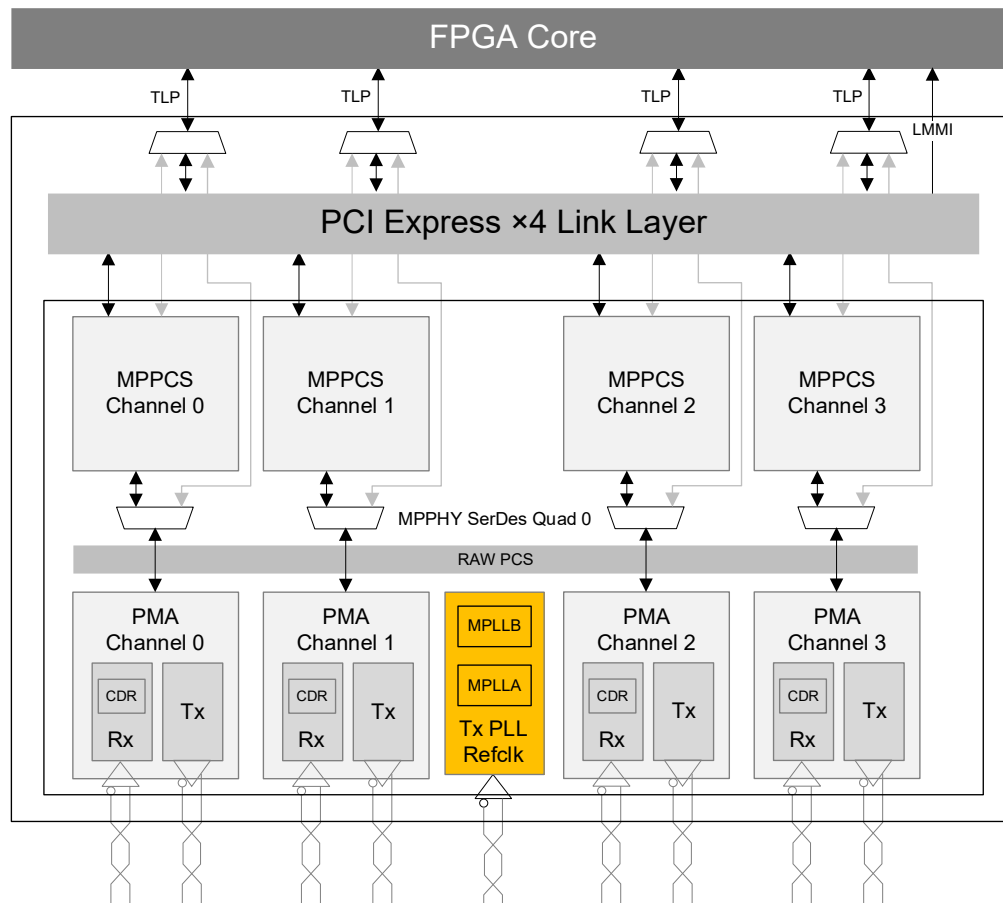
Figure 3.13. PCI Express Hard IP Mode
