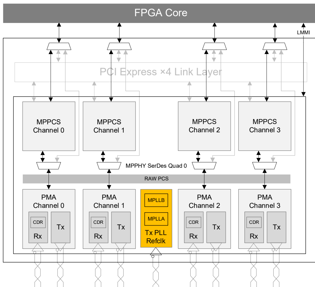
Figure 3.14. Other Modes using MPPCS bypassing PCI Express x4 Link Layer
