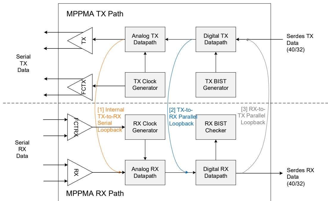
Figure 7.2. MPPMA Loopback
