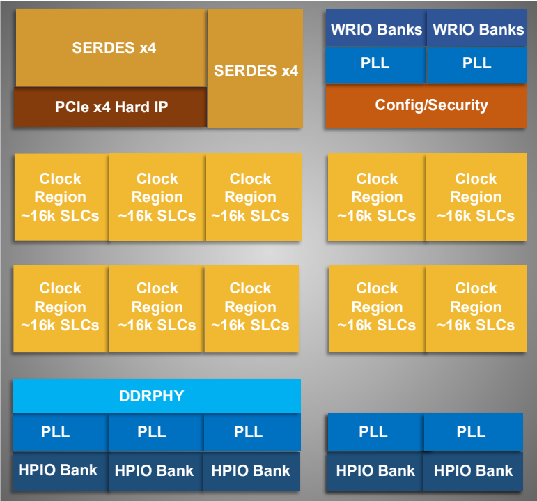
Figure 3.2. High-level Device Floorplan (LN2-CT-16 Device)
