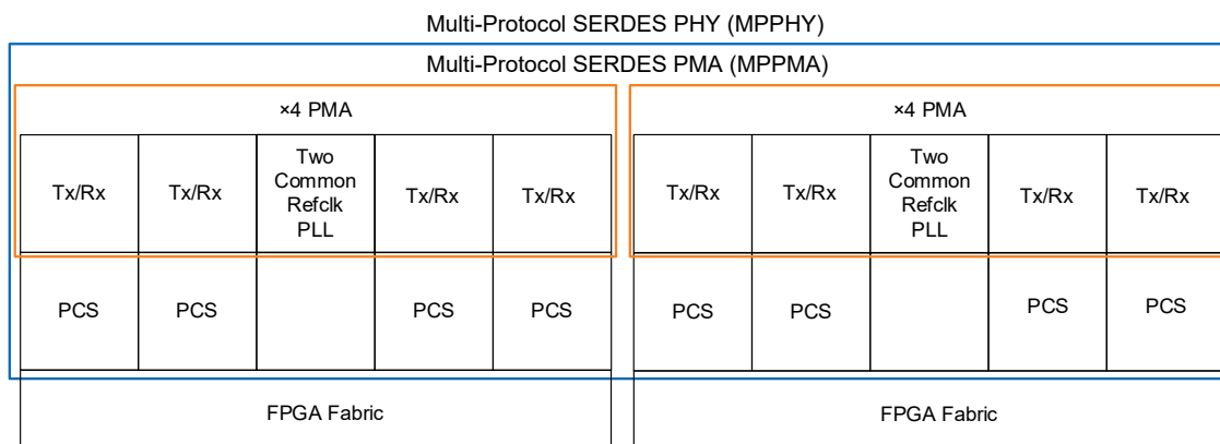
Figure 3.9. Lattice Nexus 2 SERDES Quad Architecture
