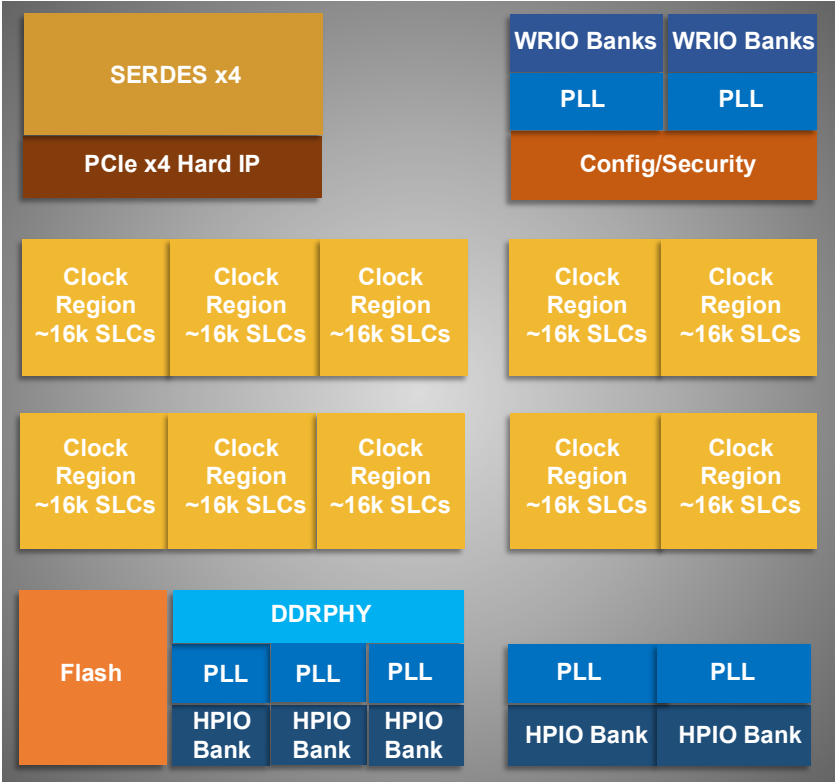
Figure 3.6. High-level Device Floorplan (LN2-MH-16 Device)
