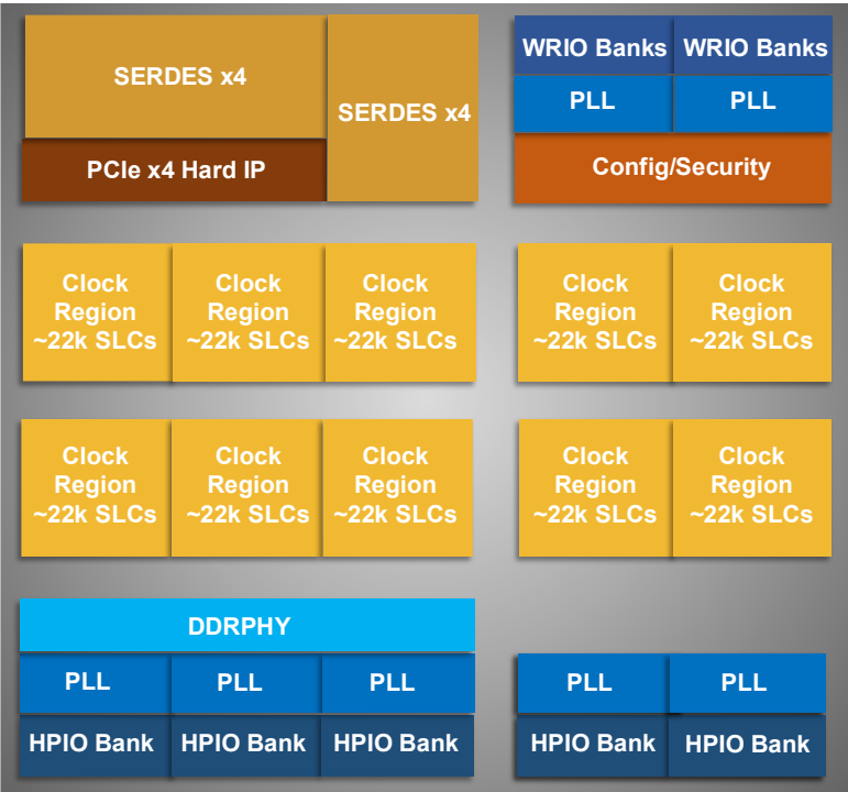
Figure 3.1. High-level Device Floorplan (LN2-CT-20 Device)
