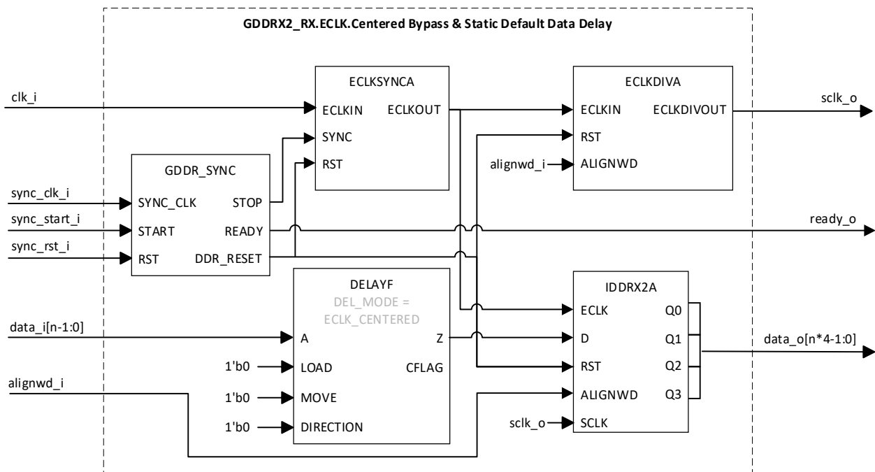
Figure 3.9. GDDR2_RX.ECLK.Centered (Bypass and Static Default Data Delay)
