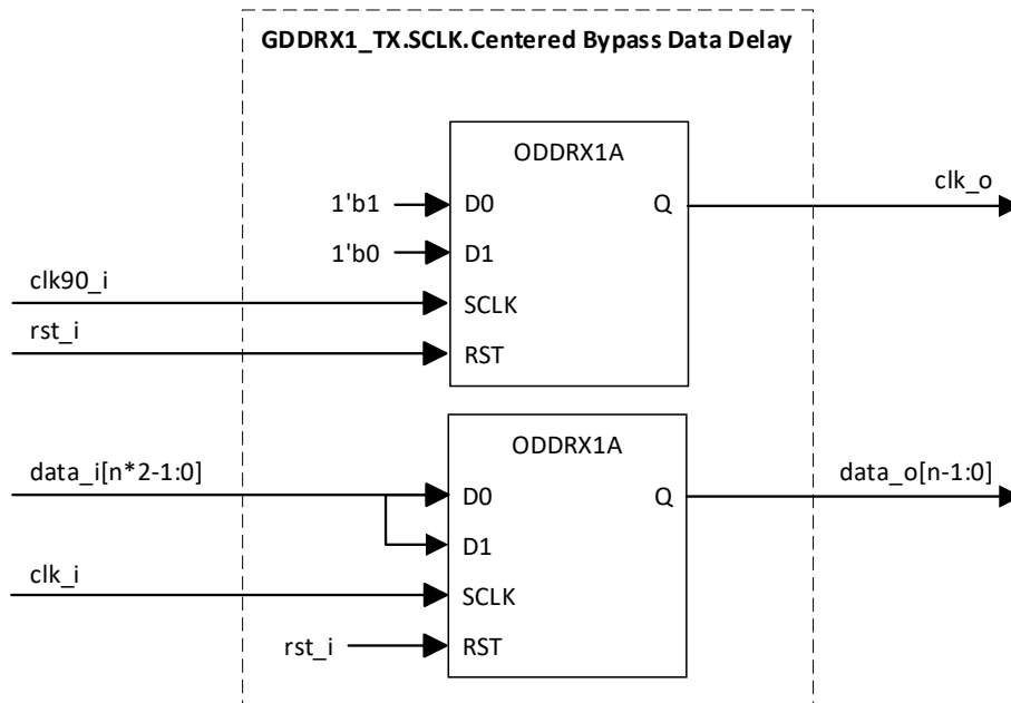
Figure 3.28. GDDR1_TX.SCLK.Centered (Bypass Data Delay)
