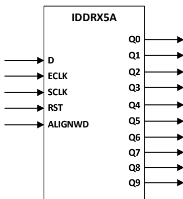
Figure 5.11. IDDRX5A Ports
