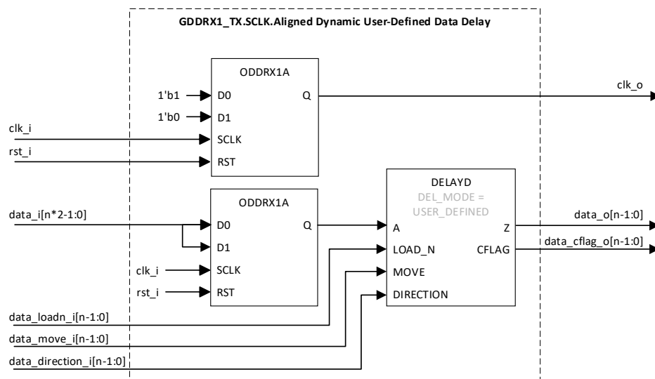
Figure 3.33. GDDR1_TX.SCLK.Aligned (Dynamic User-Defined Data Delay)
