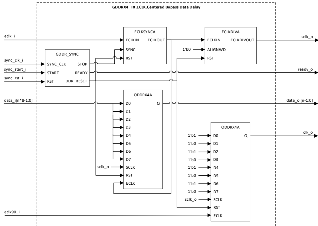
Figure 3.35. GDDR4_TX.ECLK.Centered (Bypass Data Delay)
