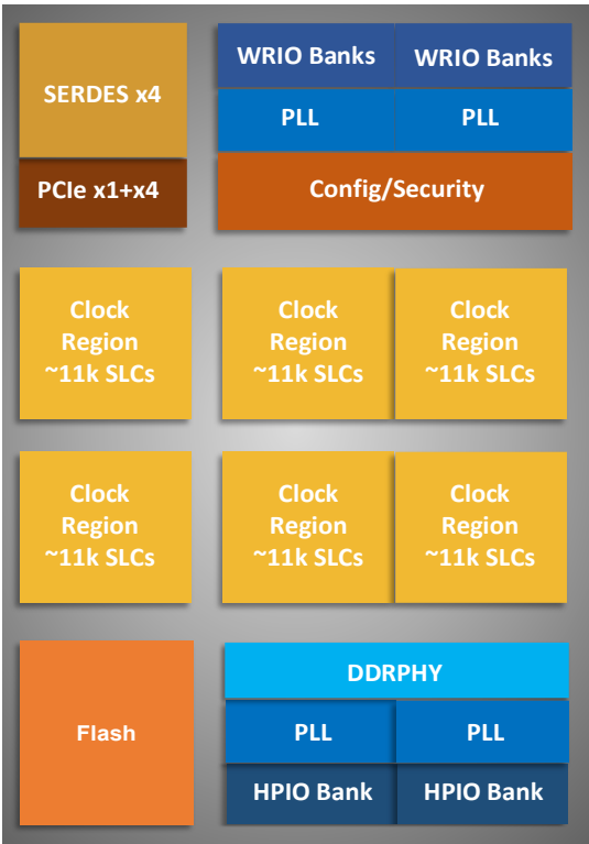
Figure 2.8. High-level Device Floorplan (LN2-MH06 Device)
