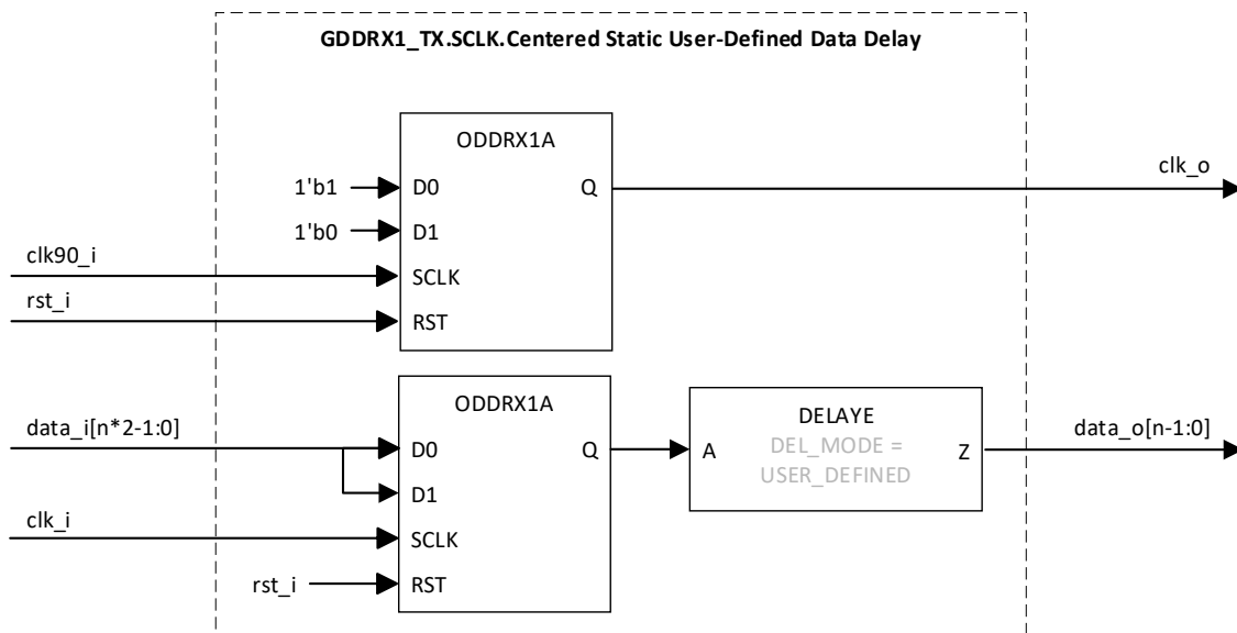
Figure 3.29. GDDR1_TX.SCLK.Centered (Static User-Defined Data Delay)
