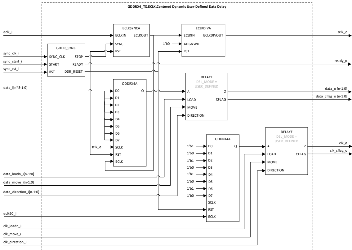
Figure 3.41. GDDR4_TX.ECLK.Centered (Dynamic User-Defined Data Delay)
