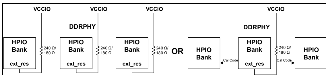
Figure 4.10. External Reference Resistor for LVSTL_I/LVSTL_II (LPDDR4)
