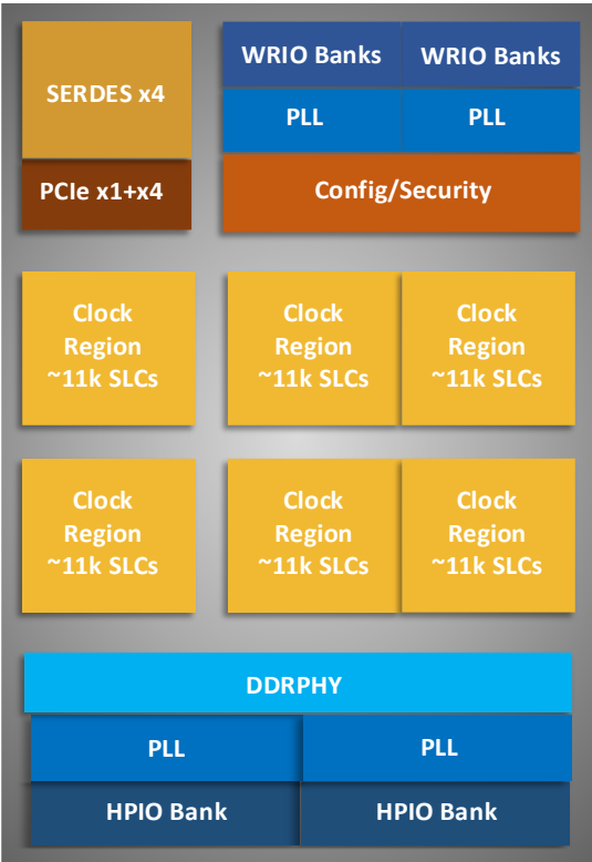
Figure 2.7. High-level Device Floorplan (LN2-CT06 Device)
