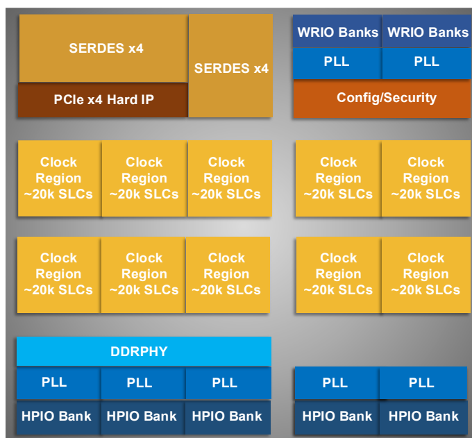
Figure 2.1. High-level Device Floorplan (LN2-CT20 Device)
