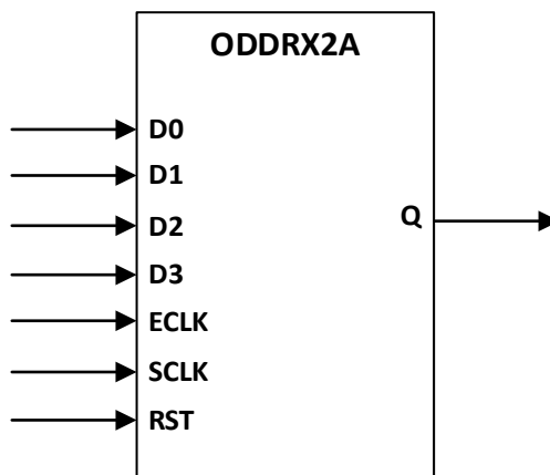
Figure 5.15. ODDRX2A Ports
