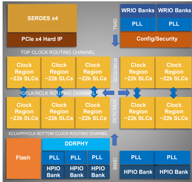
Figure 2.10. High-Level View of Clock Networks (LN2-MH20 Device)
