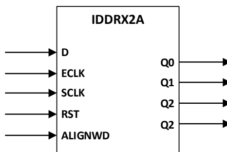
Figure 5.9. IDDRX2A Ports
