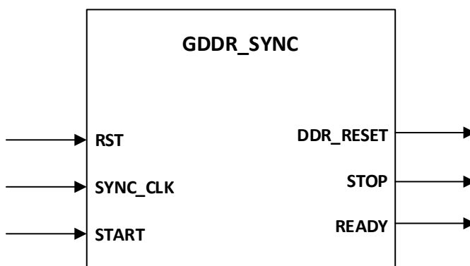
Figure 6.2. GDDR_SYNC Ports
