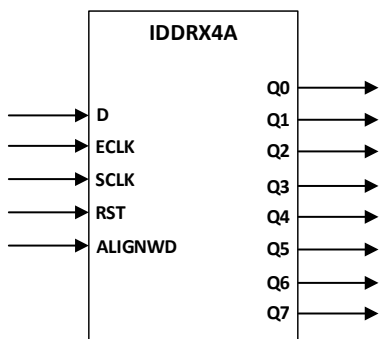
Figure 5.10. IDDRX4A Ports
