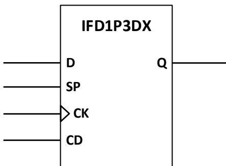
Figure 5.7. IFD1P3DX Ports
