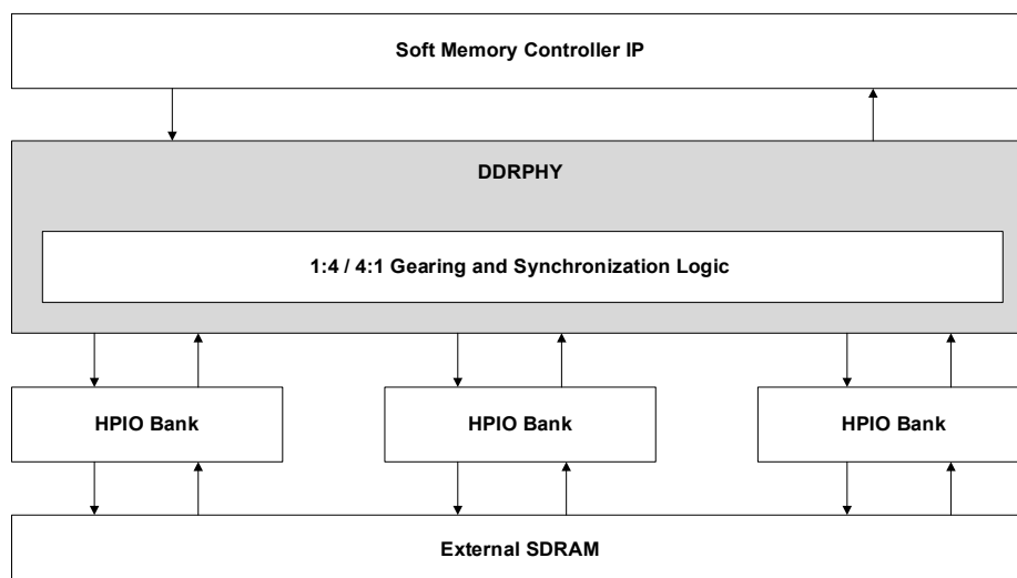
Figure 2.11. Lattice Nexus 2 DDRPHY Block Diagram
