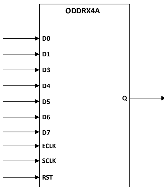
Figure 5.16. ODDRX4A Ports
