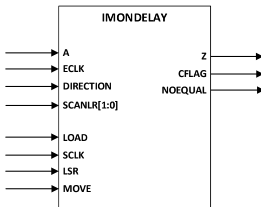
Figure 5.6. IMONDELAY Ports
