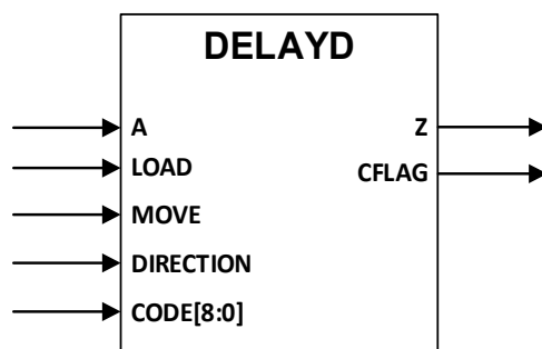
Figure 5.3. DELAYD Ports
