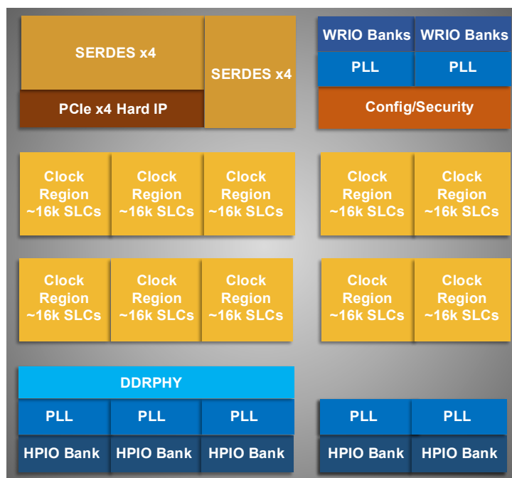
Figure 2.3. High-Level Device Floorplan (LN2-CT16 Device)
