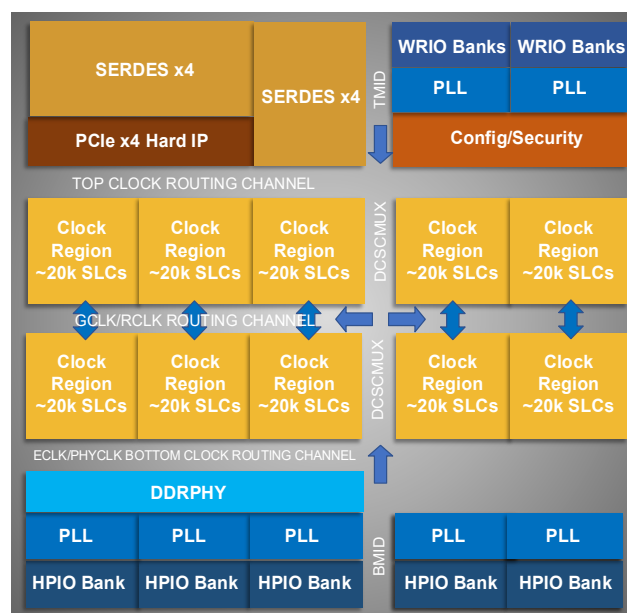
Figure 2.9. High-Level View of Clock Networks (LN2-CT20 Device)
