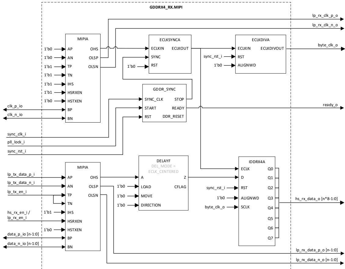
Figure 3.24. GDDR4_RX.MIPI
