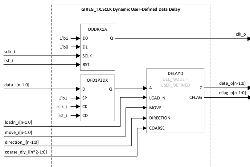
Figure 3.27. GIREG_TX.SCLK (Dynamic User-Defined Data Delay)
