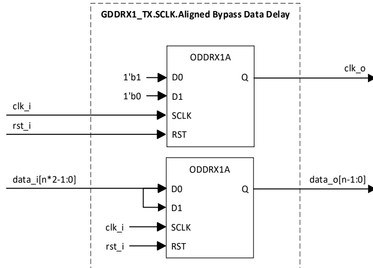
Figure 3.31. GDDR1_TX.SCLK.Aligned (Bypass Data Delay)
