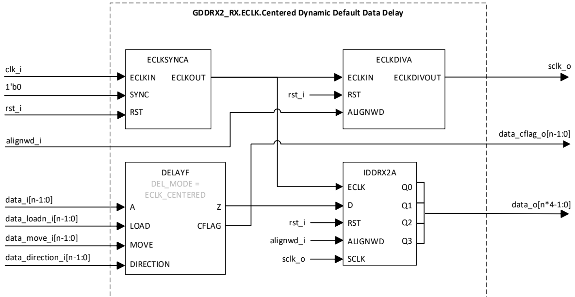
Figure 3.12. GDDR2_RX.ECLK.Centered (Dynamic Default Data Delay)
