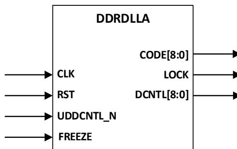
Figure 5.1. DDRDLLA Ports
