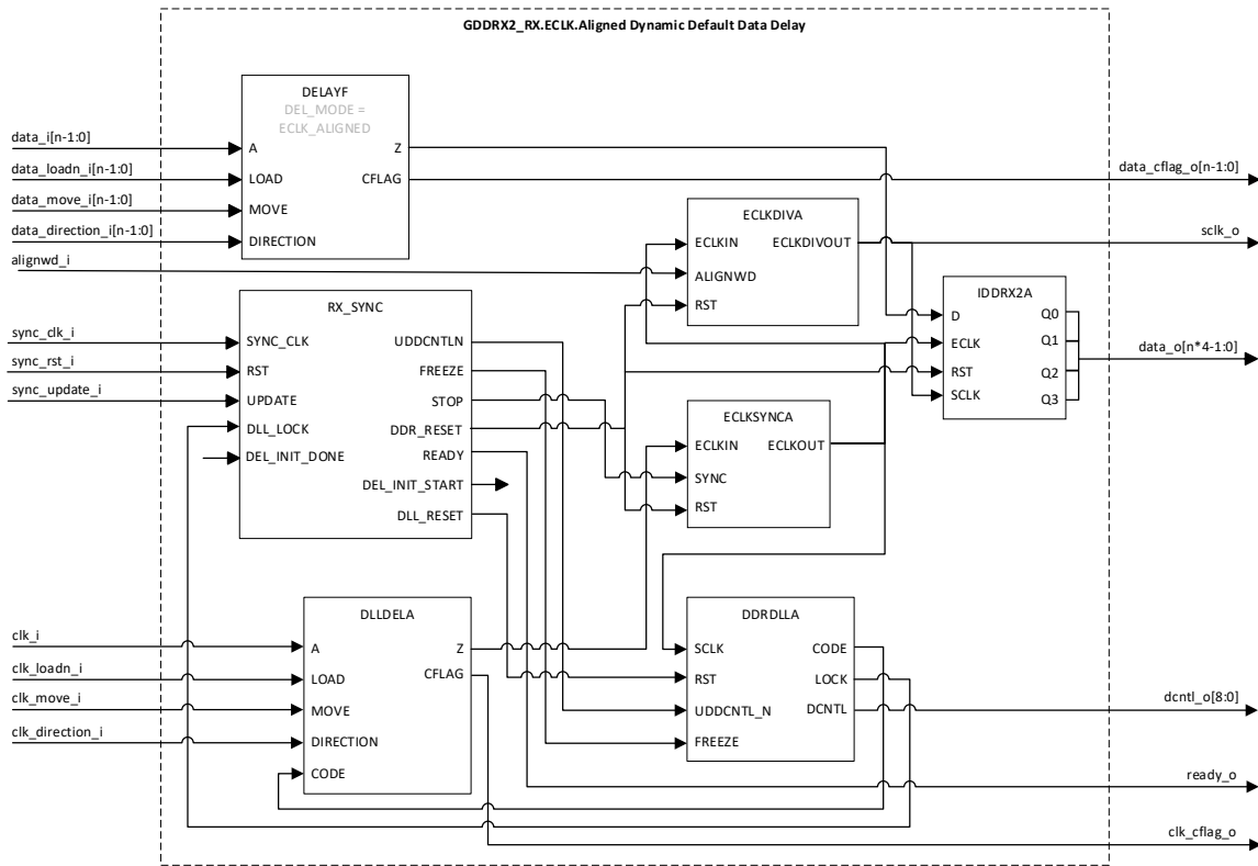
Figure 3.18. GDDR2_RX.ECLK.Aligned (Dynamic Default Data Delay)
