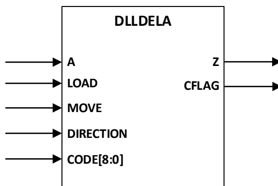
Figure 5.2. DLLDELA Ports
