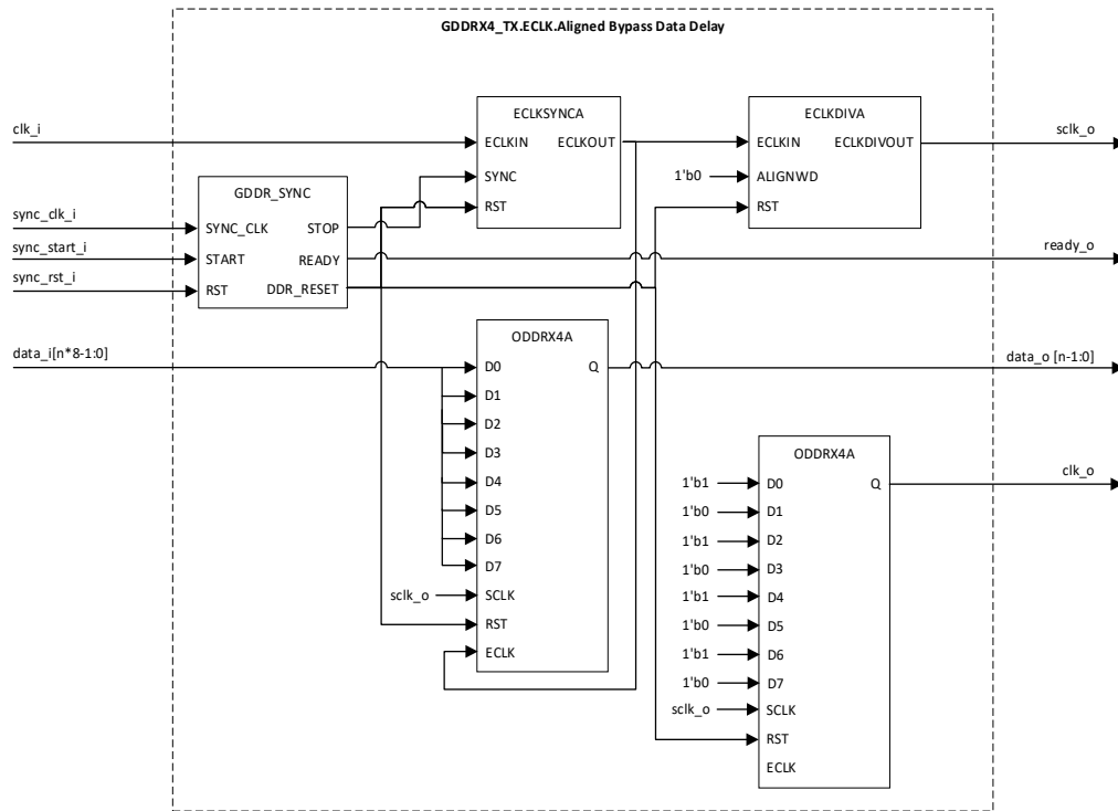
Figure 3.44. GDDR4_TX.ECLK.Aligned (Bypass Data Delay)
