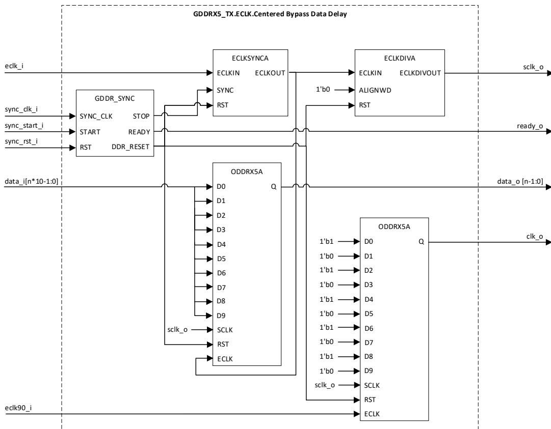
Figure 3.36. GDDR5_TX.ECLK.Centered (Bypass Data Delay)
