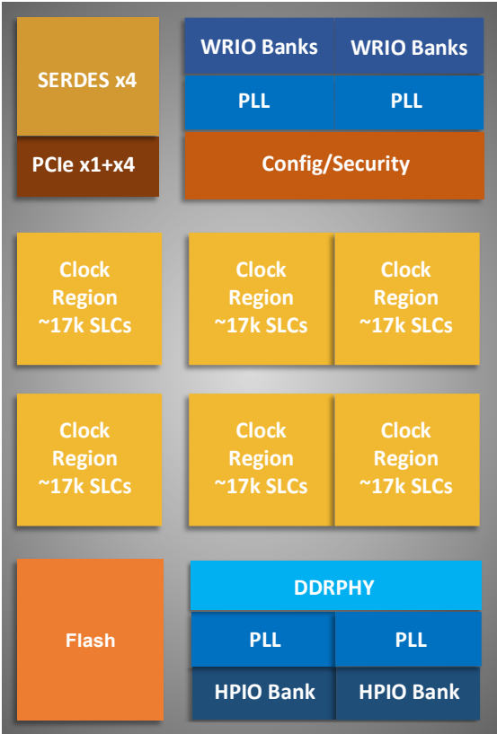
Figure 2.6. High-level Device Floorplan (LN2-MH10 Device)
