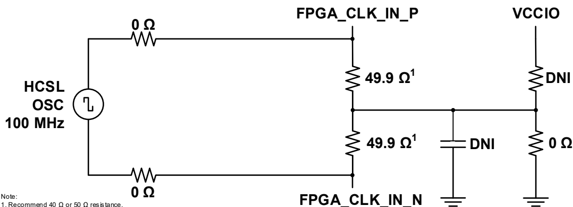
Figure 4.4. HCSL Oscillator on LVDS PCB Footprint
