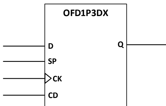
Figure 5.13. OFD1P3DX Ports
