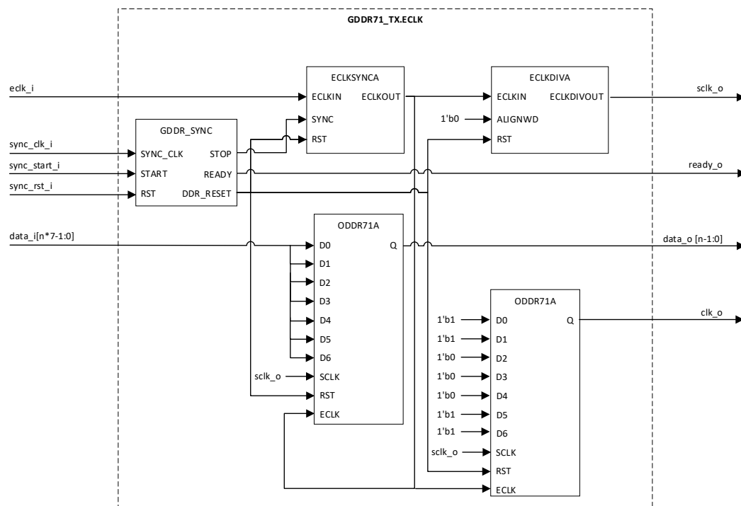
Figure 3.52. GDDR71_TX.ECLK
