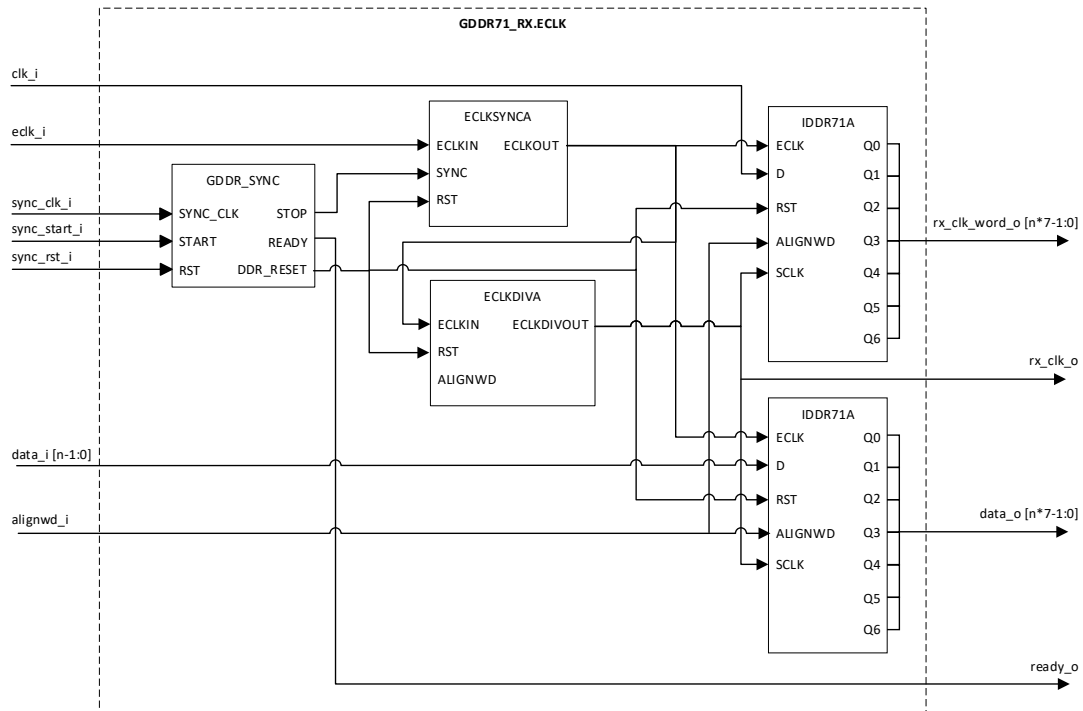
Figure 3.21. GDDR71_RX.ECLK
