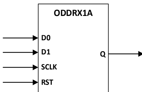
Figure 5.14. ODDRX1A Ports
