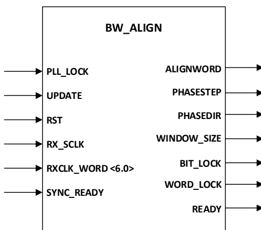
Figure 6.3. BW_ALIGN Ports
