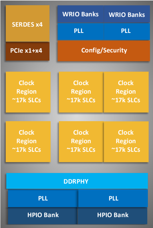
Figure 2.5. High-level Device Floorplan (LN2-CT10 Device)
