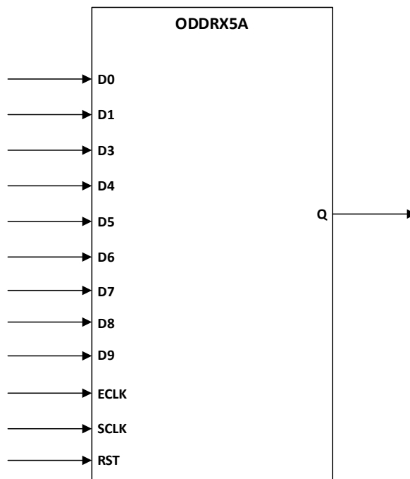
Figure 5.17. ODDR5A Ports
