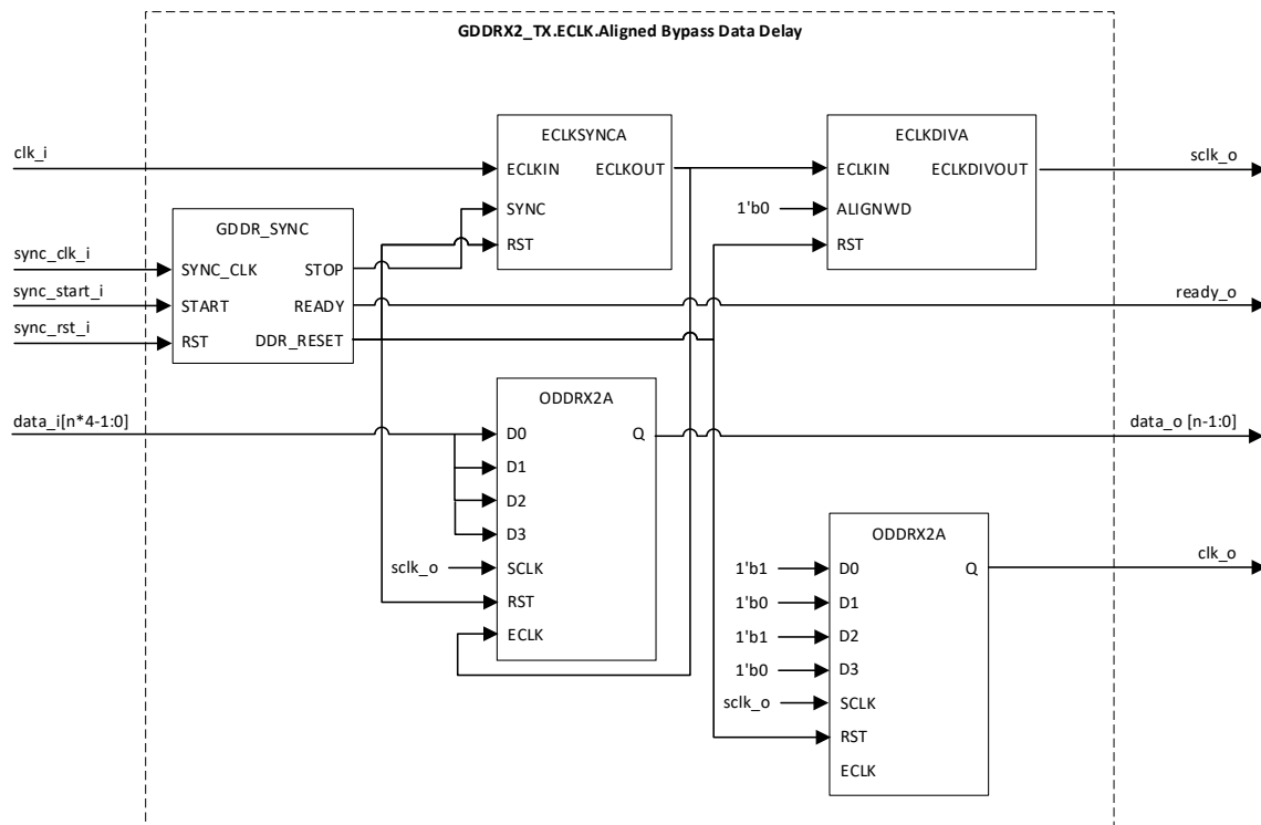
Figure 3.43. GDDR5_TX.ECLK.Aligned (Bypass Data Delay)
