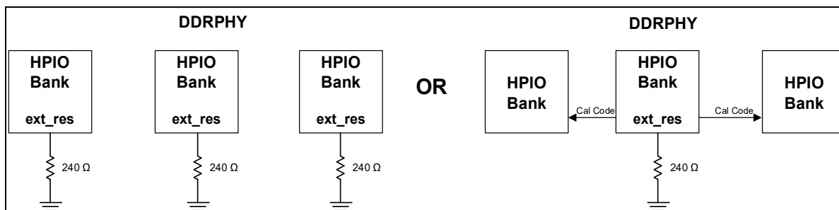
Figure 4.8. External Reference Resistor for POD (DDR4)
