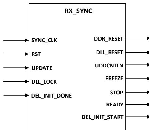
Figure 6.1. RX_SYNC Ports
