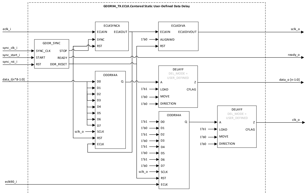
Figure 3.38. GDDR_X4_TX.ECLK.Centered (Static User-Defined Data Delay)
