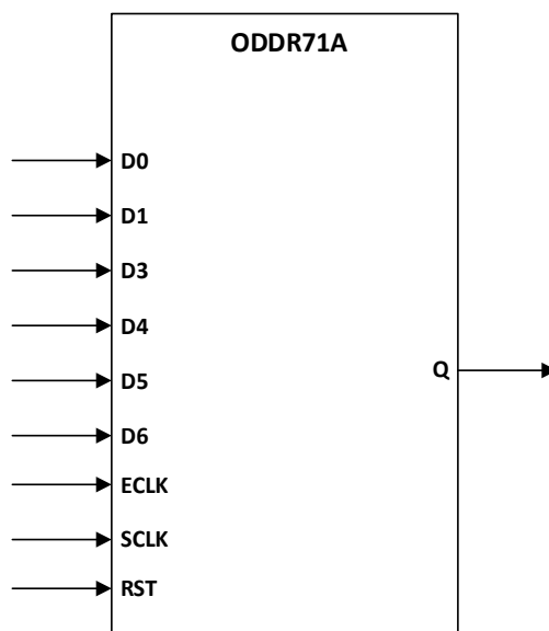
Figure 5.18. ODDR71A Ports
