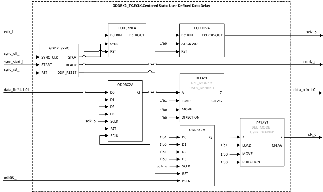
Figure 3.37. GDDR_X2_TX.ECLK.Centered (Static User-Defined Data Delay)
