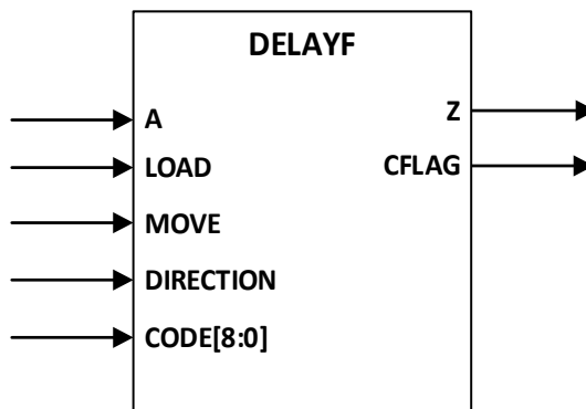
Figure 5.5. DELAYF Ports
