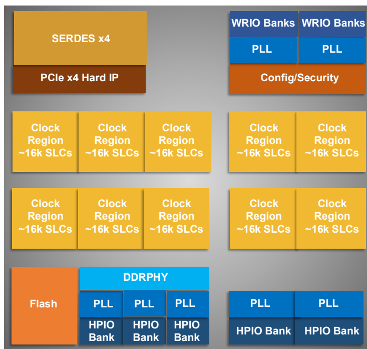
Figure 2.4. High-level Device Floorplan (LN2-MH16 Device)
