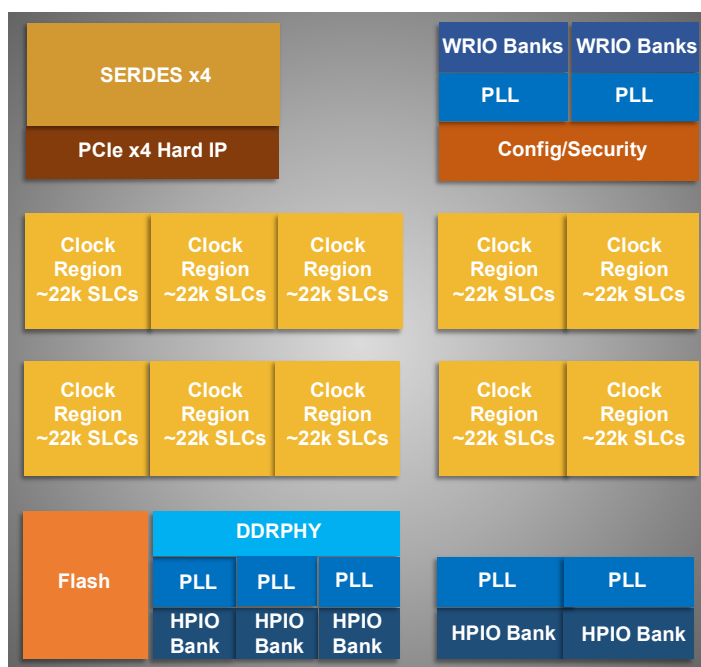
Figure 2.2. High-level Device Floorplan (LN2-MH20/21D Device)
