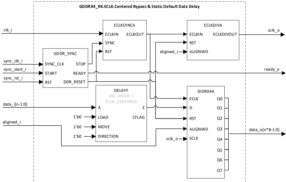
Figure 3.10. GDDR4_RX.ECLK.Centered (Bypass and Static Default Data Delay)
