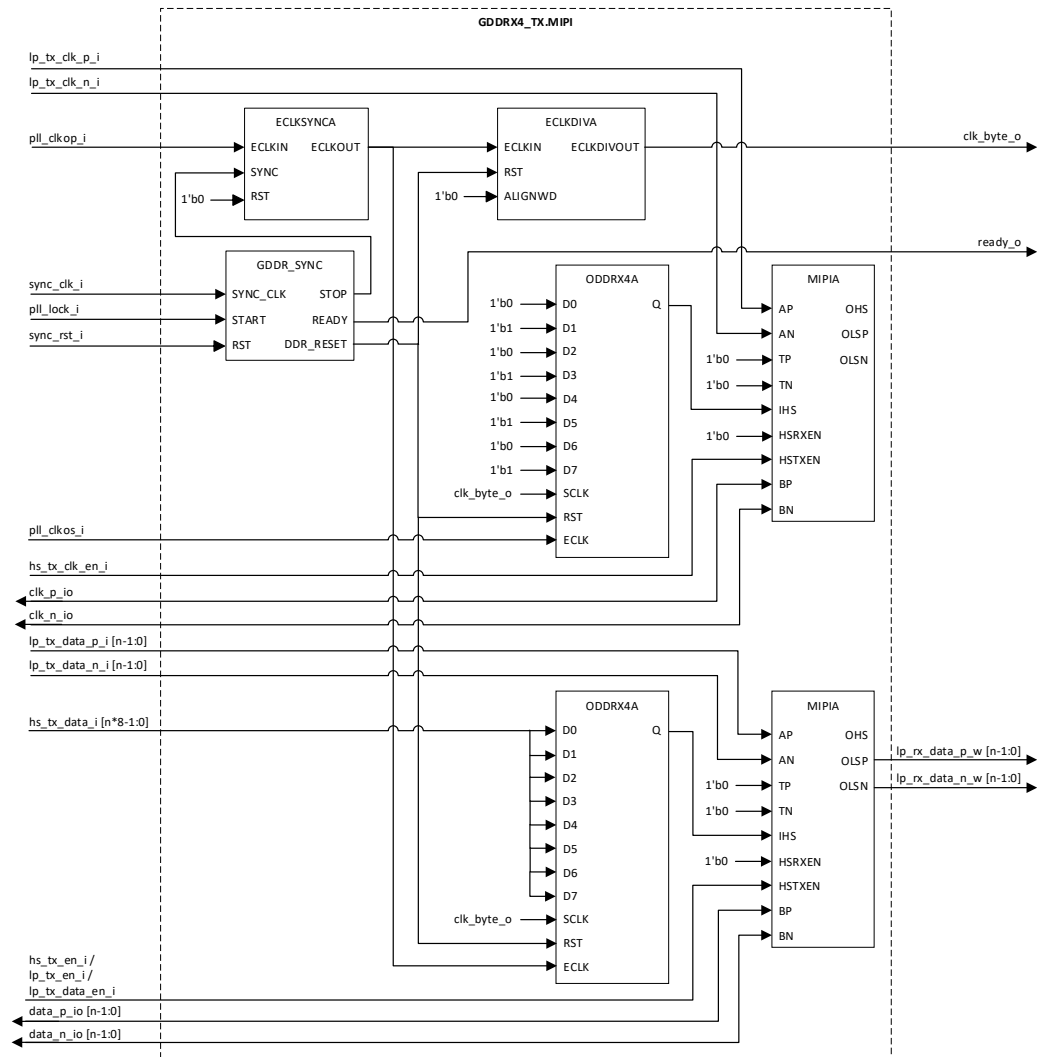
Figure 3.53. GDDR4_TX.MIPI
