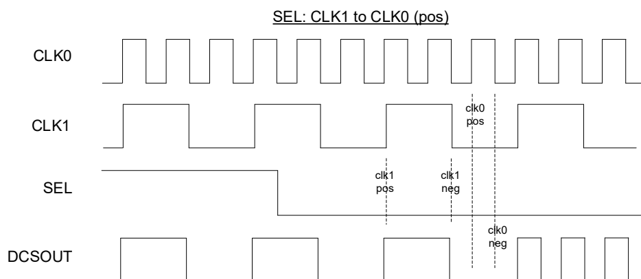
Figure 2.26. Posedge DCS Switch from SEL: 1 ≥ 0
