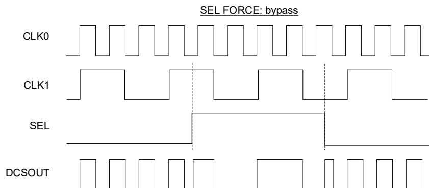
Figure 2.32. MODESEL = 1 DCS Clock Switch
