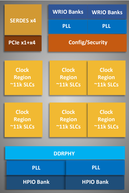
Figure 2.7. Clock Regions (LN2-CT-06 Devices)
