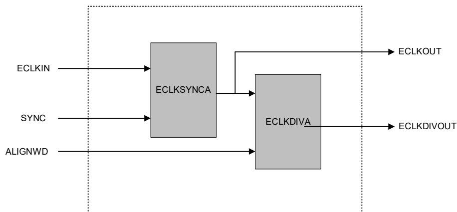
Figure 2.15. ECLKSYNCDIV
