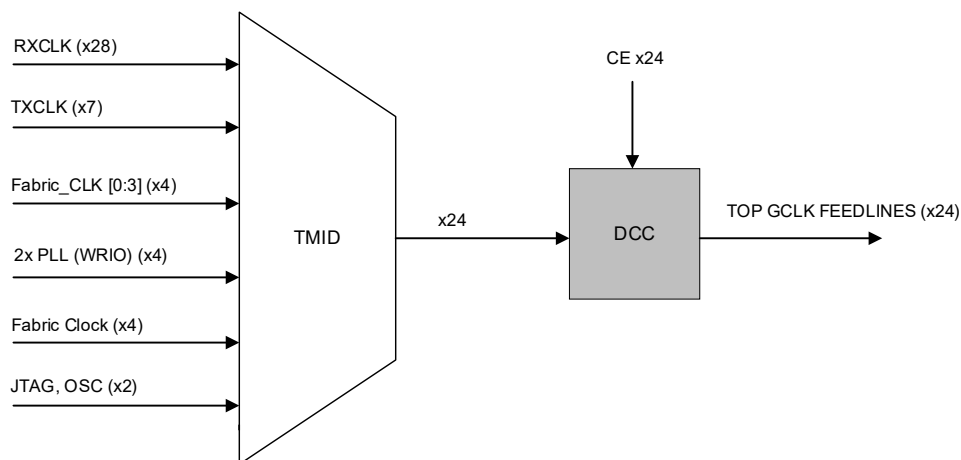
Figure 2.34. TMID Multiplexer, DCC Elements, and Top GCLK Feedlines
