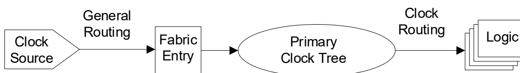
Figure 2.39. Gated Clock to the Primary Clock Routing
