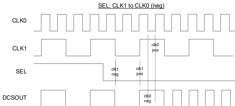
Figure 2.28. Negedge DCS Switch from SEL: 1 ≥ 0
