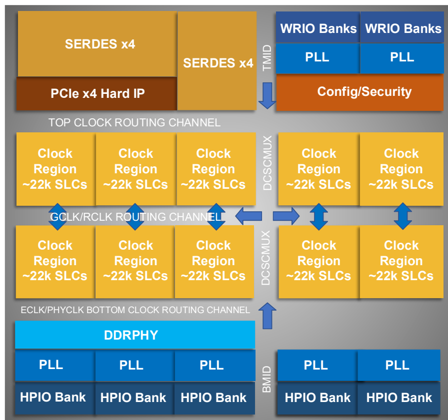
Figure 2.9. High-Level View of Clock Networks and Elements (LN2-CT-20 Devices)
