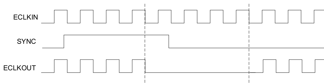
Figure 2.19. ECLKSYNCA Functional Waveform
