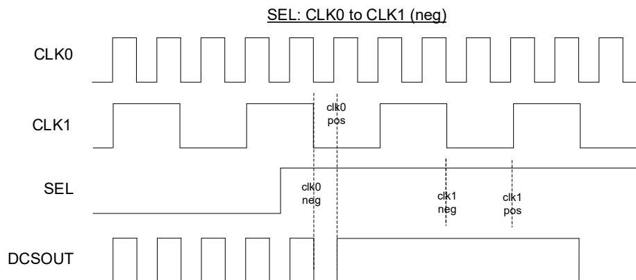
Figure 2.27. Negedge DCS Switch from SEL: 0 ≥ 1
