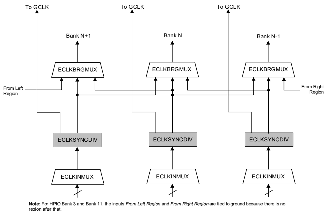
Figure 2.16. Edge Clock Sources Bridged to Multiple Banks
