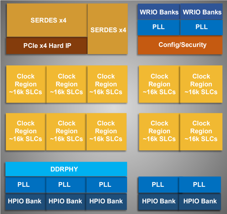
Figure 2.3. Clock Regions (LN2-CT-16 Devices)
