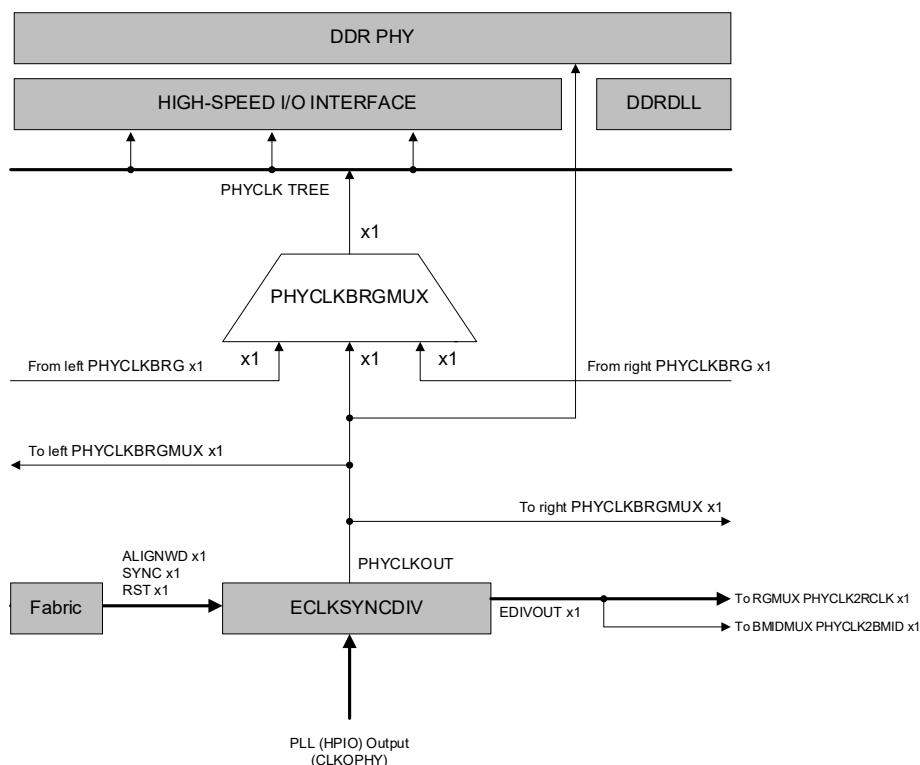
Figure 2.17. PHYCLK Network
