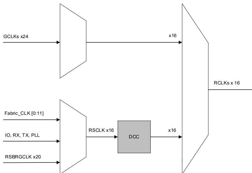
Figure 2.13. Generic RGMUX Implementation
