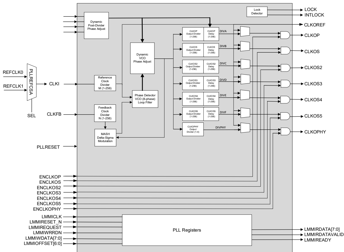
Figure 3.1. Lattice Nexus 2 PLL Block Diagram
