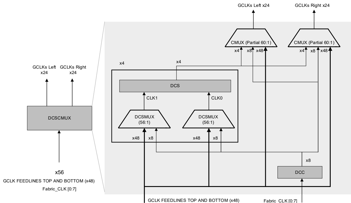
Figure 2.24. DCSCMUX
