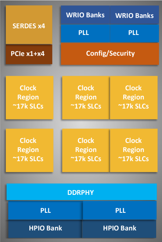
Figure 2.5. Clock Regions (LN2-CT-10 Devices)
