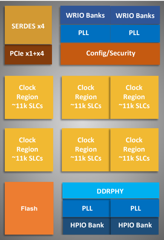
Figure 2.8. Clock Regions (LN2-MH-06 Devices)
