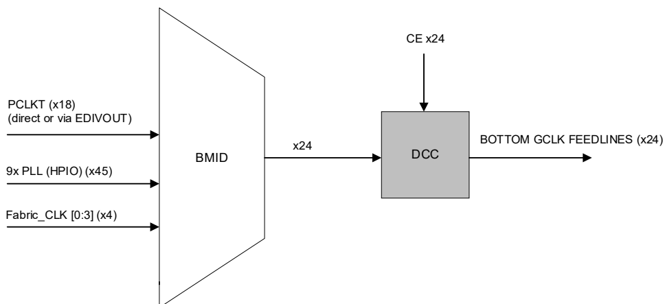
Figure 2.35. BMID Multiplexer, DCC Elements, and Bottom GCLK Feedlines
