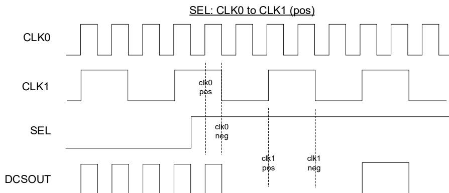
Figure 2.25. Posedge DCS Switch from SEL: 0 ≥ 1
