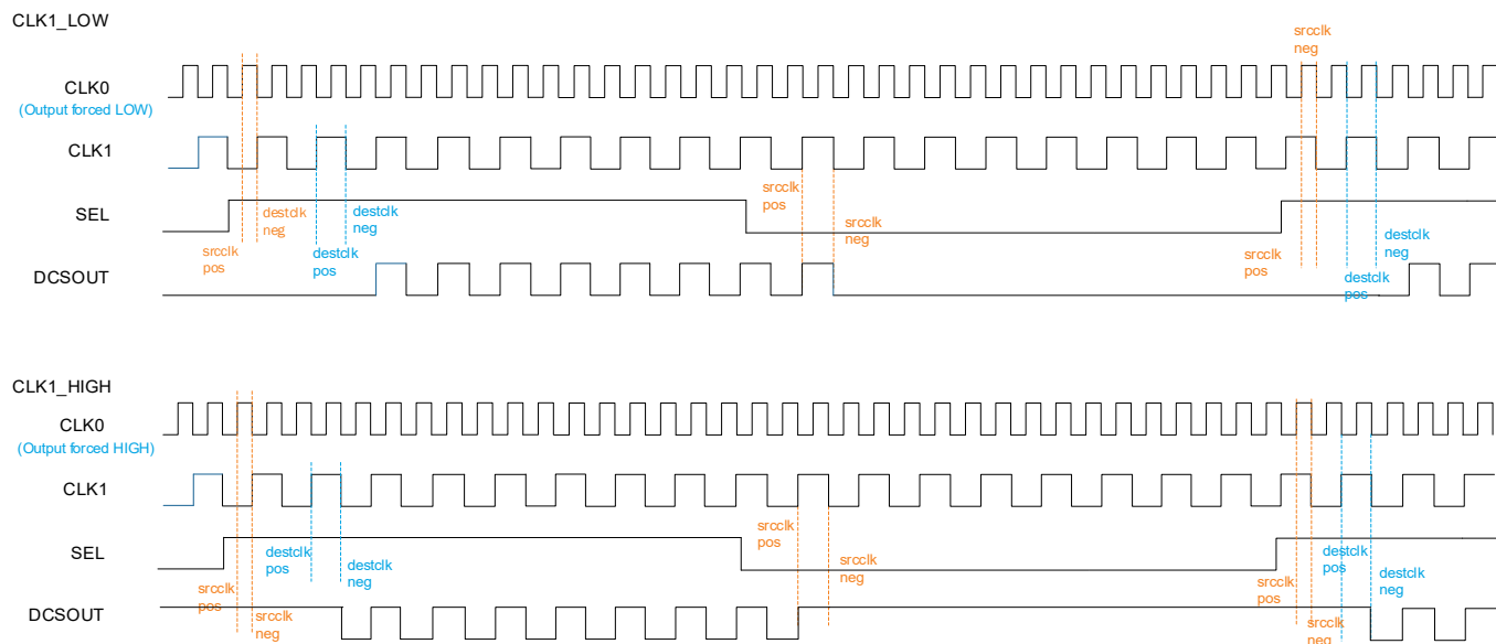
Figure 2.31. DCSMODE = CLK1_LOW or CLK1_HIGH
