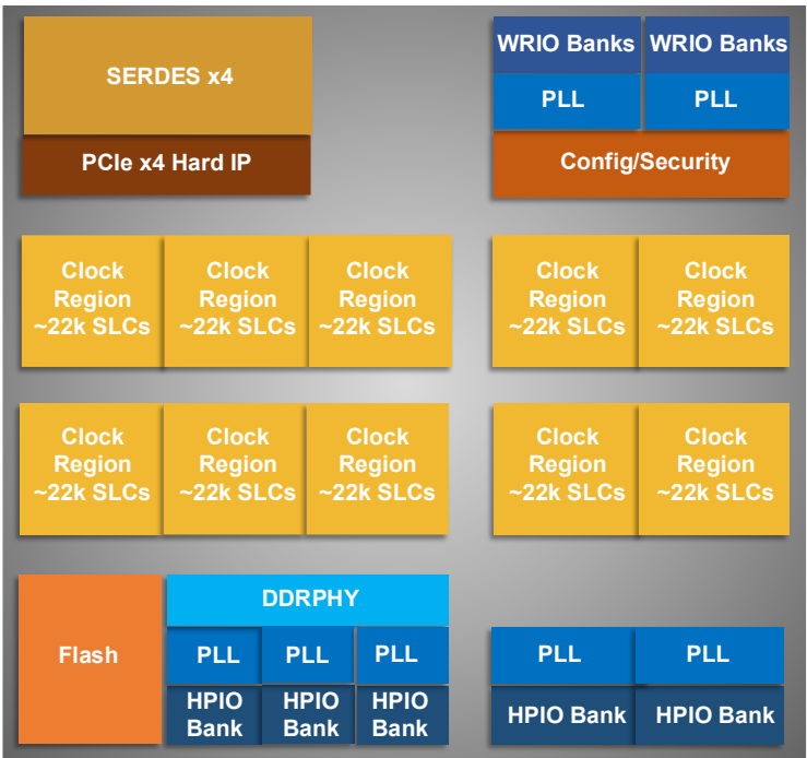
Figure 2.2. Clock Regions (LN2-MH-20 Devices)
