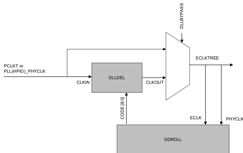
Figure 2.21. High-Level Implementation of DLLDEL and Code Control in HPIO Bank
