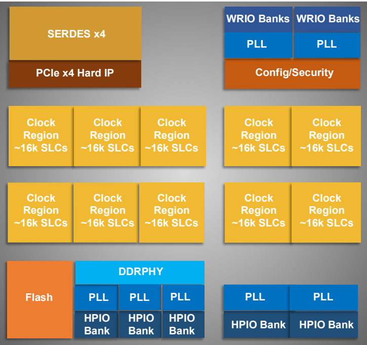
Figure 2.4. Clock Regions (LN2-MH-16 Devices)
