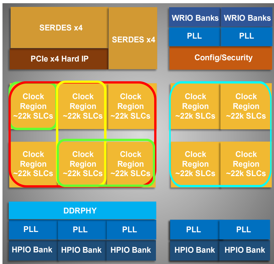
Figure 2.12. Multi-Region Clock Formations (LN2-CT-20 Devices)
