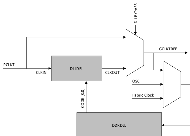
Figure 2.22. High-Level Implementation of DLLDEL and Code Control in WRIO Bank
