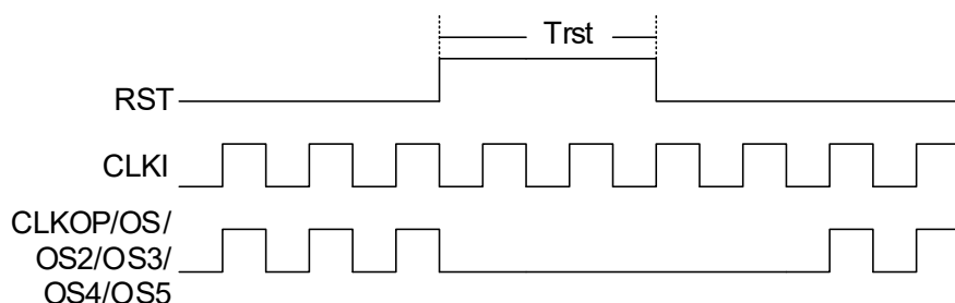
Figure 3.4. RST Input Timing Diagram
