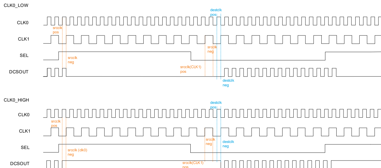
Figure 2.30. DCSMODE = CLK0_LOW or CLK0_HIGH
