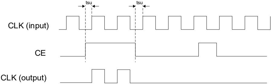
Figure 2.36. Glitchless DCC Functional Waveform
