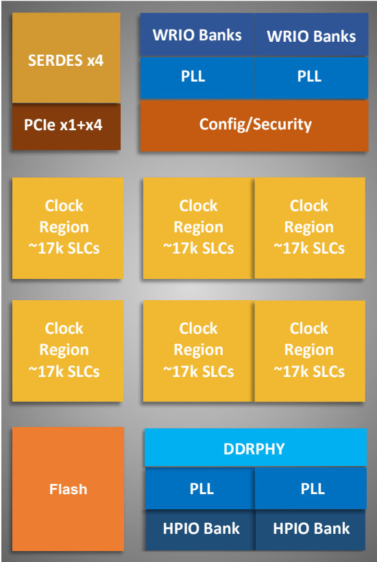
Figure 2.6. Clock Regions (LN2-MH-10 Devices)
