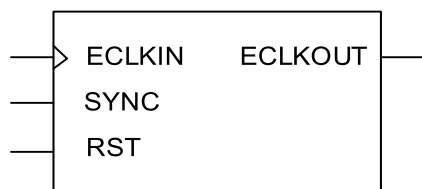
Figure 2.18. ECLKSYNCA Component Symbol
