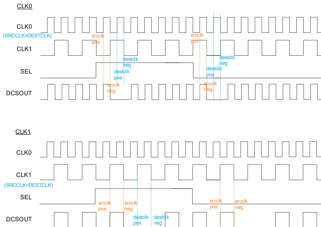
Figure 2.29. DCSMODE = CLK0 or CLK1
