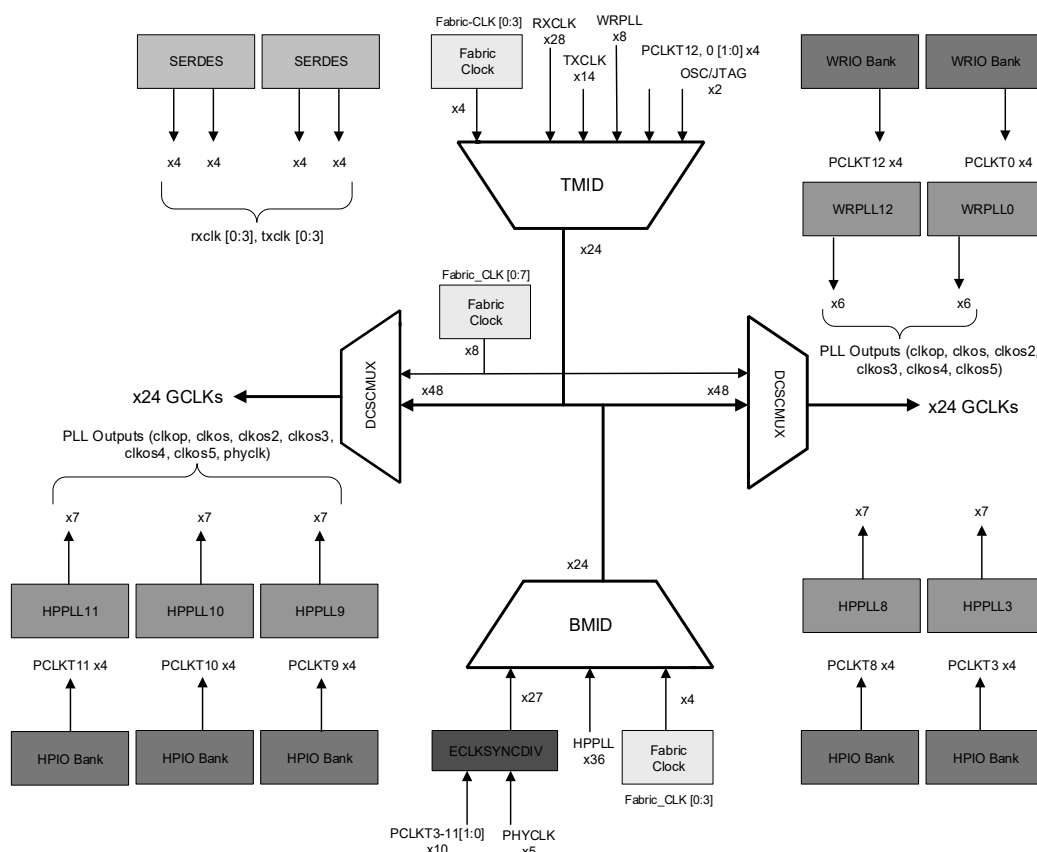
Figure 2.10. Global Clock Routing Architecture for LN2-CT-20 Devices
