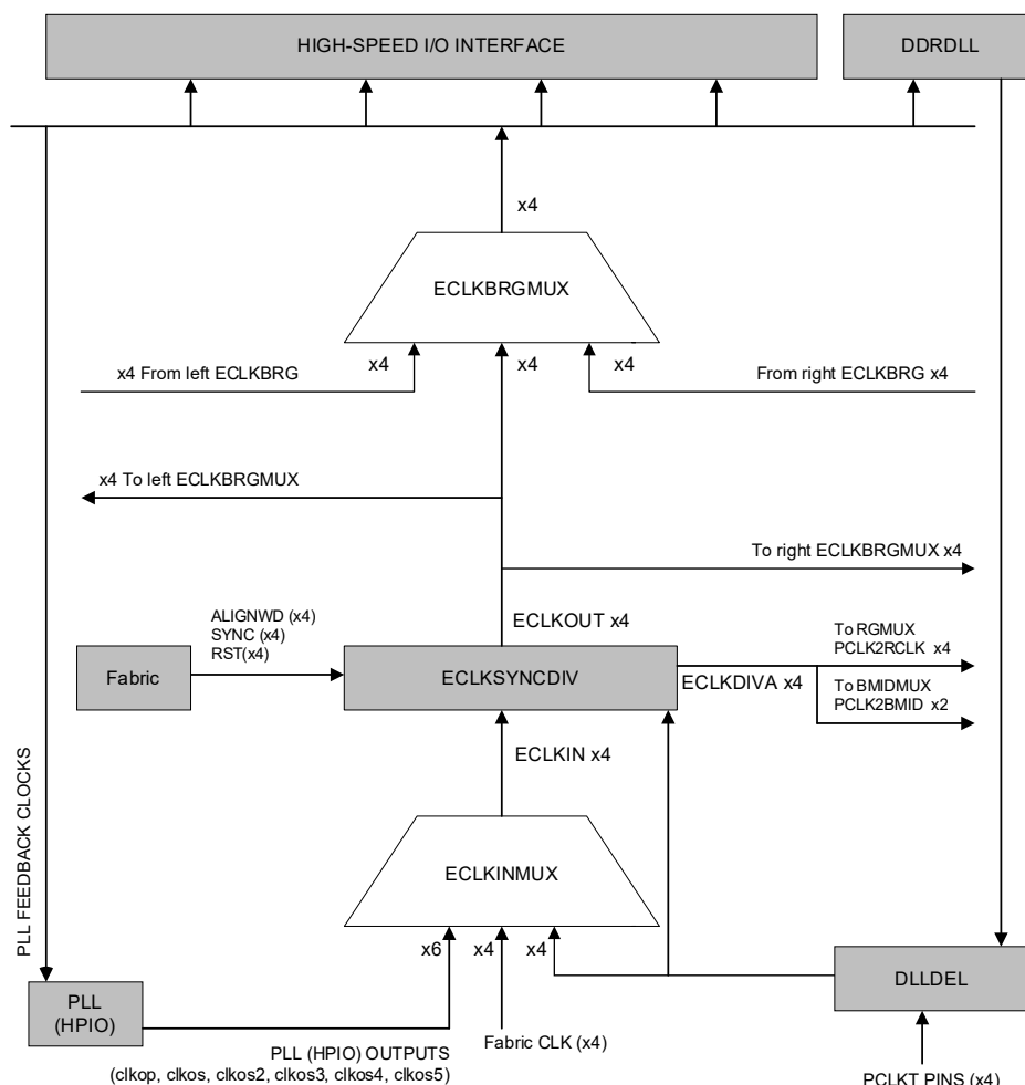
Figure 2.14. Edge Clock Sources per Bank
