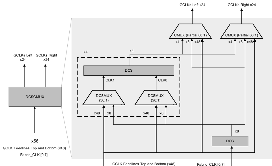
Figure 2.11. DCSCMUX
