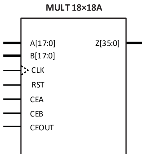
Figure 3.5. MULT18×18A Primitive
