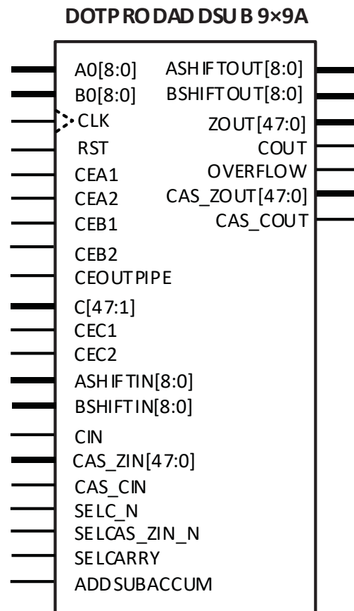
Figure 3.12. DOTPRODADDSUB9×9A Primitive
