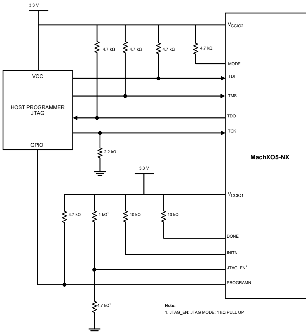
Figure 6.1. Typical Connections for Device Provisioning via JTAG for LFMXO5-15D, LFMXO5-20TD/Q, and LFMXO5-30TD/Q
