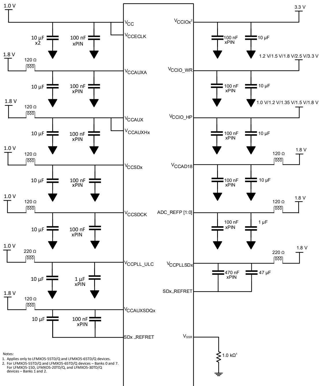
Figure 3.1. Recommended Power Filter
