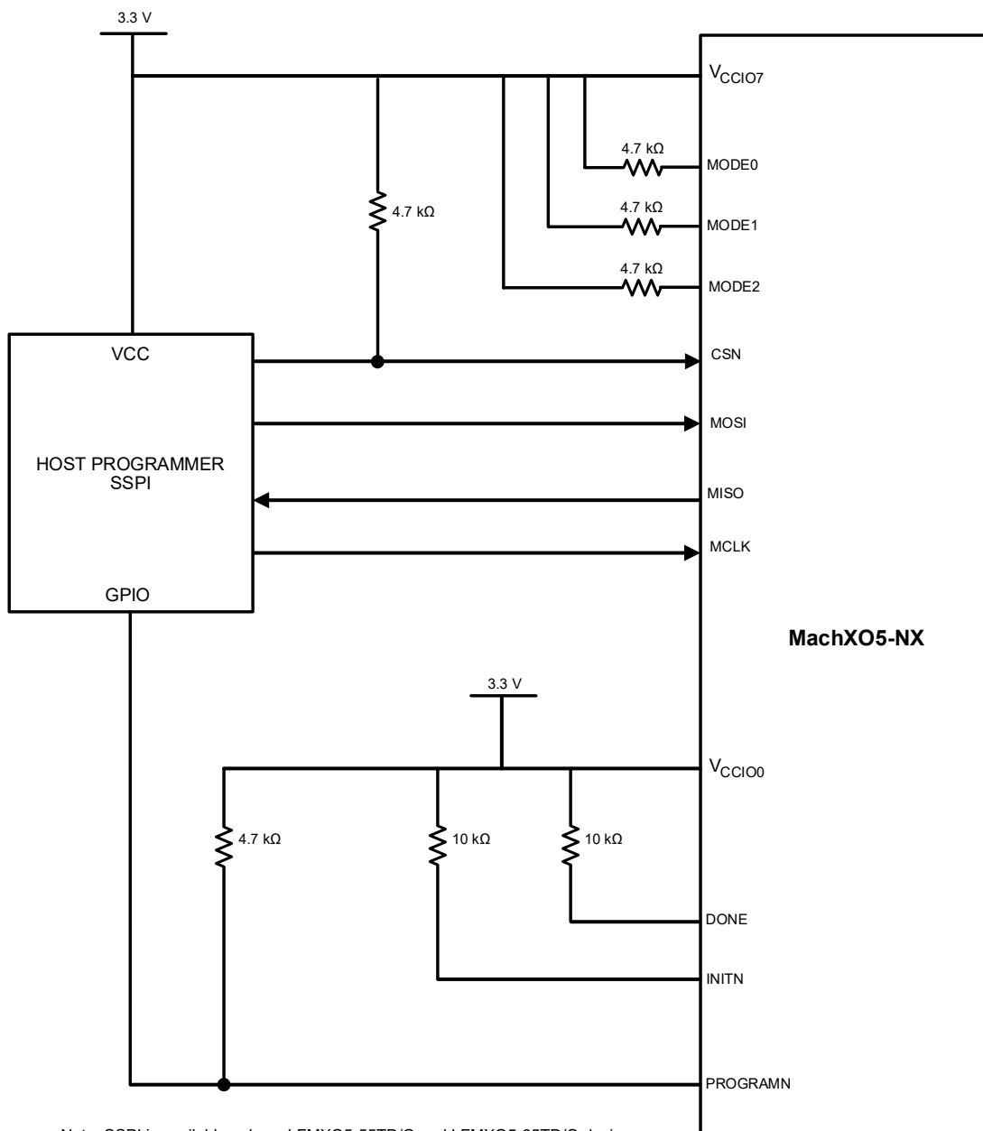
Figure 6.3. Typical Connections for Device Provisioning via SSPI
