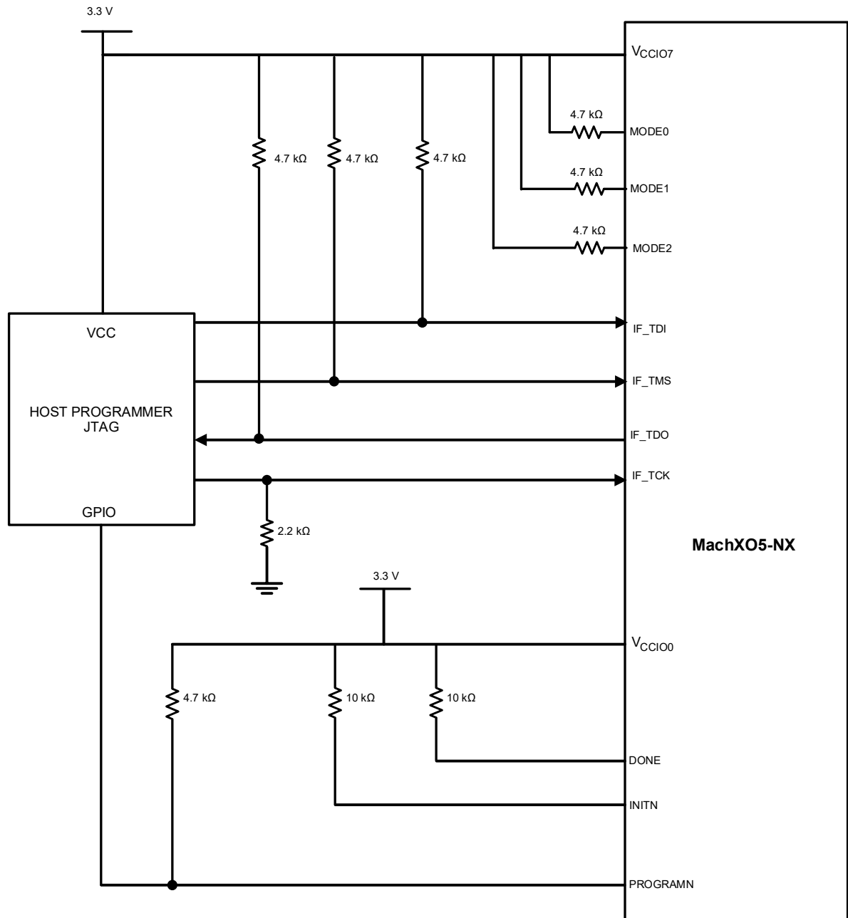
Figure 6.2 Typical Connections for Device Provisioning via JTAG for LFMXO5-55TD/Q and LFMXO5-65TD/Q
