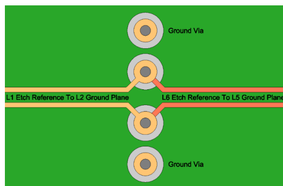
Figure 12.1. Ground Vias Implementation
