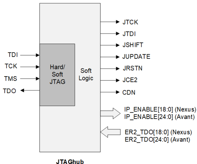
Figure 4: JTAGhub Architecture
