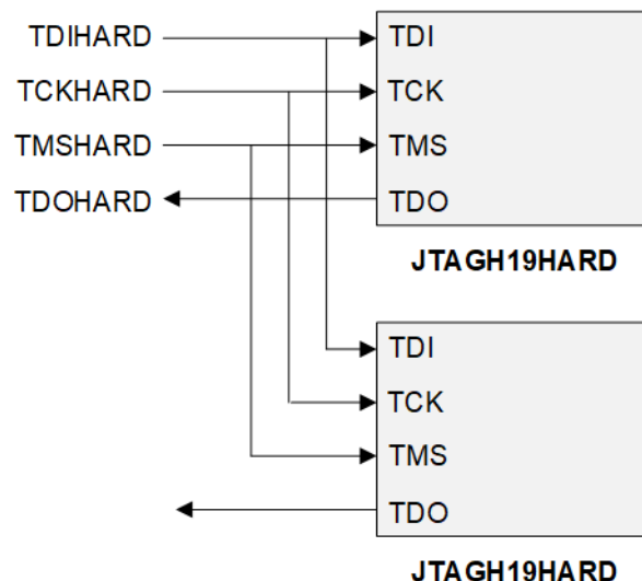
Figure 5: Hard JTAGhub - Merged
