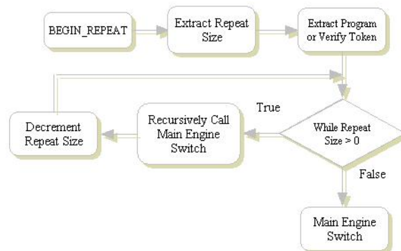
Figure 64: BEGIN_REPEAT Case Statement
