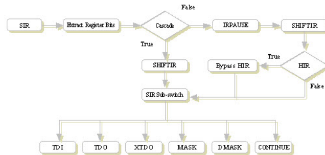
Figure 19: SIR Case Statement
