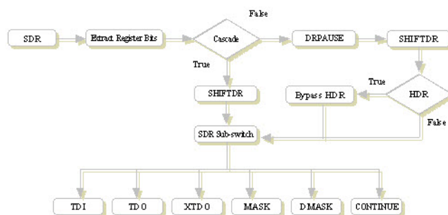
Figure 21: SDR Case Statement
