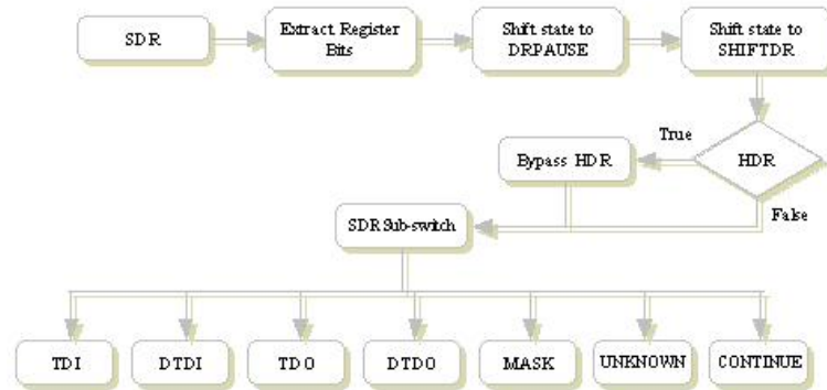
Figure 63: SDR Case Statement Continued
