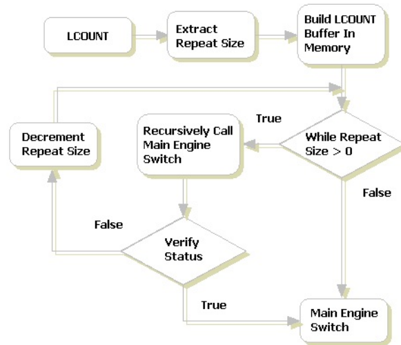
Figure 44: LCOUNT Case Statement
