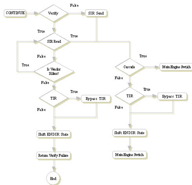
Figure 20: SIR Case Statement Continued
