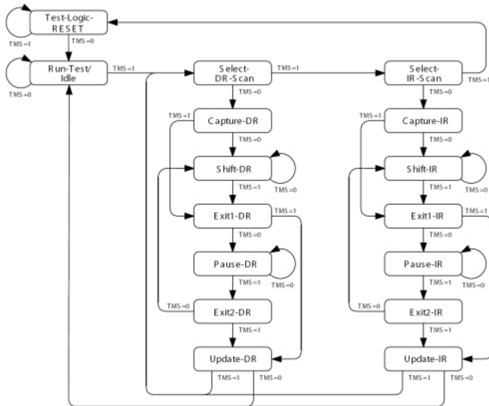
Figure 15: TAP Controller State Diagram
