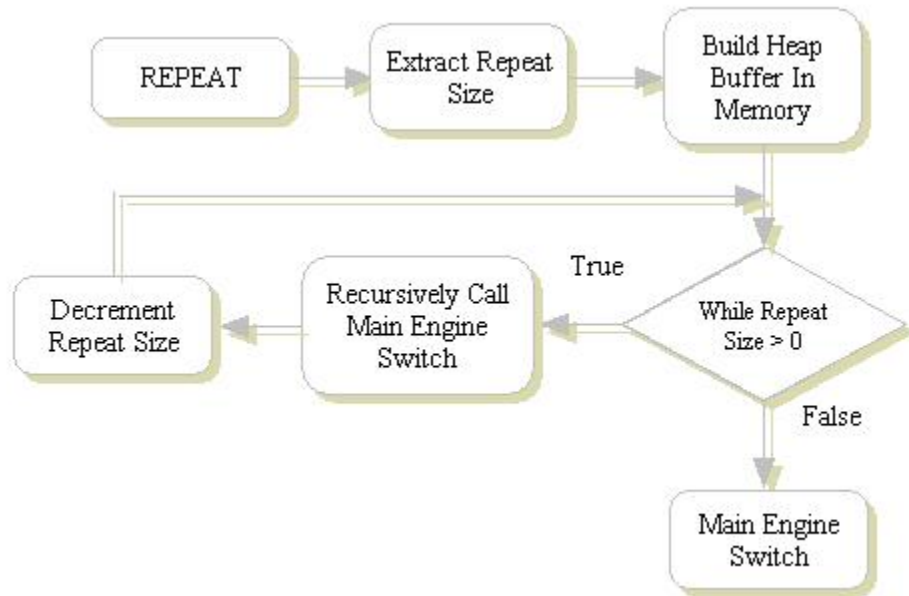
Figure 36: REPEAT Case Statement
