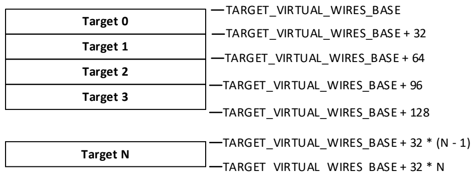
Figure 5.3. Target Virtual Wire Register Allocation
