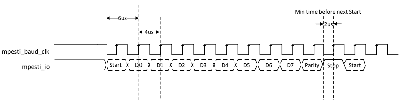
Figure 2.2. M-PESTI UART Frame
