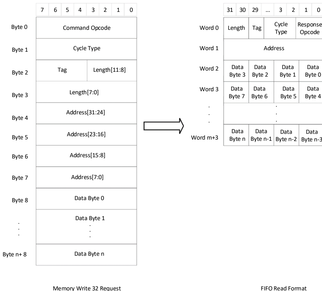
Figure 2.12. FIFO Read Format
