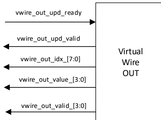
Figure 2.4. Virtual Wire OUT Interface
