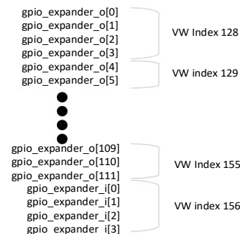
Figure 2.6. Select GPIO Output First
