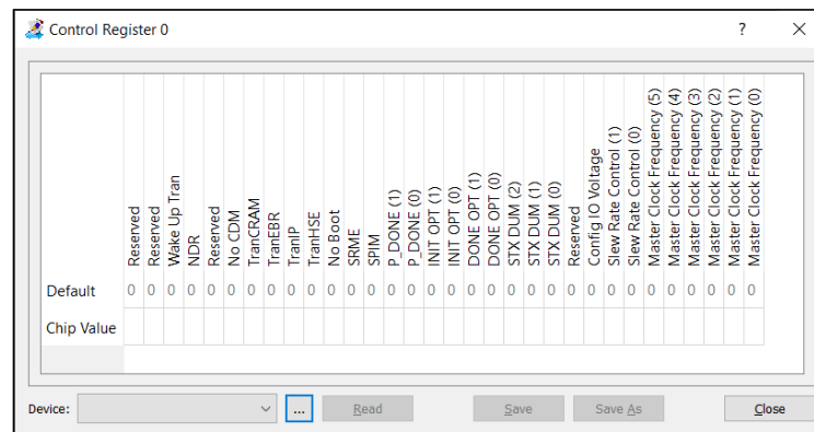
Figure 8.4. Lattice Programming File Utility Control Register GUI
