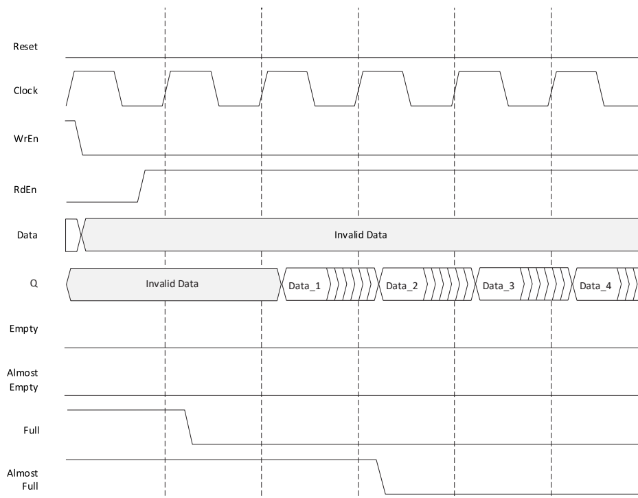
FIFO with Output Registers, Start of Data Read Cycle
