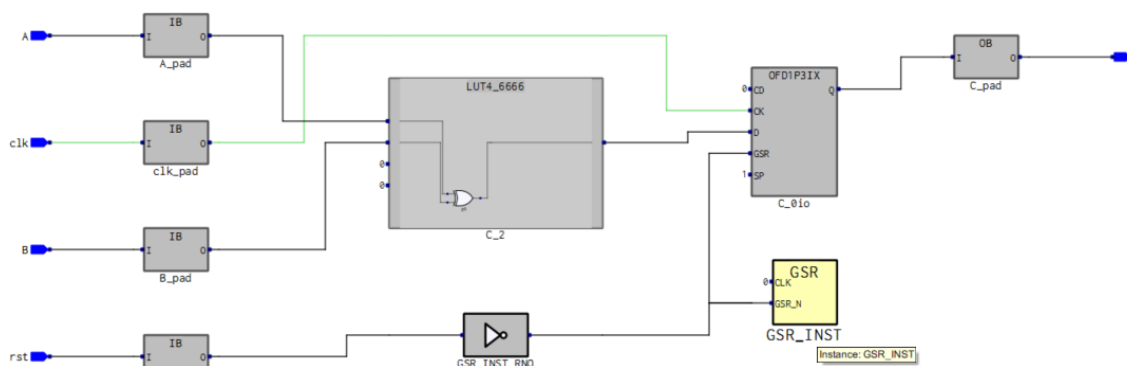
Figure 4.4. RTL View of Input, Output and Clock Buffers Automatically Inferred by Lattice Software
