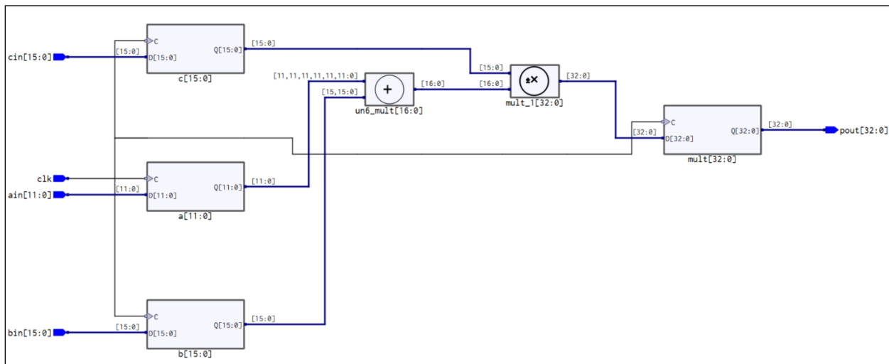
Figure 2.11. Synplify Pro RTL View
