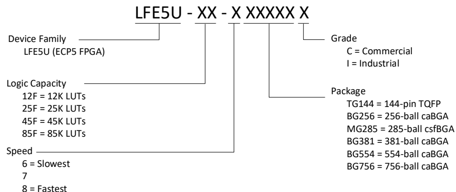
Figure 1.3. Lattice ECP5/ECP5-5G Part Number Description
