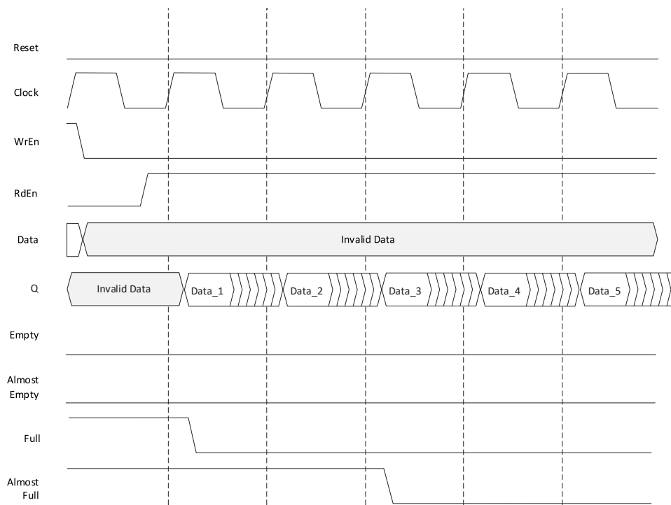
FIFO Without Output Registers, Start of Data Read Cycle
