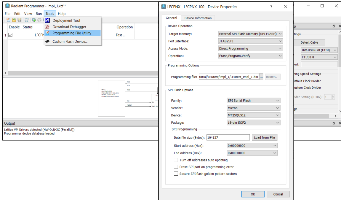
Figure 8.3. Lattice Radiant Programmer GUI
