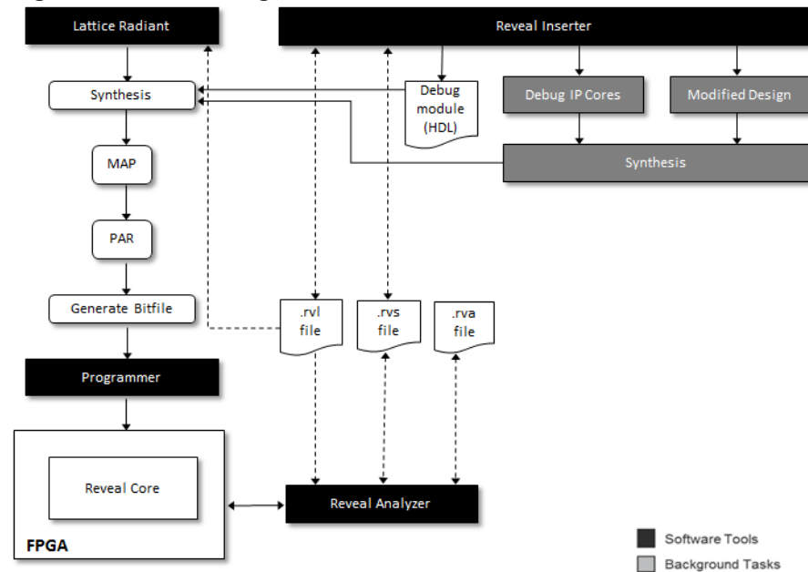
Figure 8: Reveal Design Flow
