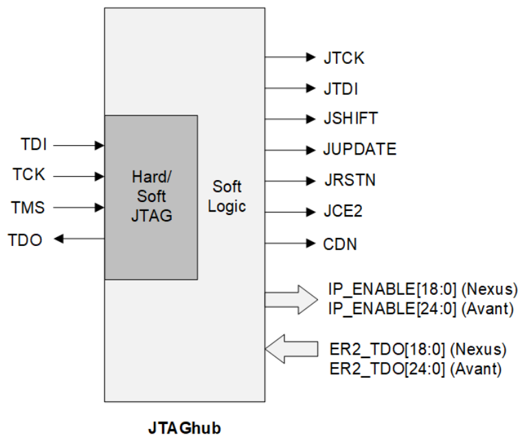
Figure 3: JTAGhub Architecture
