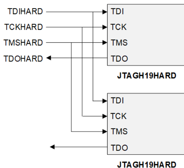
Figure 4: Hard JTAGhub - Merged
