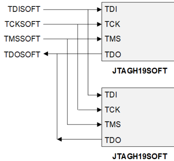
Figure 5: Soft JTAGhub - Merged
