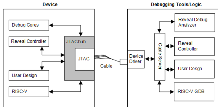
Figure 7: JTAGhub Ecosystem
