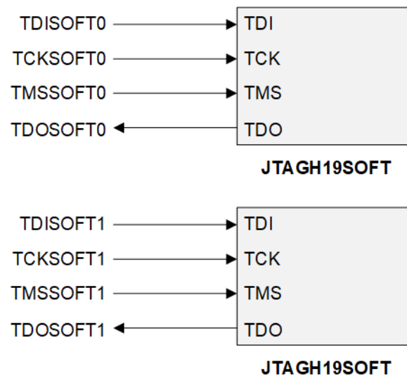
Figure 6: Soft JTAGhub - Not Merged
