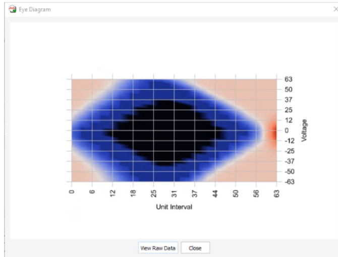
Figure 10: Example of Eye Diagram for Non-Avant Devices
