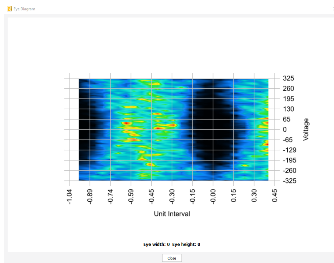
Figure 6: Example of Eye Diagram for Avant Devices
