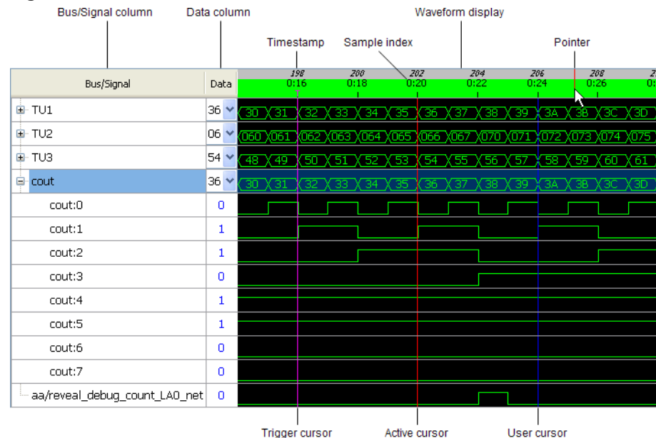
Figure 8: Elements of the LA Waveform View
