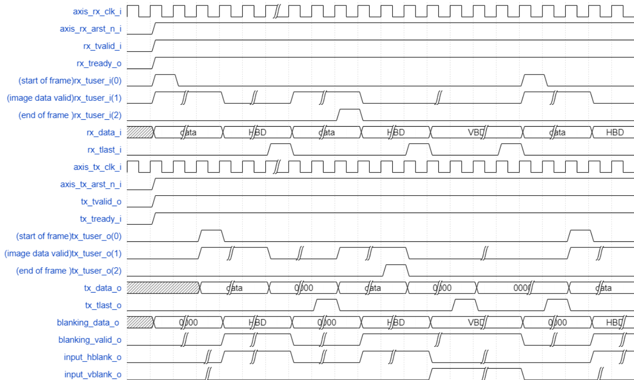
Figure 2.16. AXI-Stream Receiver with Blanking Related Signals for PPC=1(RGB Format)
