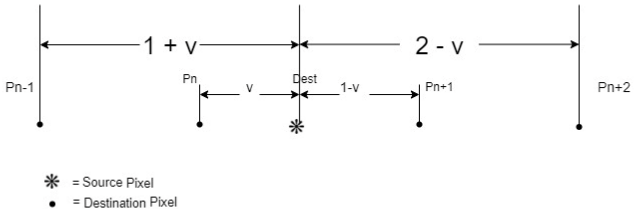
Figure 2.2. Scaling Process with 4-tap Bicubic Filter
