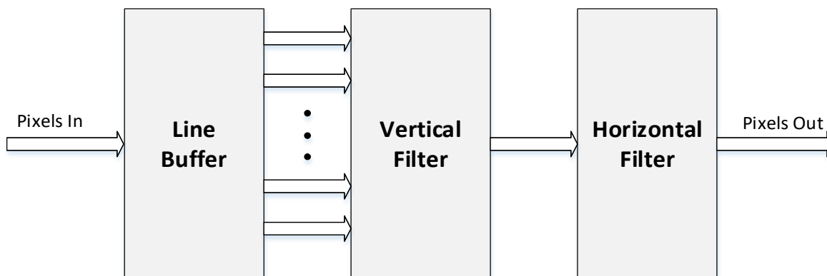
Figure 2.1. Video IP Architecture Diagram
