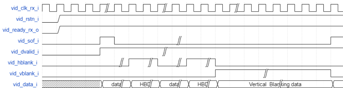
Figure 2.14. Native Input Video Timing Diagram
