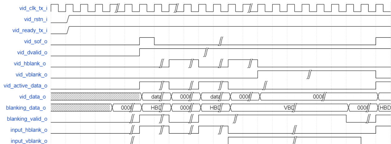
Figure 2.15. Native Output Video Timing Diagram
