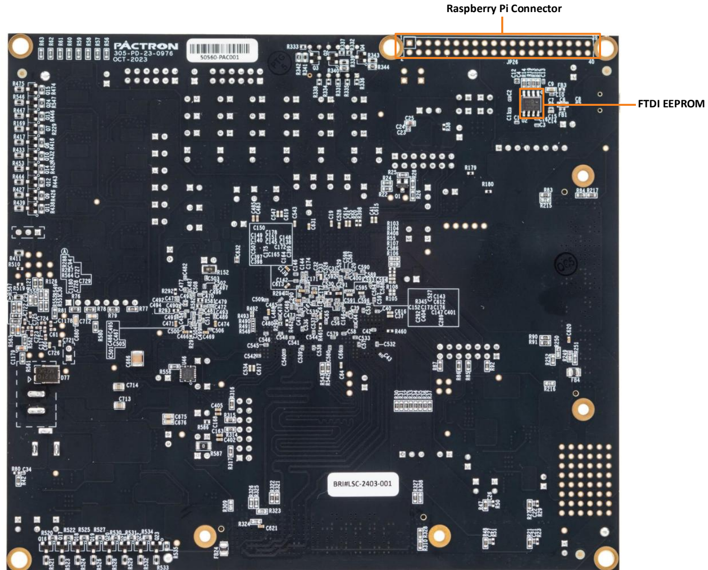
Figure 1.2. Bottom View of Avant-E Evaluation Board
