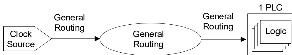
Figure 2.34. Gated Clock to Small Logic Domain
