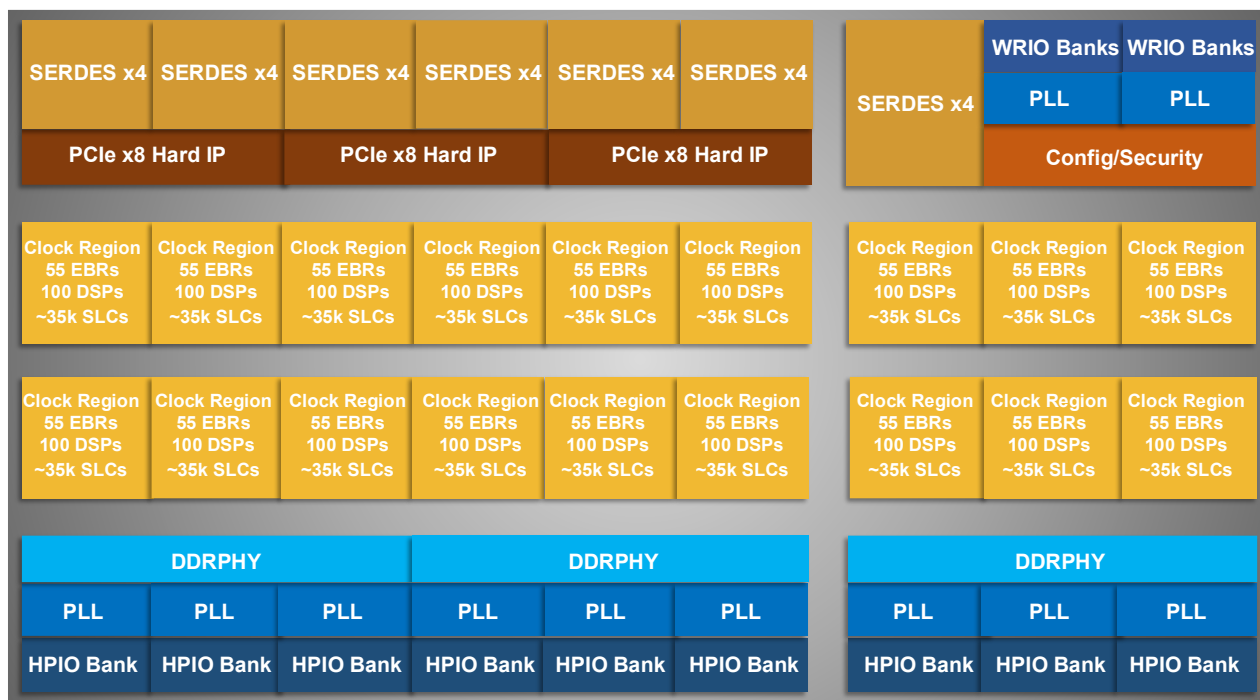
Figure 2.1. Clock Regions (LAV-AT-E/G/X70 Devices)
