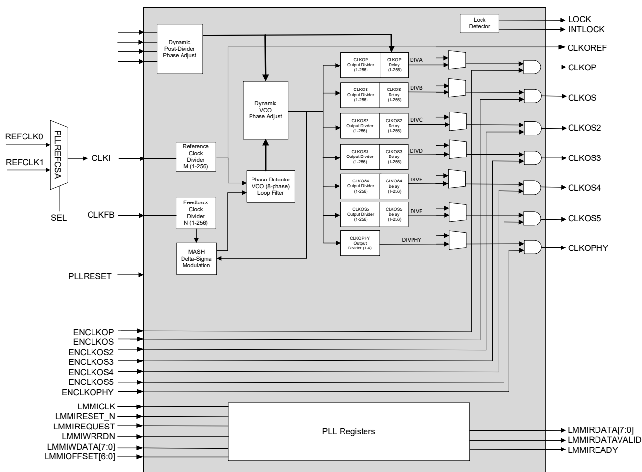
Figure 3.1. Lattice Avant PLL Block Diagram
