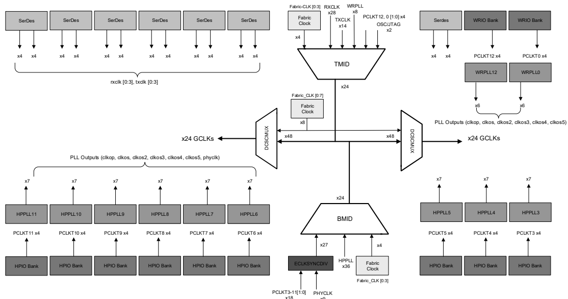
Figure 2.5. Global Clock Routing Architecture for LAV-AT-E/G/X70 Devices
