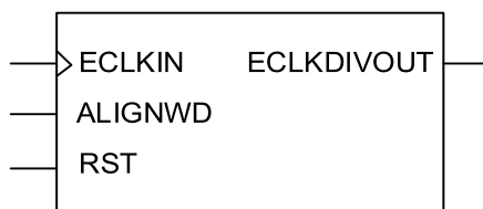
Figure 2.15. ECLKDIVA Component Symbol
