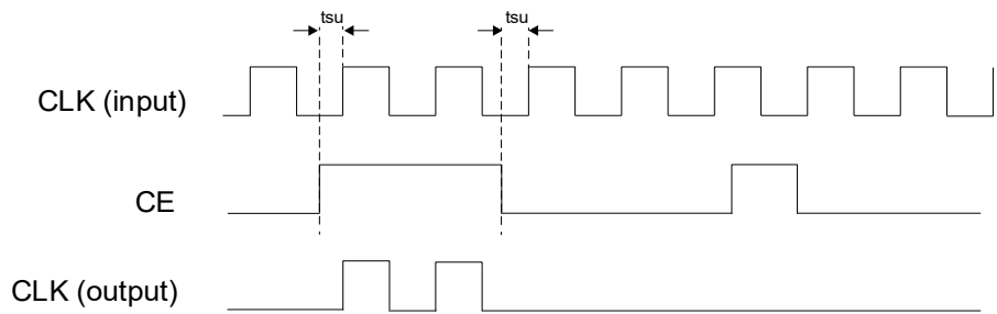
Figure 2.30. Glitchless DCC Functional Waveform
