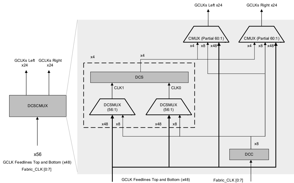
Figure 2.6. DCSCMUX
