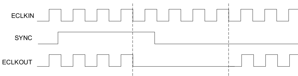
Figure 2.14. ECLKSYNCA Functional Waveform
