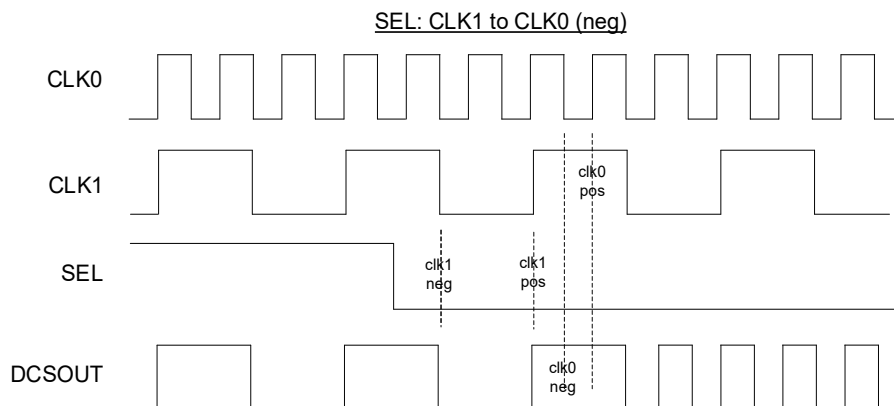
Figure 2.22. Negedge DCS Switch from SEL: 1 ≥ 0
