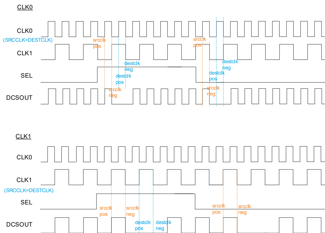
Figure 2.23. DCSMODE = CLK0 or CLK1
