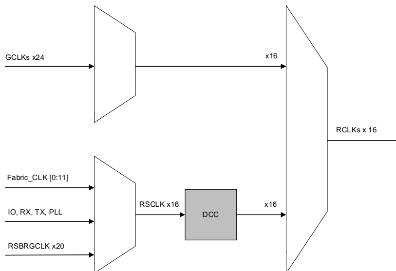
Figure 2.8. Generic RGMUX Implementation
