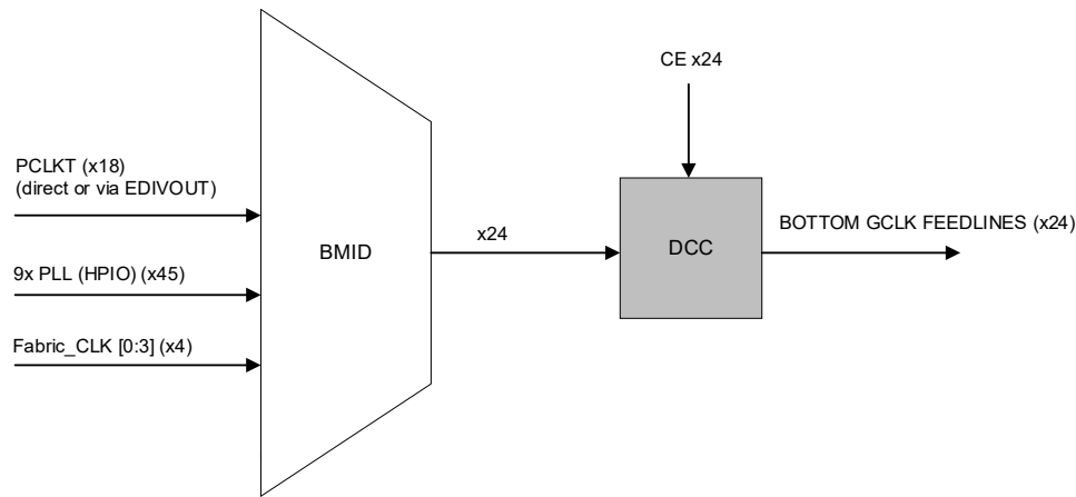
Figure 2.29. BMID Multiplexer, DCC Elements, and Bottom GCLK Feedlines
