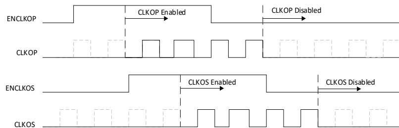
Figure 3.8. Dynamic Clock Enable for PLL Outputs
