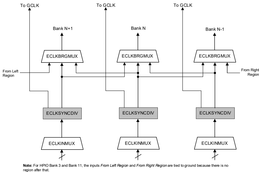
Figure 2.11. Edge Clock Sources Bridged to Multiple Banks
