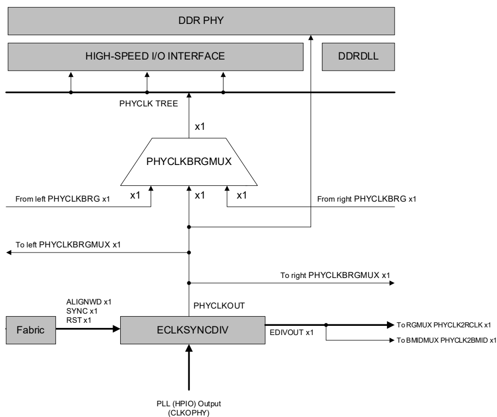
Figure 2.12. PHYCLK Network
