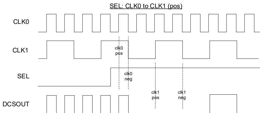
Figure 2.19. Posedge DCS Switch from SEL: 0 ≥ 1
