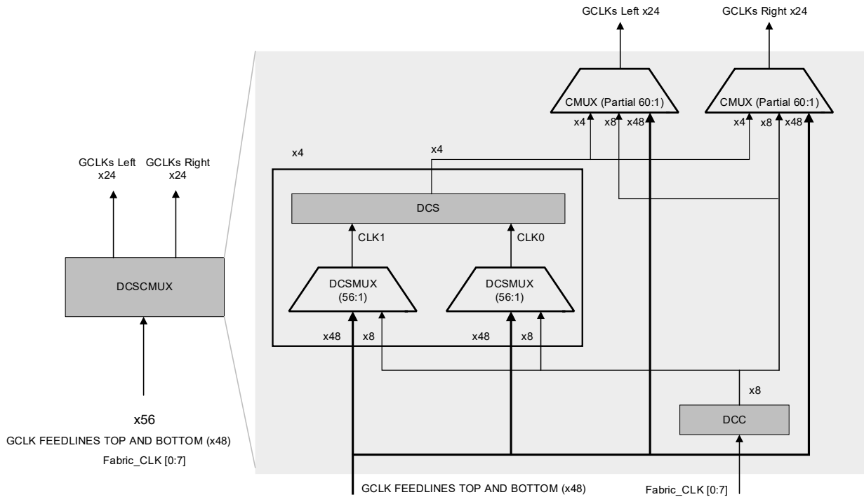
Figure 2.18. DCSCMUX
