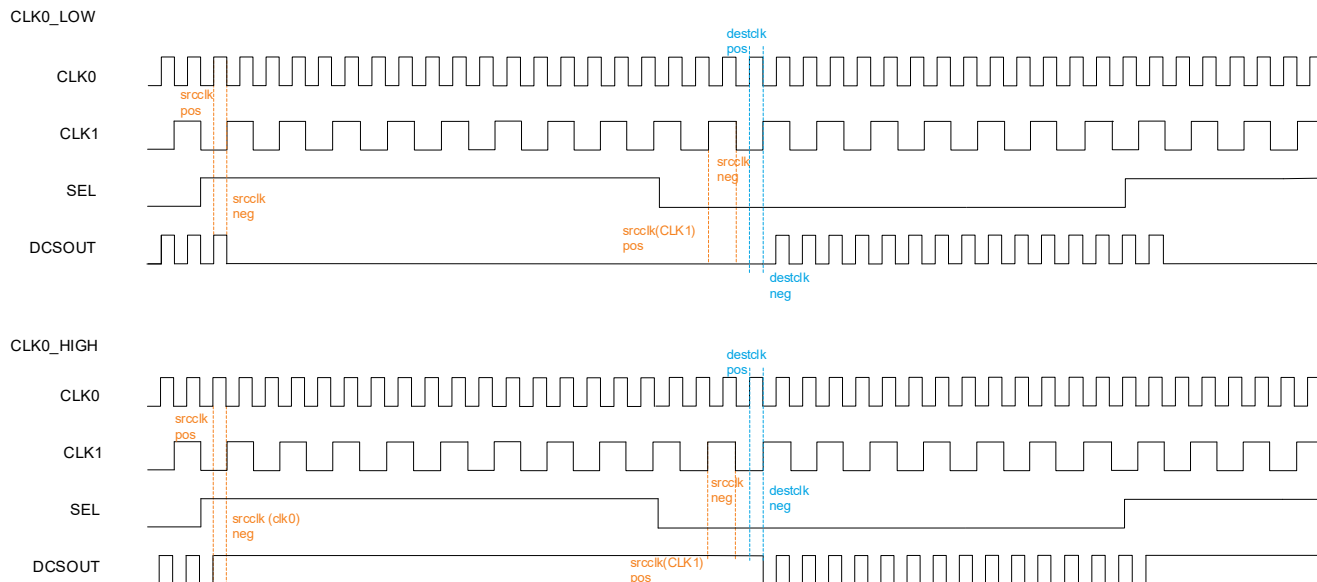
Figure 2.24. DCSMODE = CLK0_LOW or CLK0_HIGH
