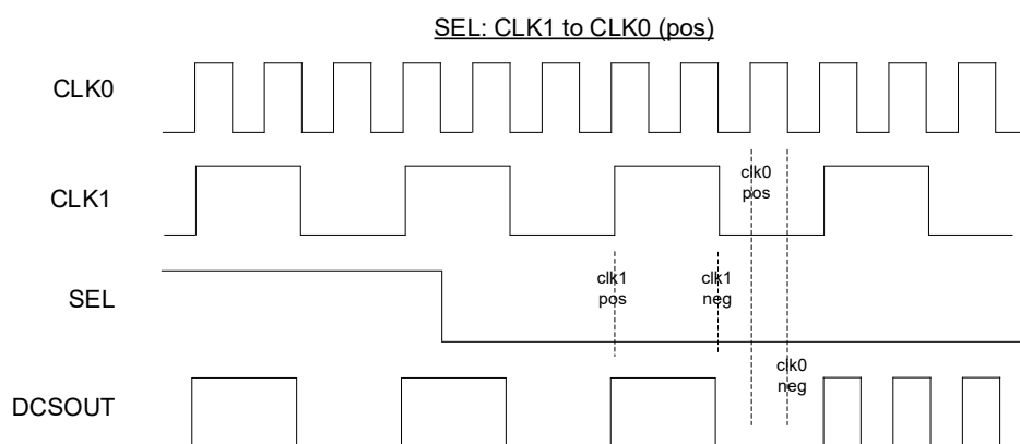
Figure 2.20. Posedge DCS Switch from SEL: 1 ≥ 0
