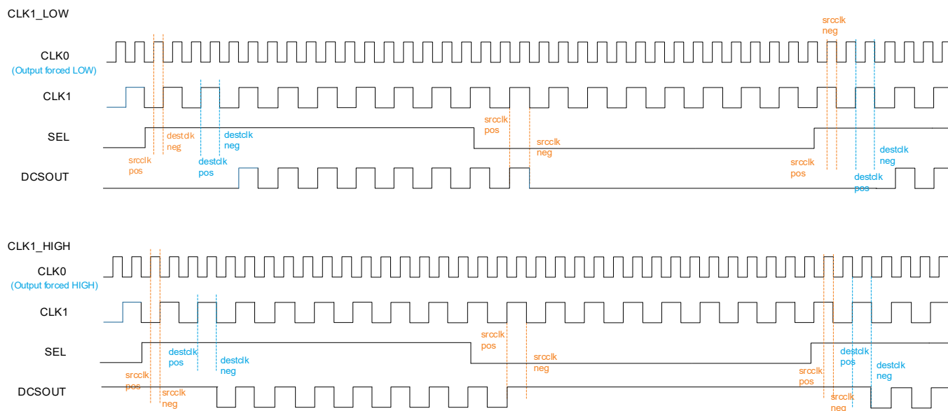
Figure 2.25. DCSMODE = CLK1_LOW or CLK1_HIGH
