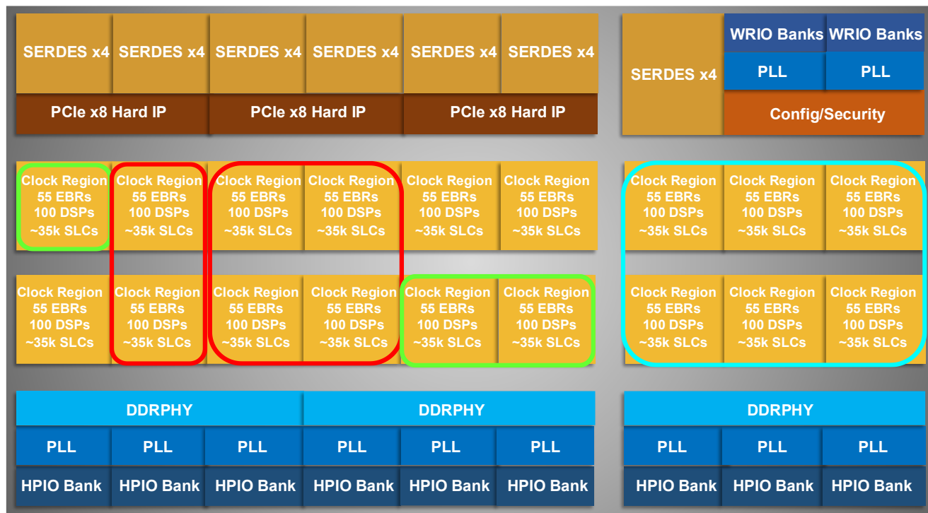
Figure 2.7. Multi-Region Clock Formations
