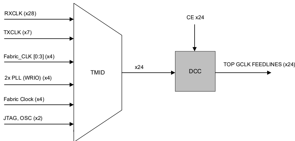
Figure 2.28. TMID Multiplexer, DCC Elements, and Top GCLK Feedlines
