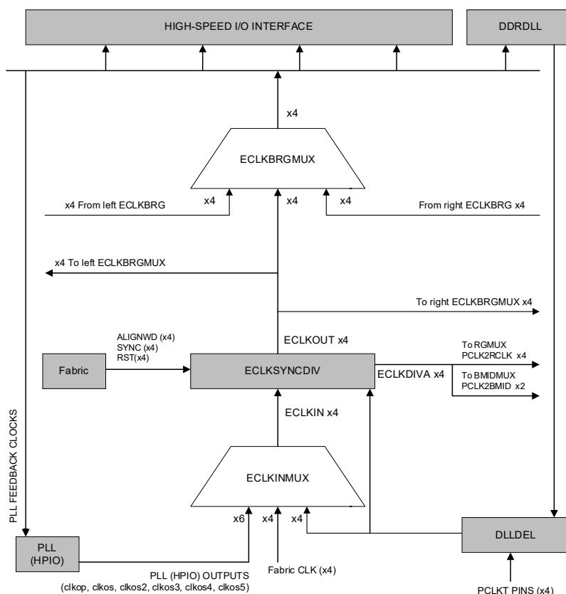
Figure 2.9. Edge Clock Sources per Bank
