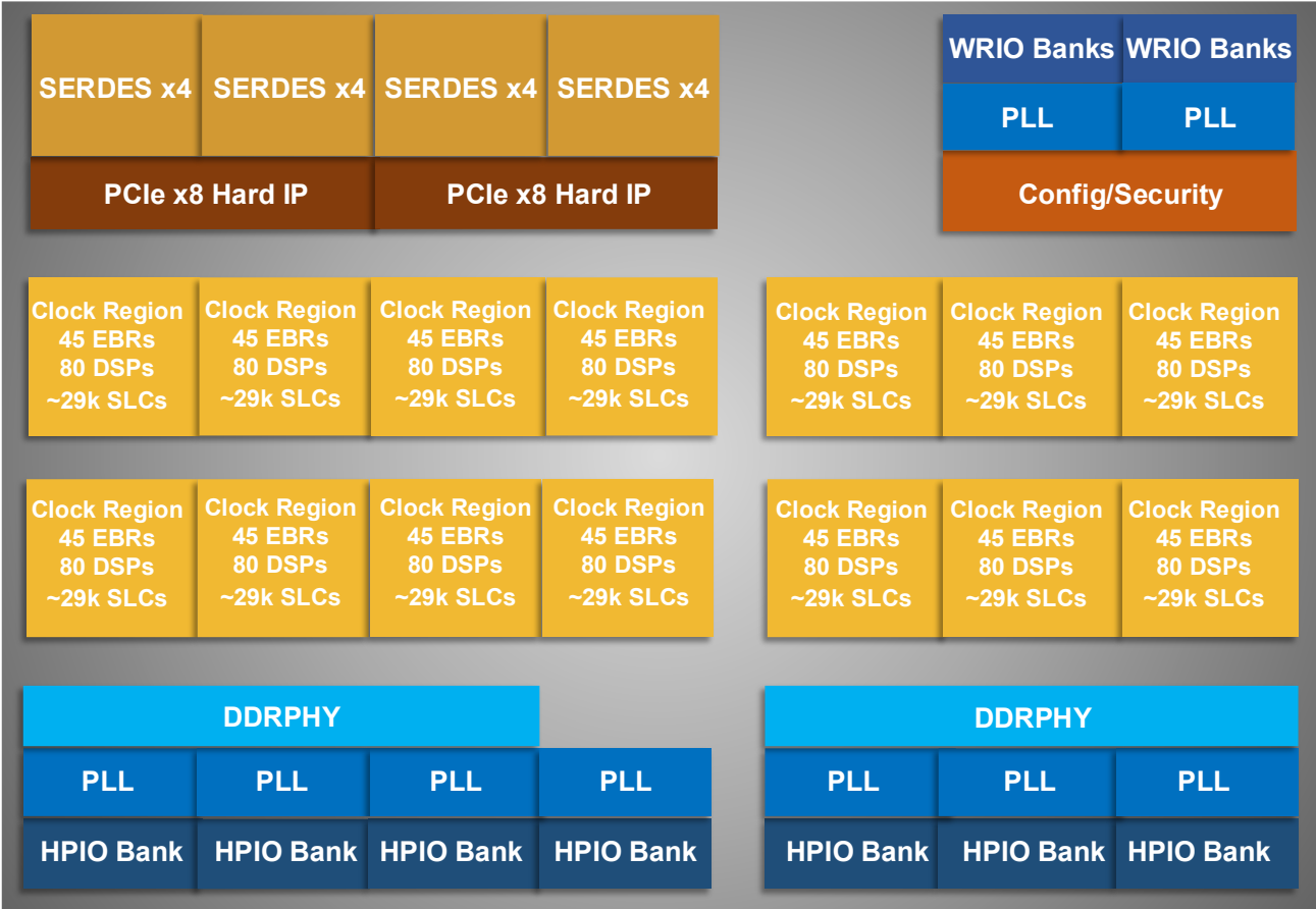
Figure 2.2. Clock Regions (LAV-AT-E/G/X50 Devices)
