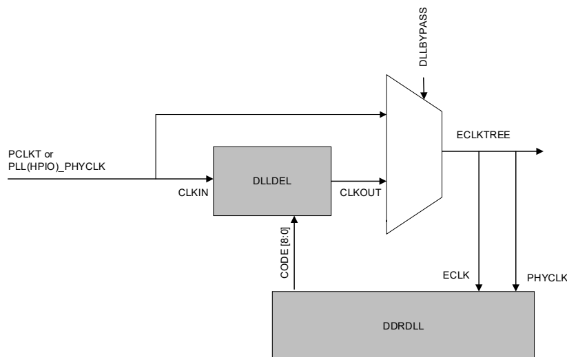
Figure 2.16. High-Level Implementation of DLLDEL and Code Control
