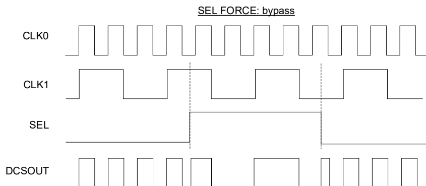
Figure 2.26. MODESEL = 1 DCS Clock Switch
