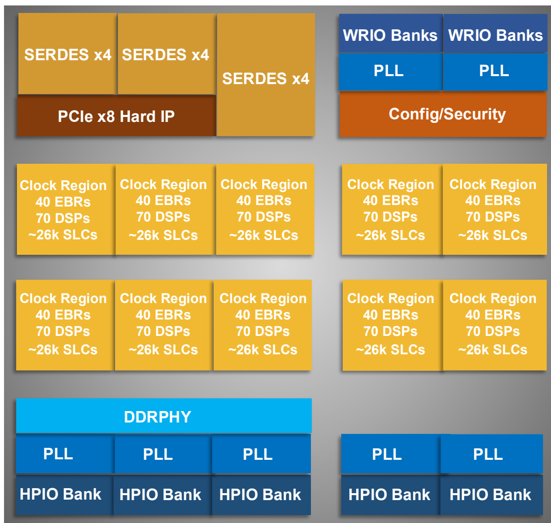
Figure 2.3. Clock Regions (LAV-AT-E/G/X30 Devices)
