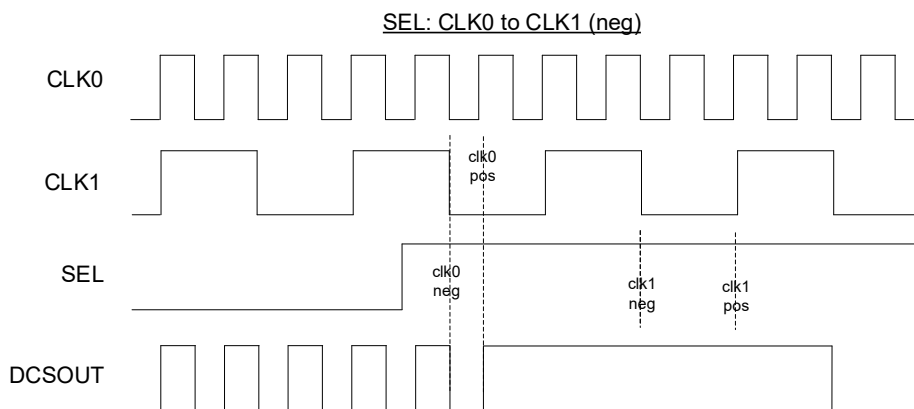
Figure 2.21. Negedge DCS Switch from SEL: 0 ≥ 1
