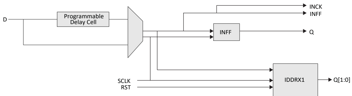
Figure 2.24. Input Register Block for PIO on Top, Left, and Right Sides of the Device
