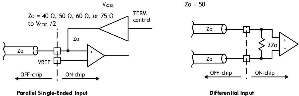
Figure 4.1. On-Chip Termination
