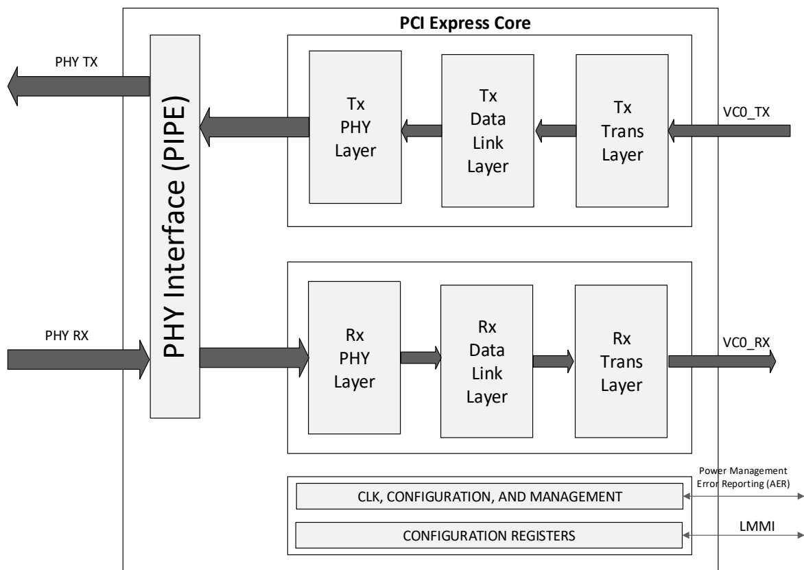
Figure 2.35. PCIe Core
