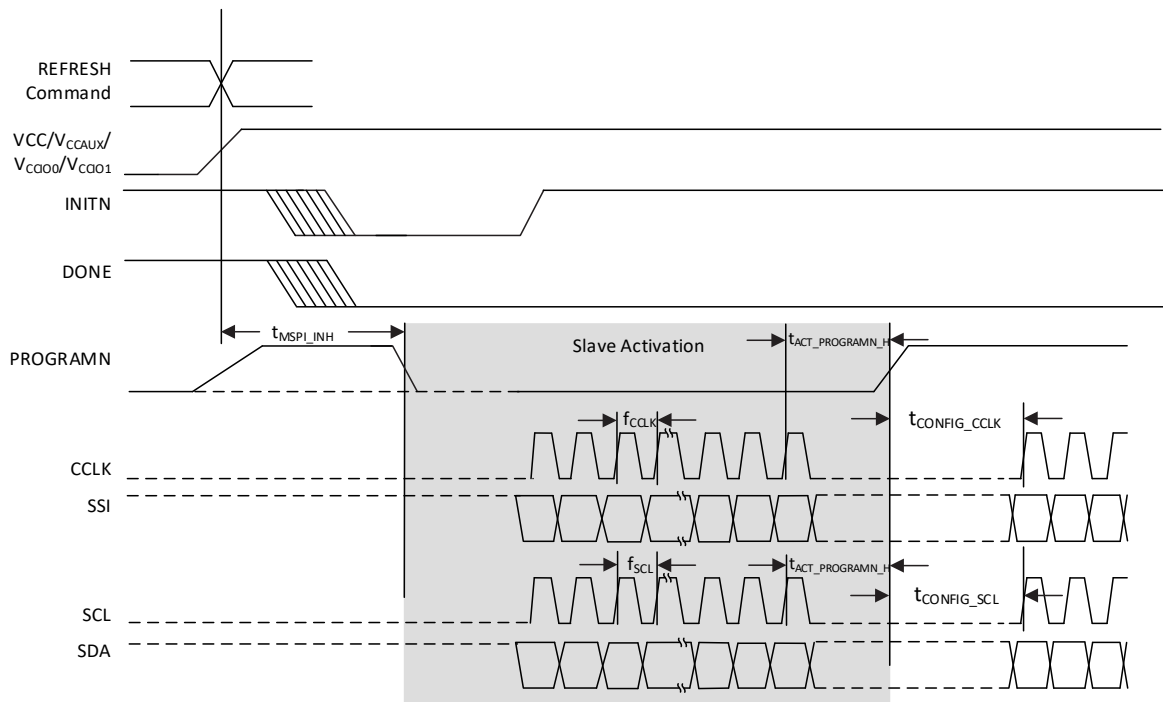
Figure 3.15. Slave SPI/I2C/I3C POR/REFRESH Timing
