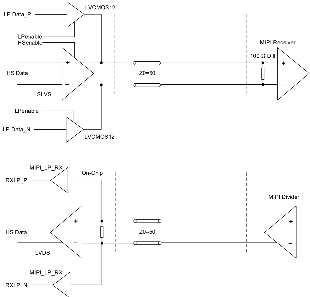
Figure 4.6. MIPI Interface
