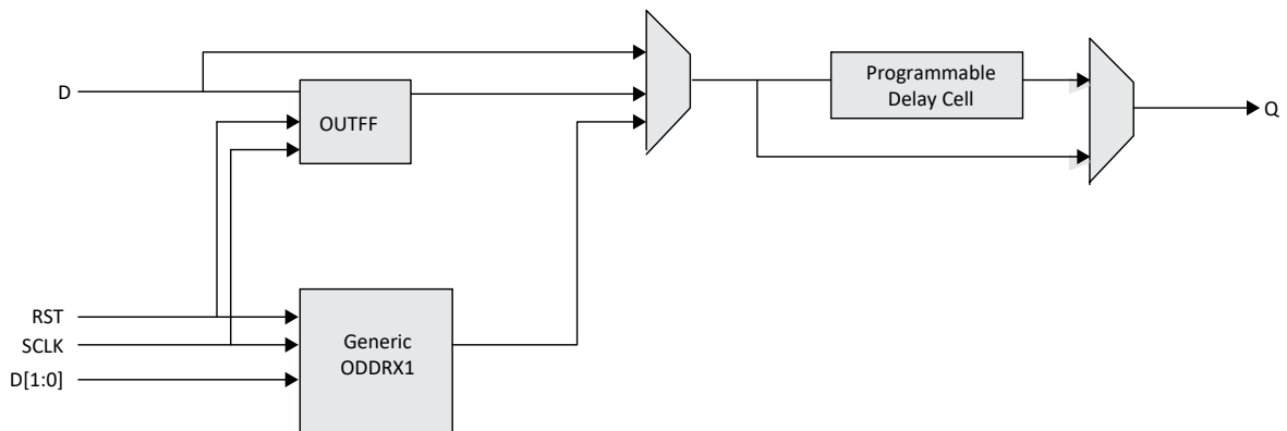
Figure 2.26. Output Register Block on Top, Left, and Right Sides
