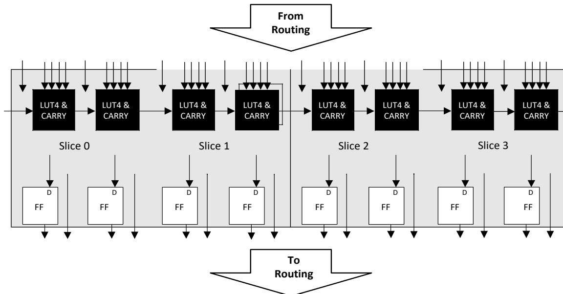
Figure 2.5. PFU Diagram
