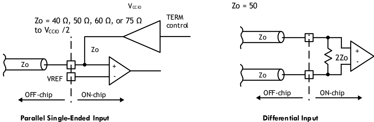
Figure 3.1. On-Chip Termination
