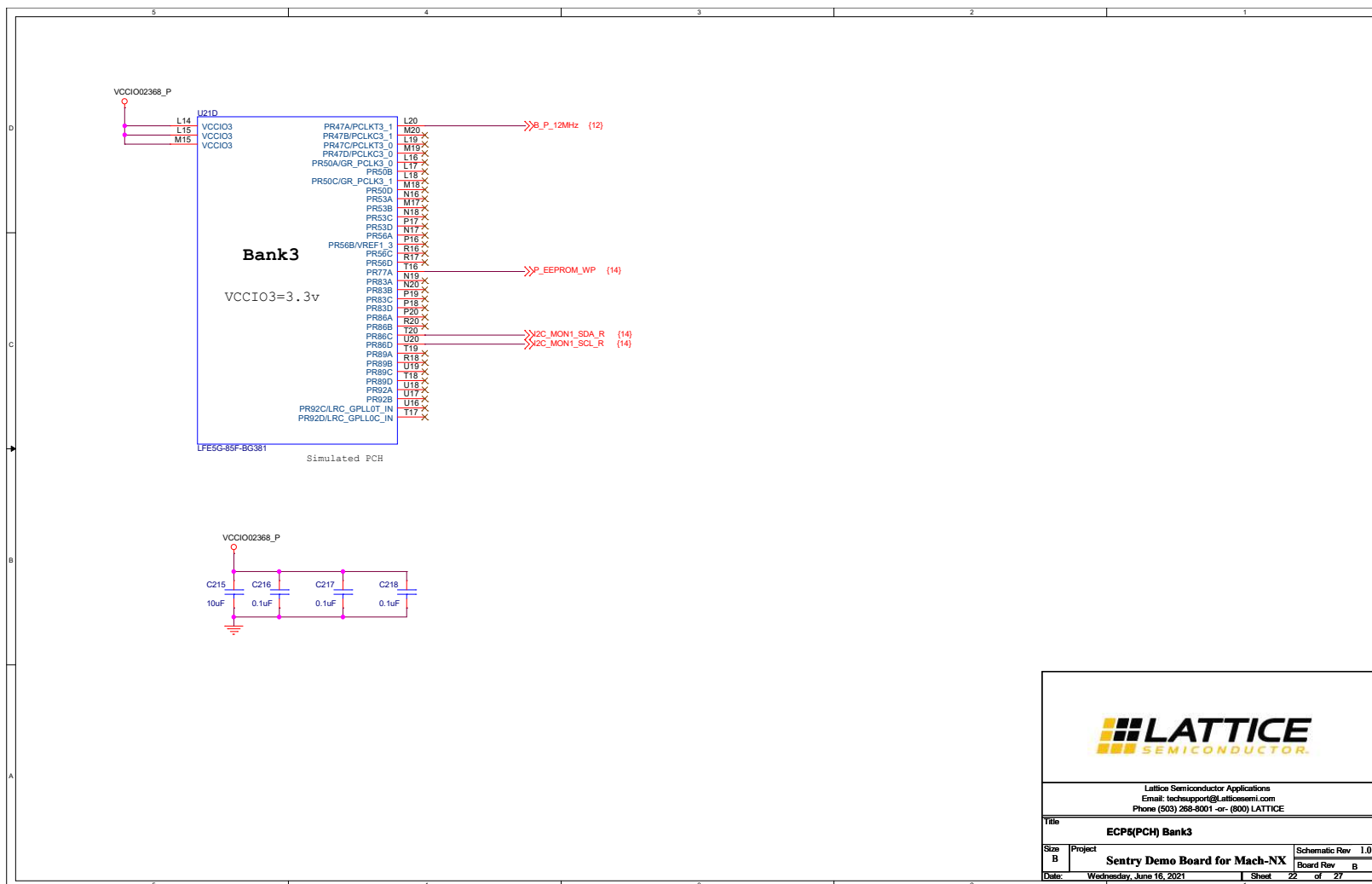
Figure A.22. ECP5(PCH) Bank3
