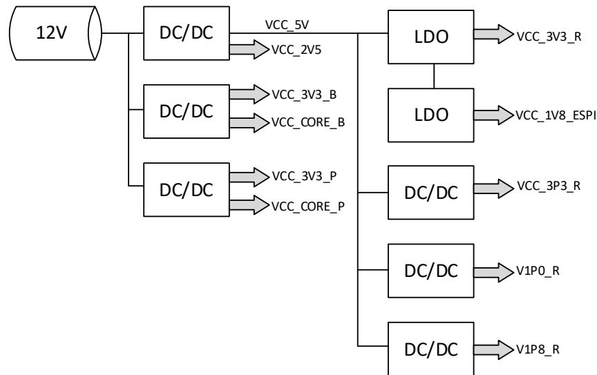
Figure 3.1. Power Supply Architecture
