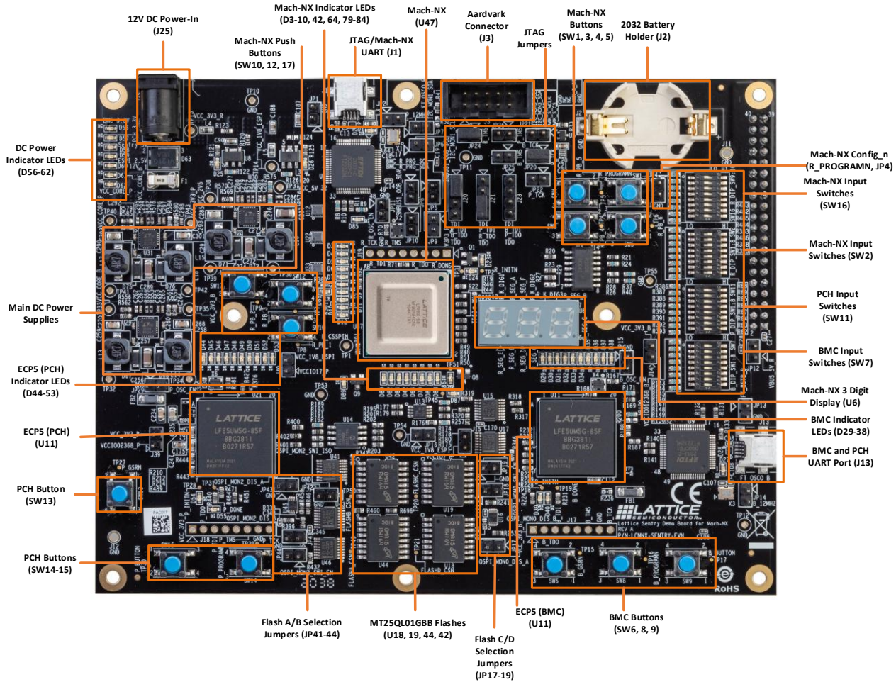
Figure 1.1. Lattice Sentry Demo Board for Mach-NX, Top View
