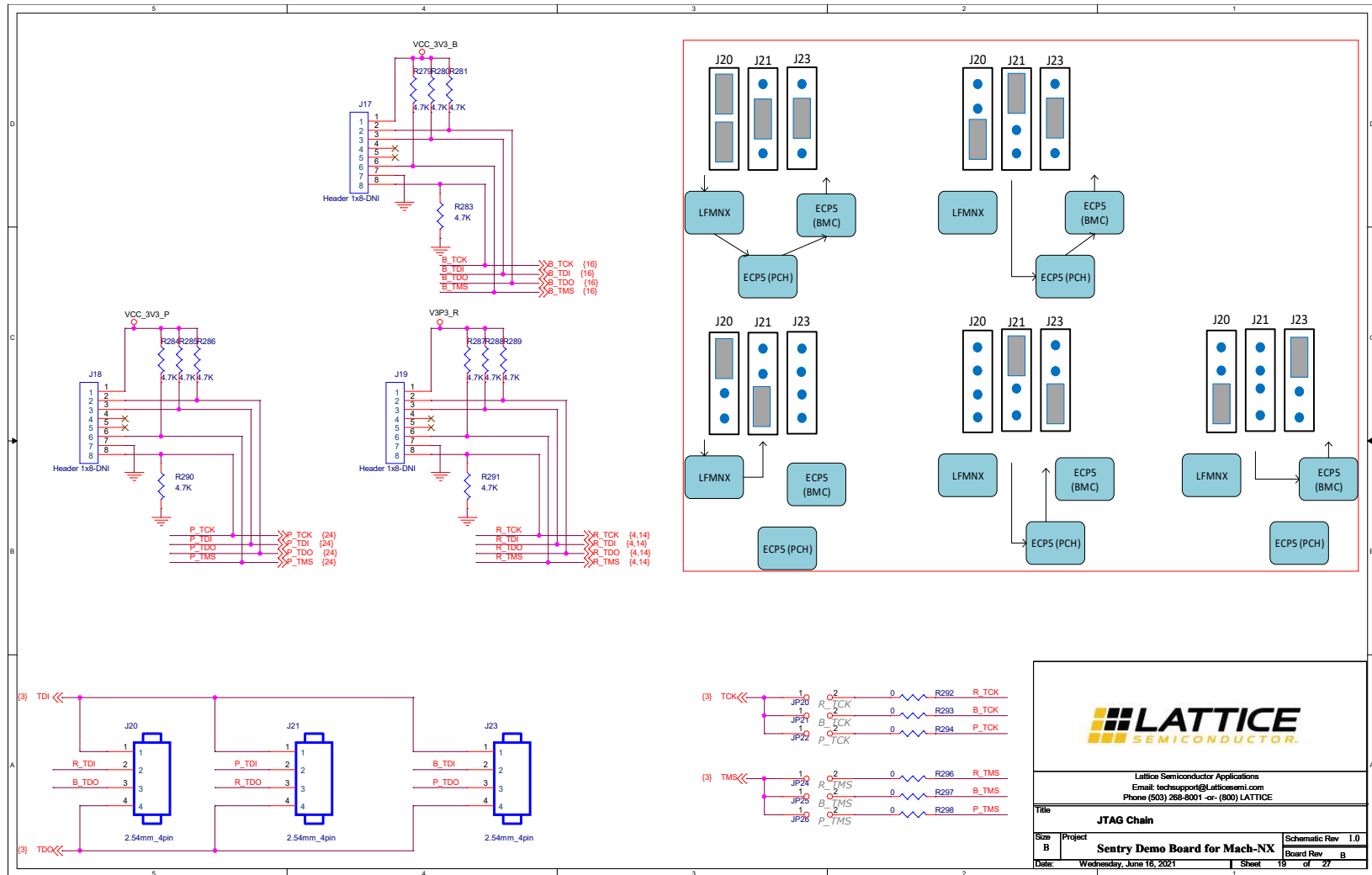
Figure A.19. JTAG Chain
