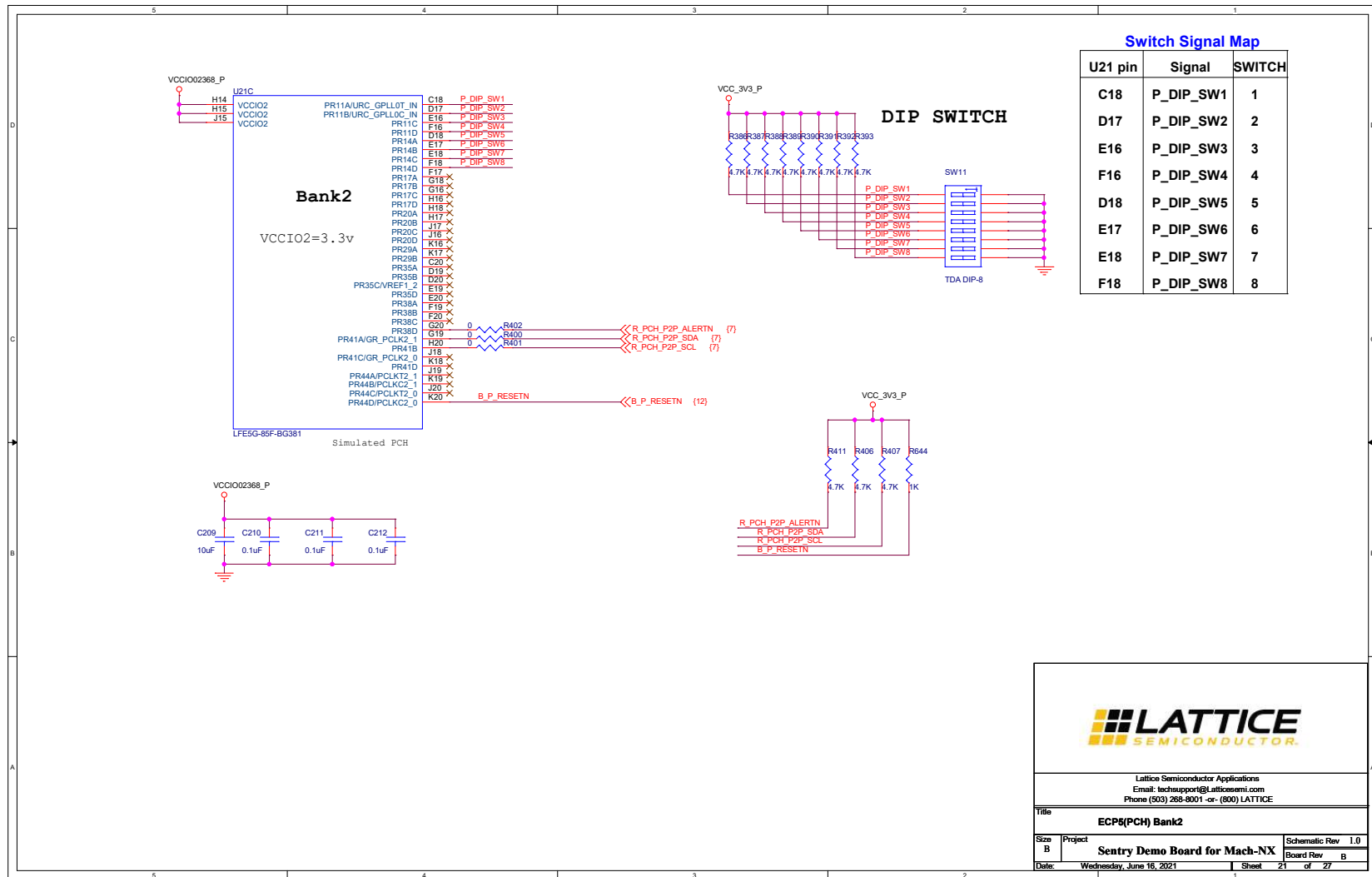
Figure A.21. ECP5(PCH) Bank2
