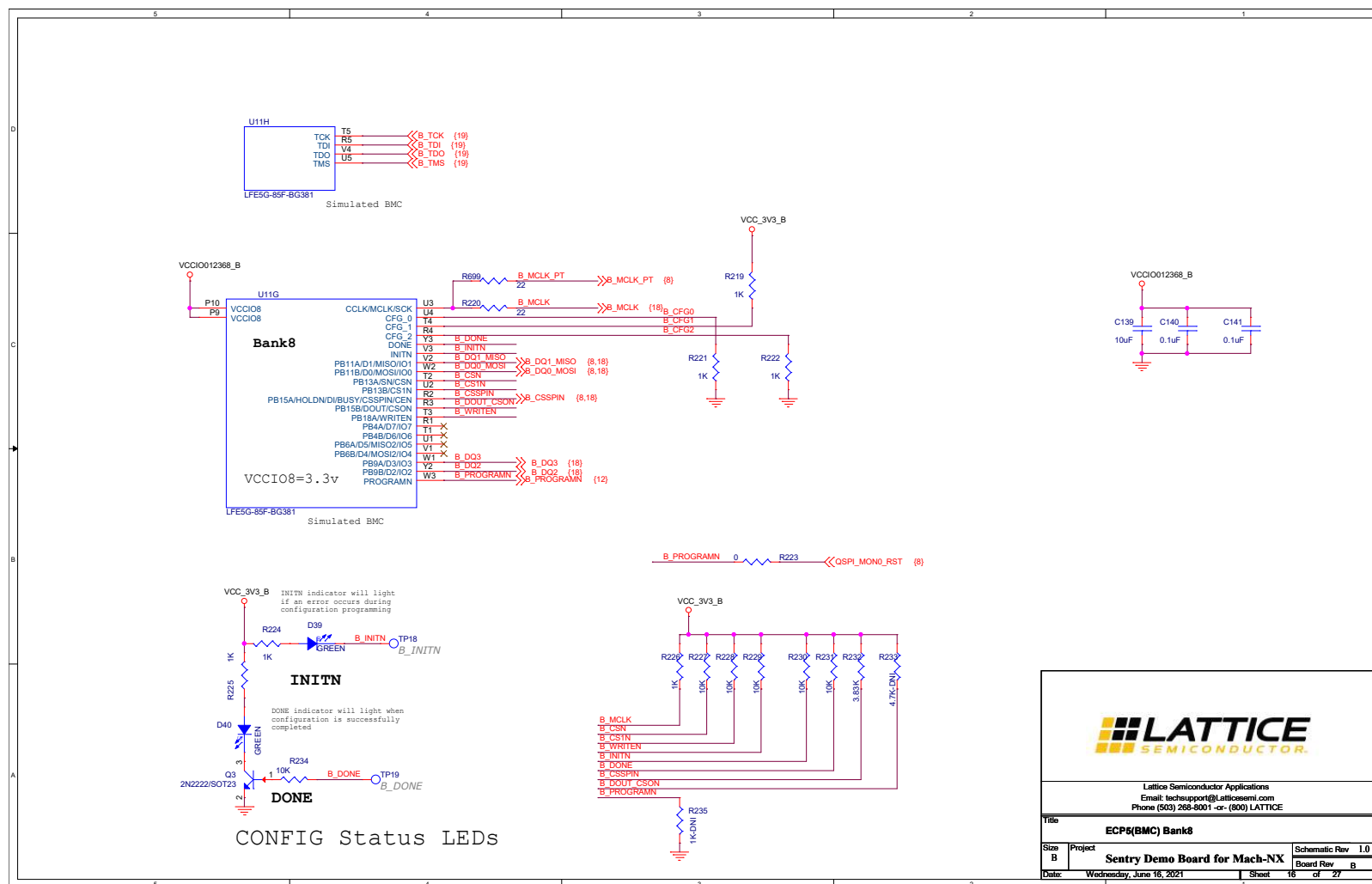
Figure A.16. ECP5(BMC) Bank8
