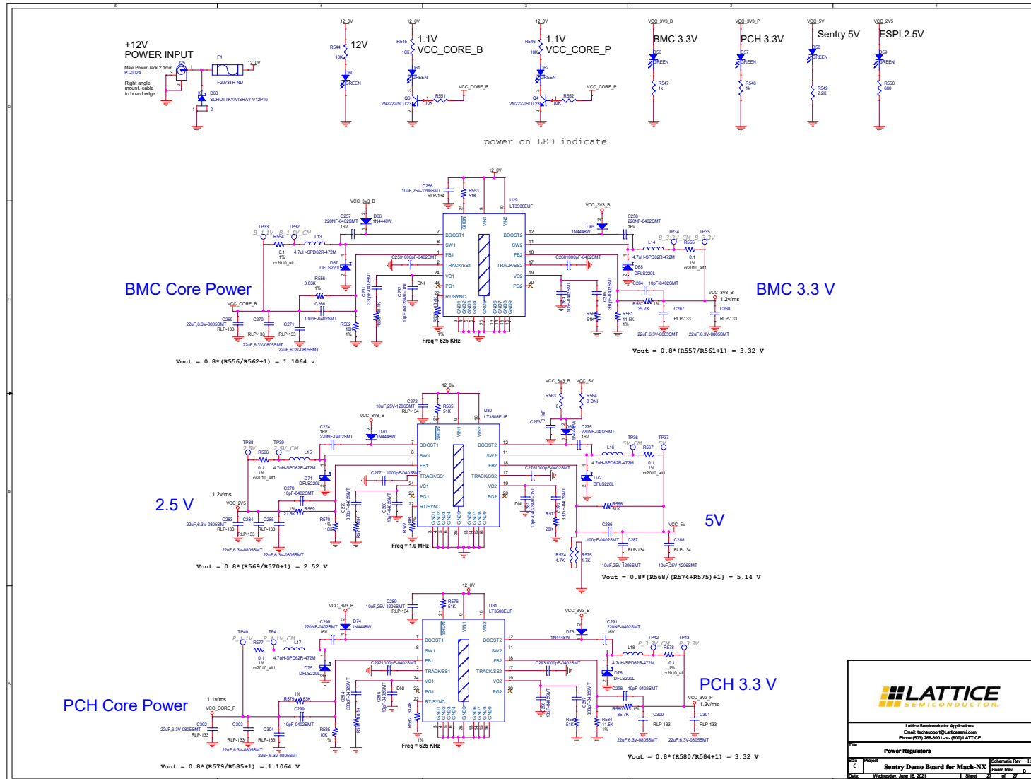
Figure A.27. Power Regulators
