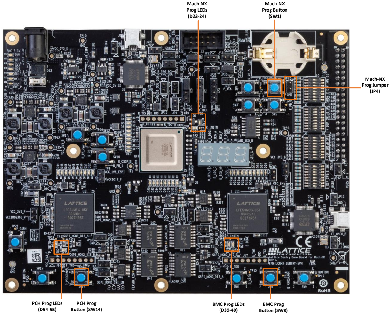
Figure 4.4. Location of Configuration Buttons and LEDs
