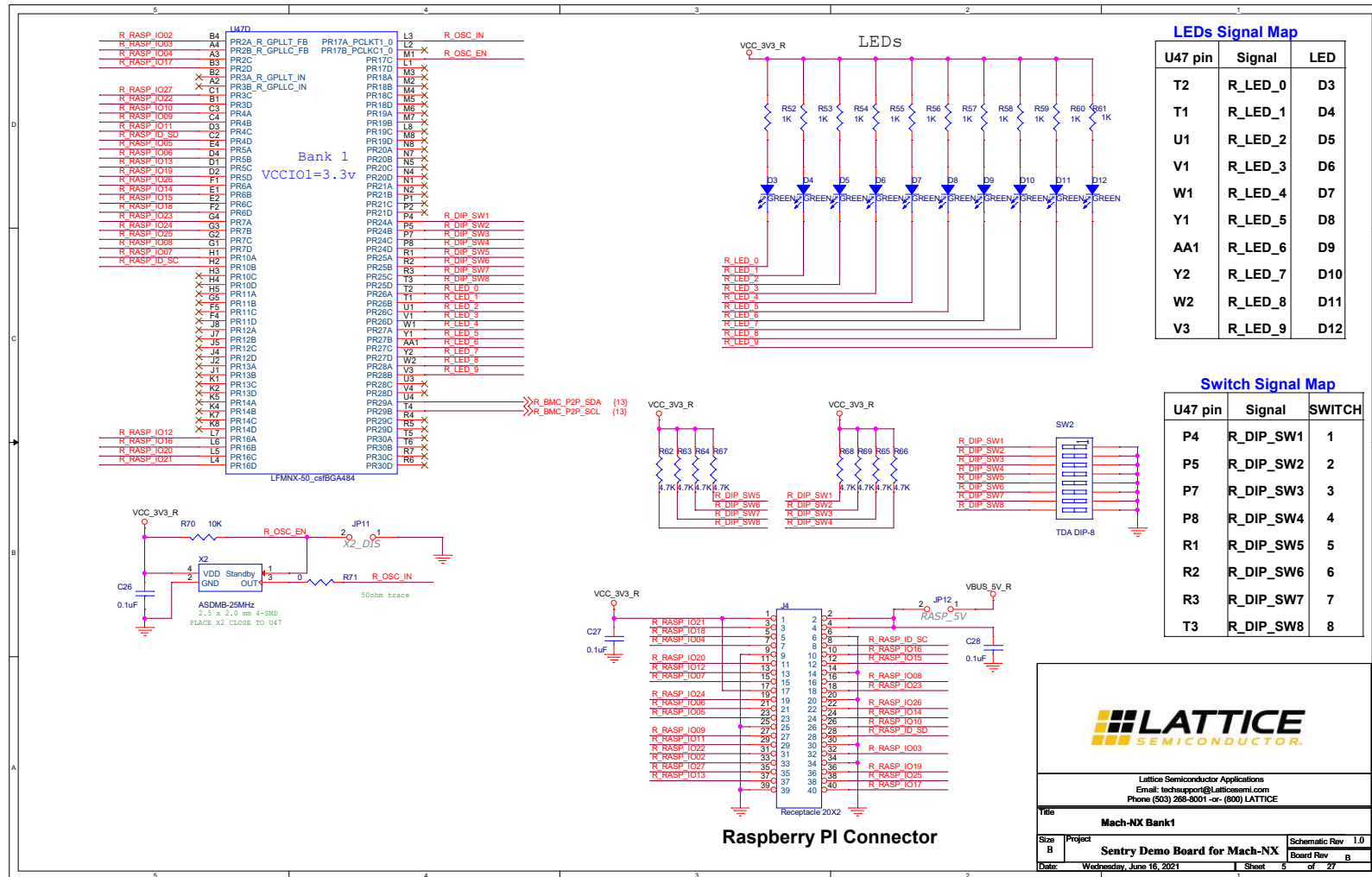
Figure A.5. Mach-NX Bank1
