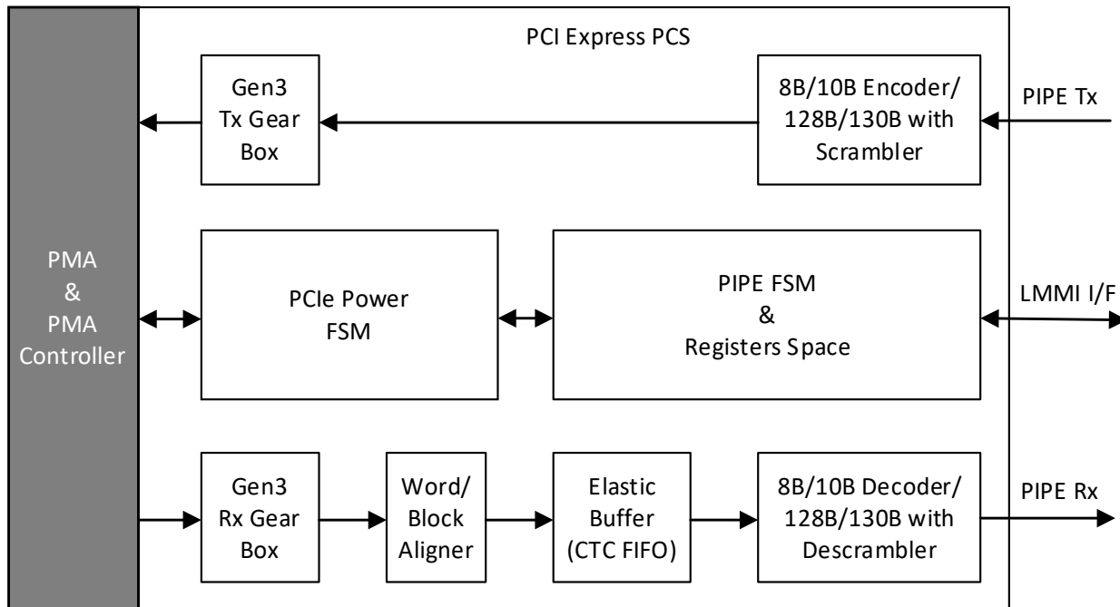
Figure 6.4. PCI Express PCS & PMA Controller Block Diagram
