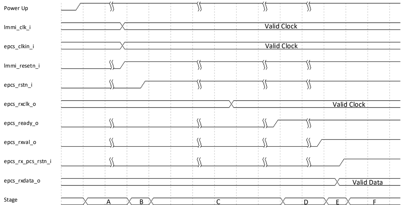
Figure 7.22. EPCS Mode Reset Sequence (Rx Path)
