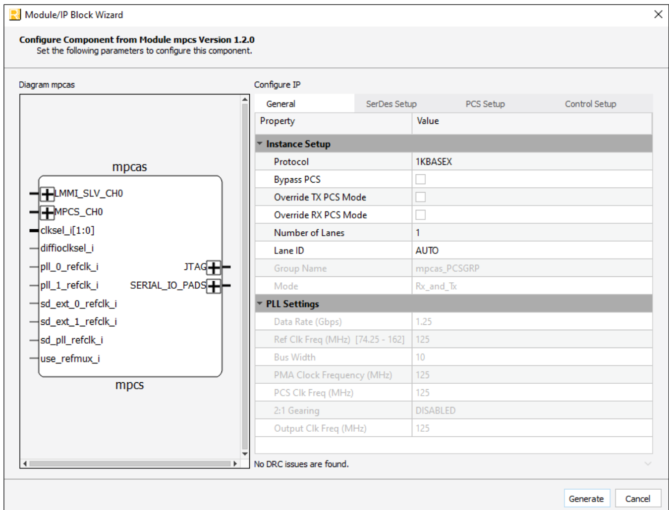
Figure 14.1. MPCAS Configuration GUI
