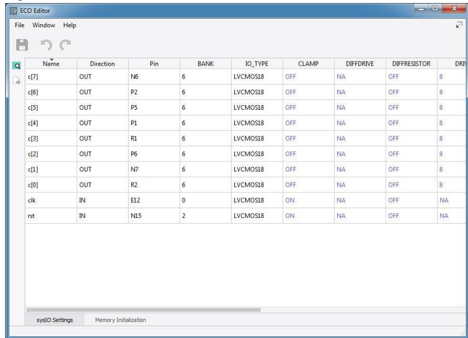
Figure 74: ECO Editor
