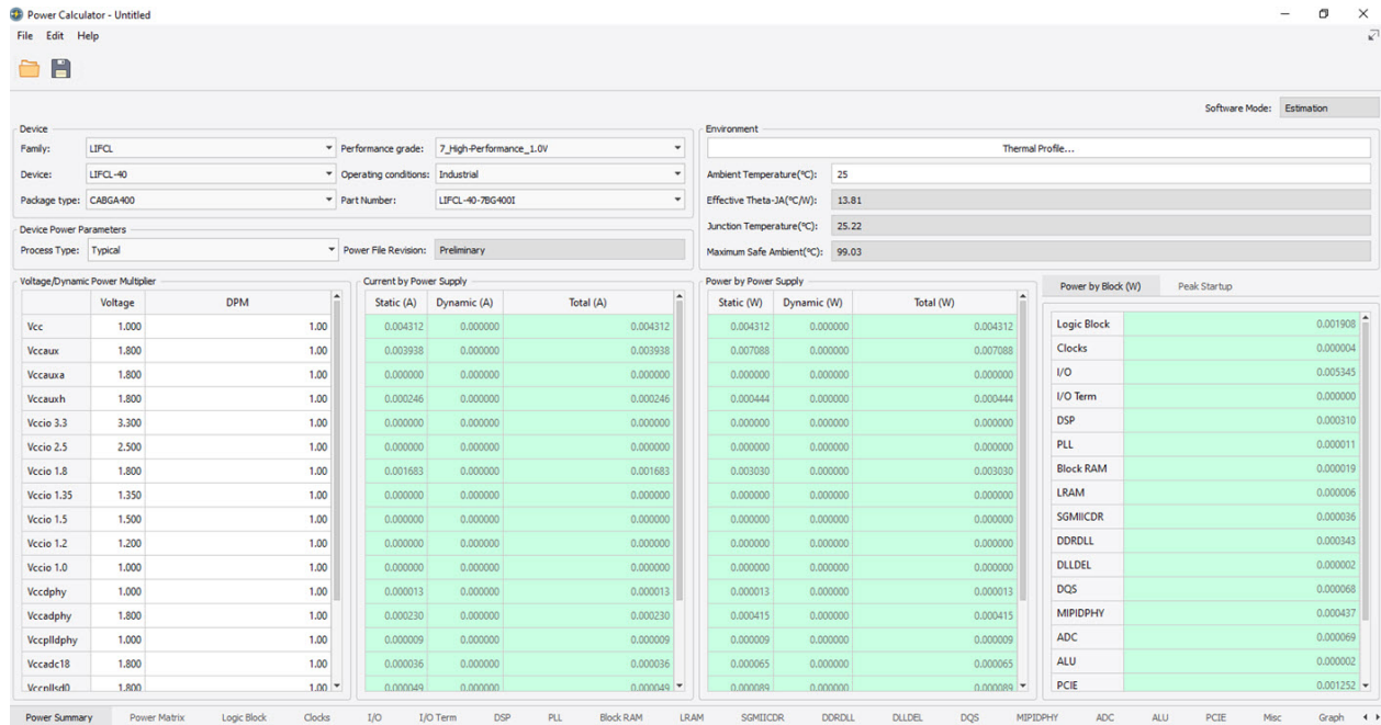
Figure 73: Power Calculator
