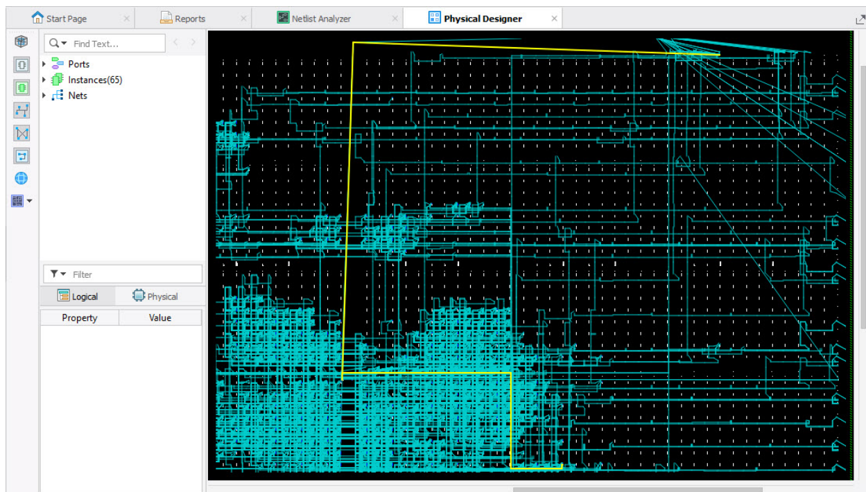
Figure 71: Routing Mode
