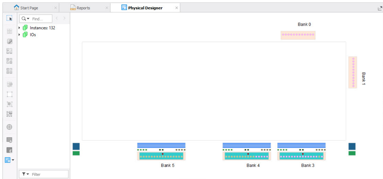
Figure 70: IO Mode
