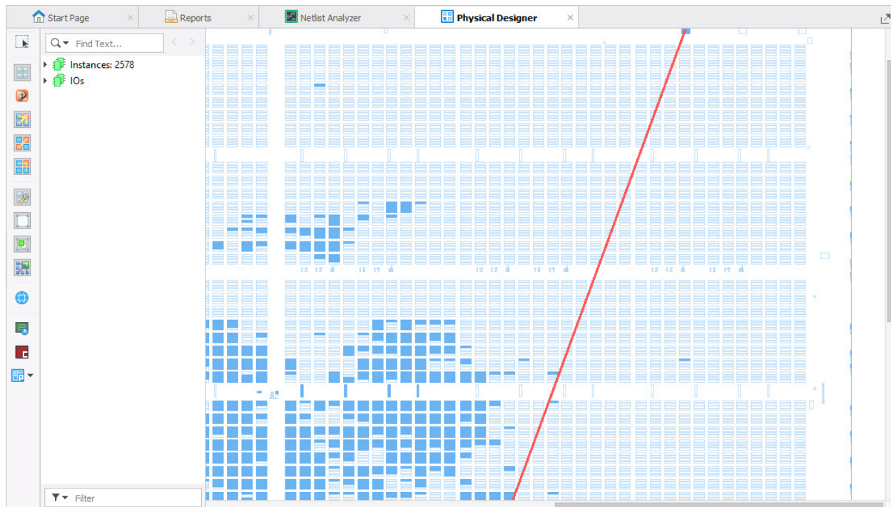
Figure 69: Placement Mode
