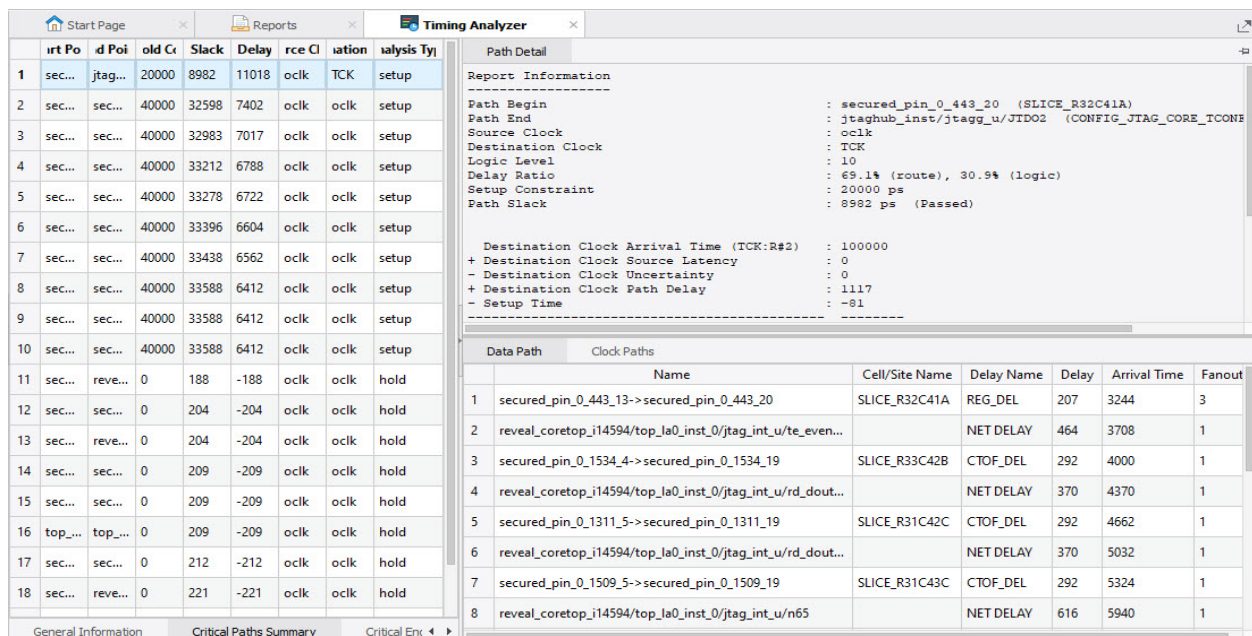
Figure 72: Timing Analyzer
