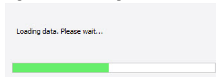
Figure 13: Loading Data
