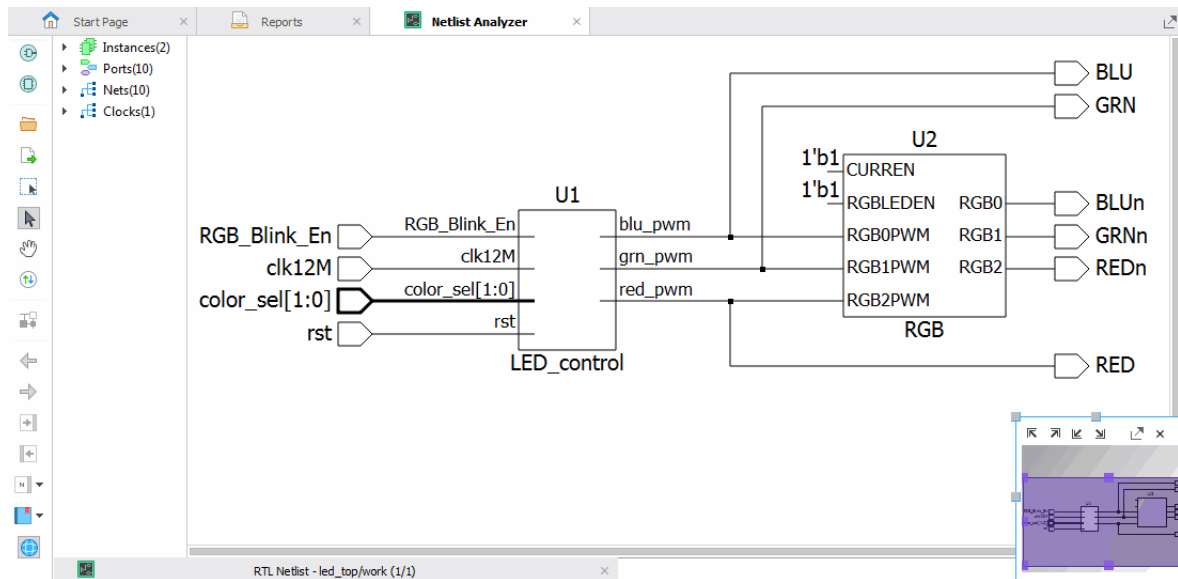
Figure 68: Netlist Analyzer
