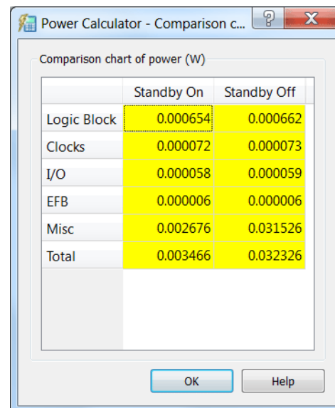
Figure 116: Standby Mode Comparison Chart
