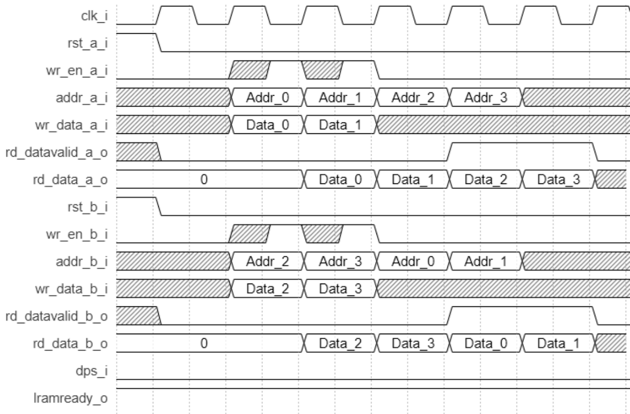
Figure 2.50. True Dual-Port Large RAM Timing Waveform in Write-Through Mode, Without Output Registers
