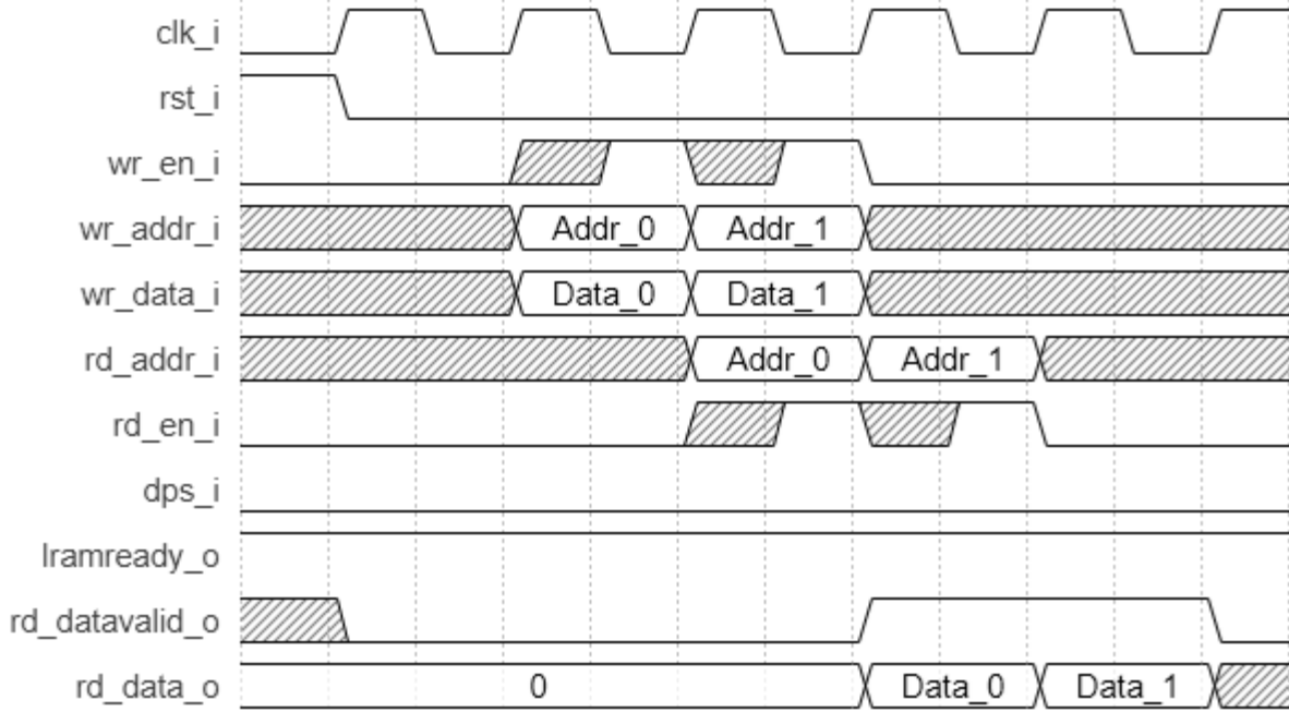
Figure 2.45. PSEUDO DUAL PORT Large RAM Timing Diagram, Without Output Registers
