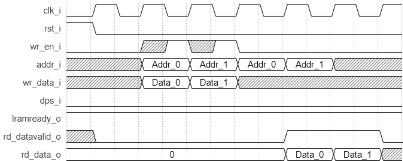
Figure 2.40. Single Port Large RAM Timing Waveform in NORMAL Mode, Without Output Registers
