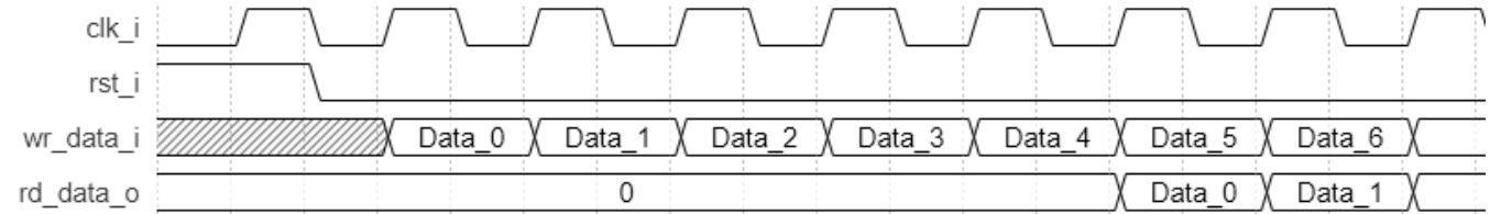
Figure 2.38. Shift Register Without Output Register (LUT Memory, iCE40 UltraPlus)
