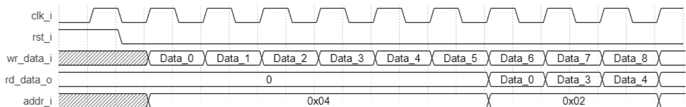
Figure 2.36. Shift Register Variable Configuration and Without Output Register
