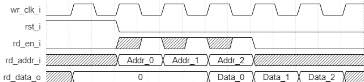
Figure 2.23. Distributed ROM Timing Diagram, With Output Registers and Synchronous Reset
