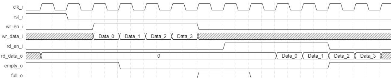
Figure 2.26. FIFO Single Clock With Output Registers and Synchronous Reset
