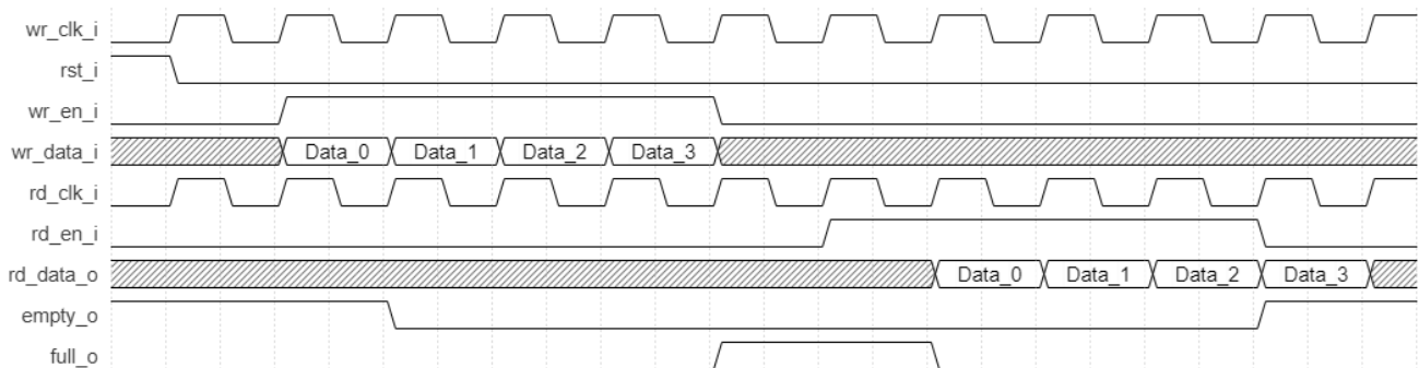
Figure 2.31. Hard Controller FIFO Dual Clock Module Without Output Registers
