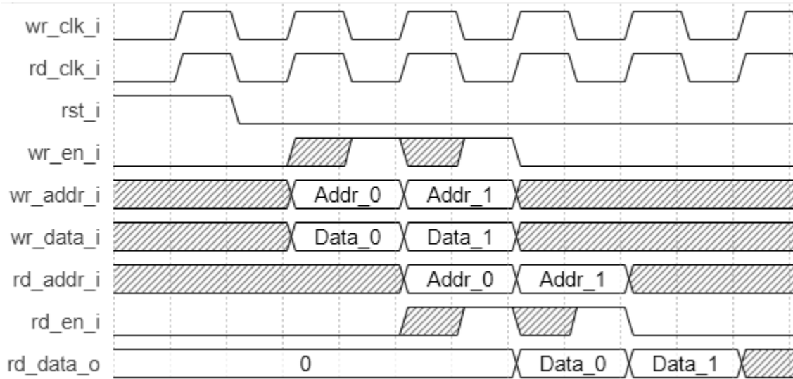
Figure 2.5. PSEUDO DUAL PORT RAM Timing Diagram, Without Output Registers
