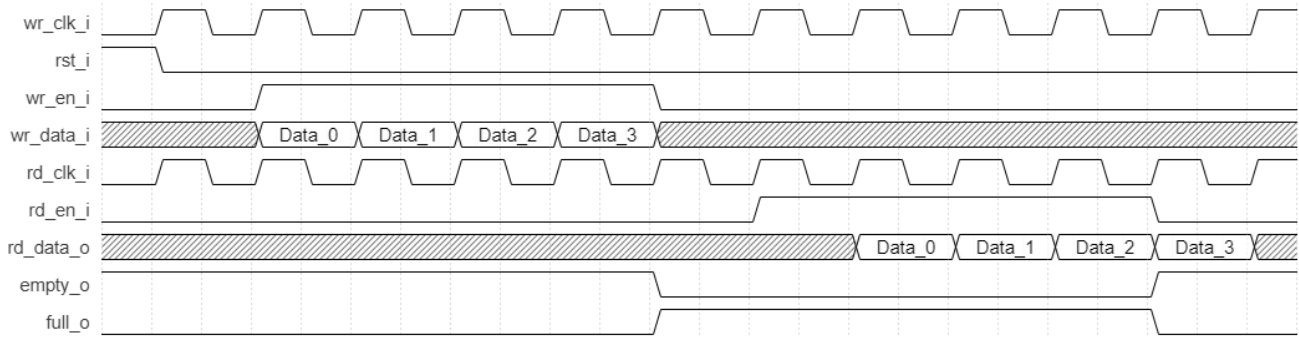
Figure 2.28. FIFO Dual Clock Module Without registers
