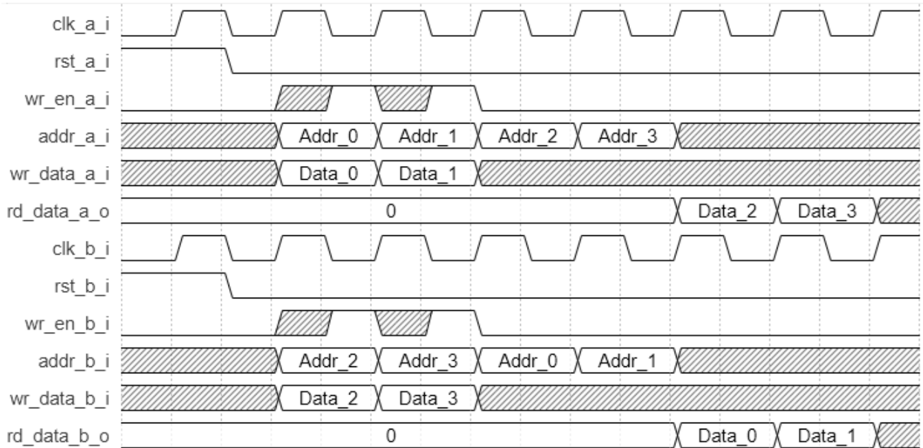
Figure 2.10. TRUE DUAL PORT RAM Timing Diagram, With Output Registers
