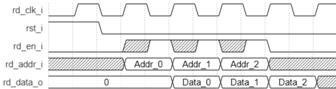
Figure 2.13. ROM Timing Diagram, Without Output Registers
