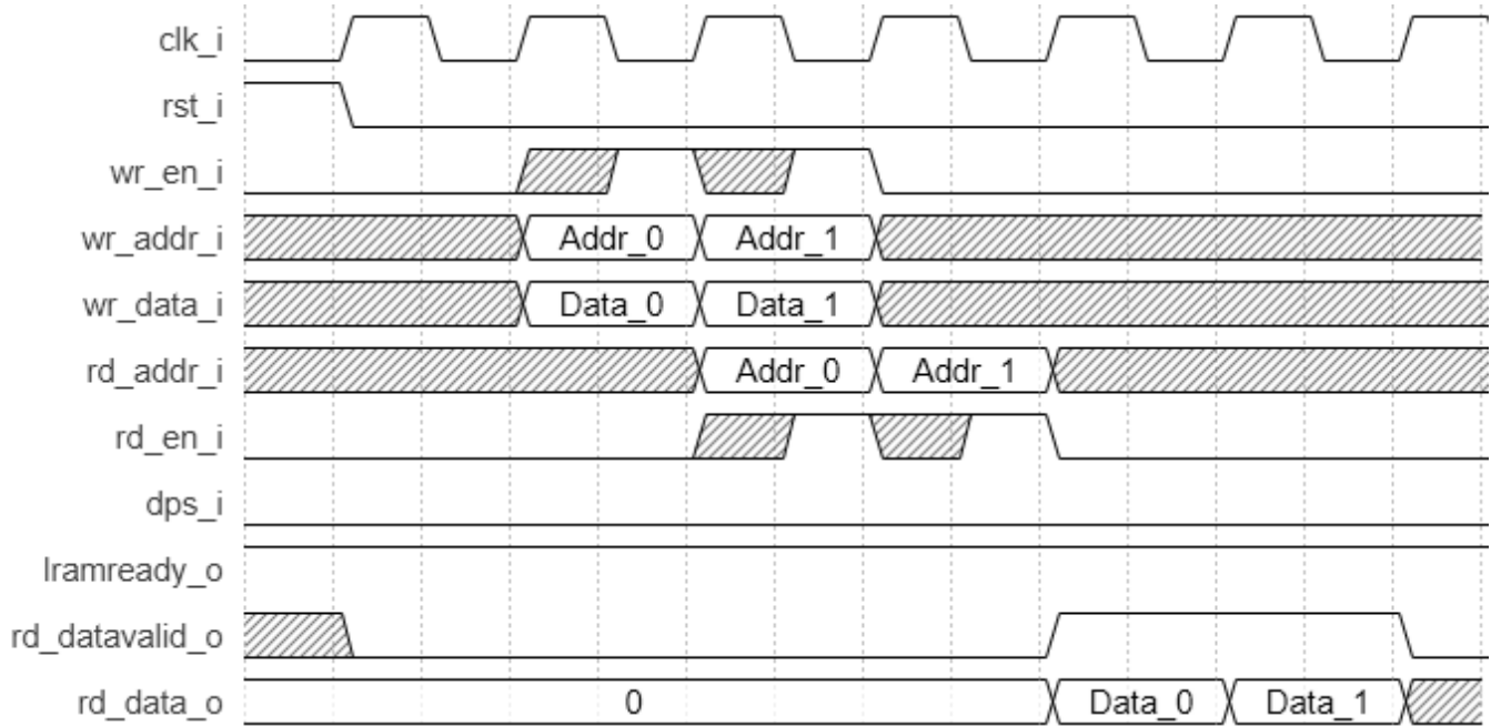
Figure 2.46. PSEUDO DUAL PORT Large RAM Timing Diagram, With Output Registers
