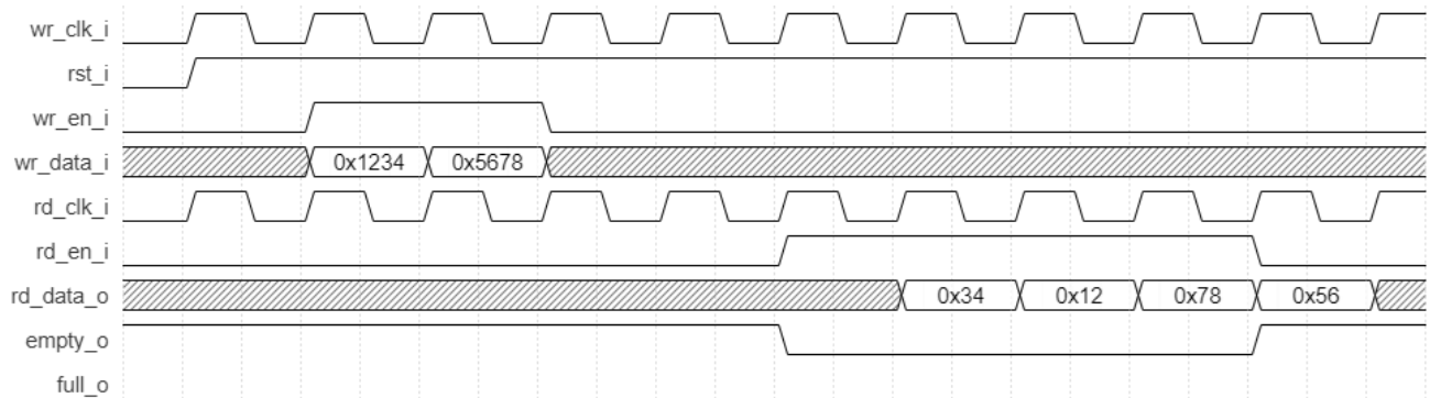
Figure 2.30. FIFO Dual Clock Module, Mixed-Width Without Output Registers
