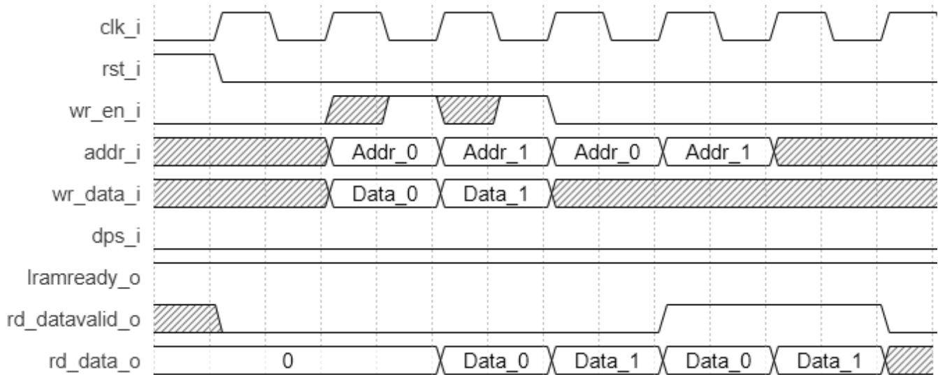
Figure 2.42. Single Port Large RAM Timing Waveform in Write-Through Mode, Without Output Registers
