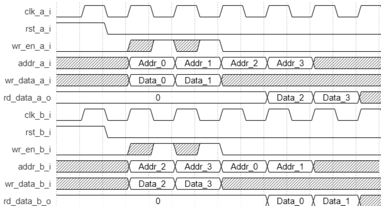
Figure 2.9. TRUE DUAL PORT RAM Timing Diagram, Without Output Registers
