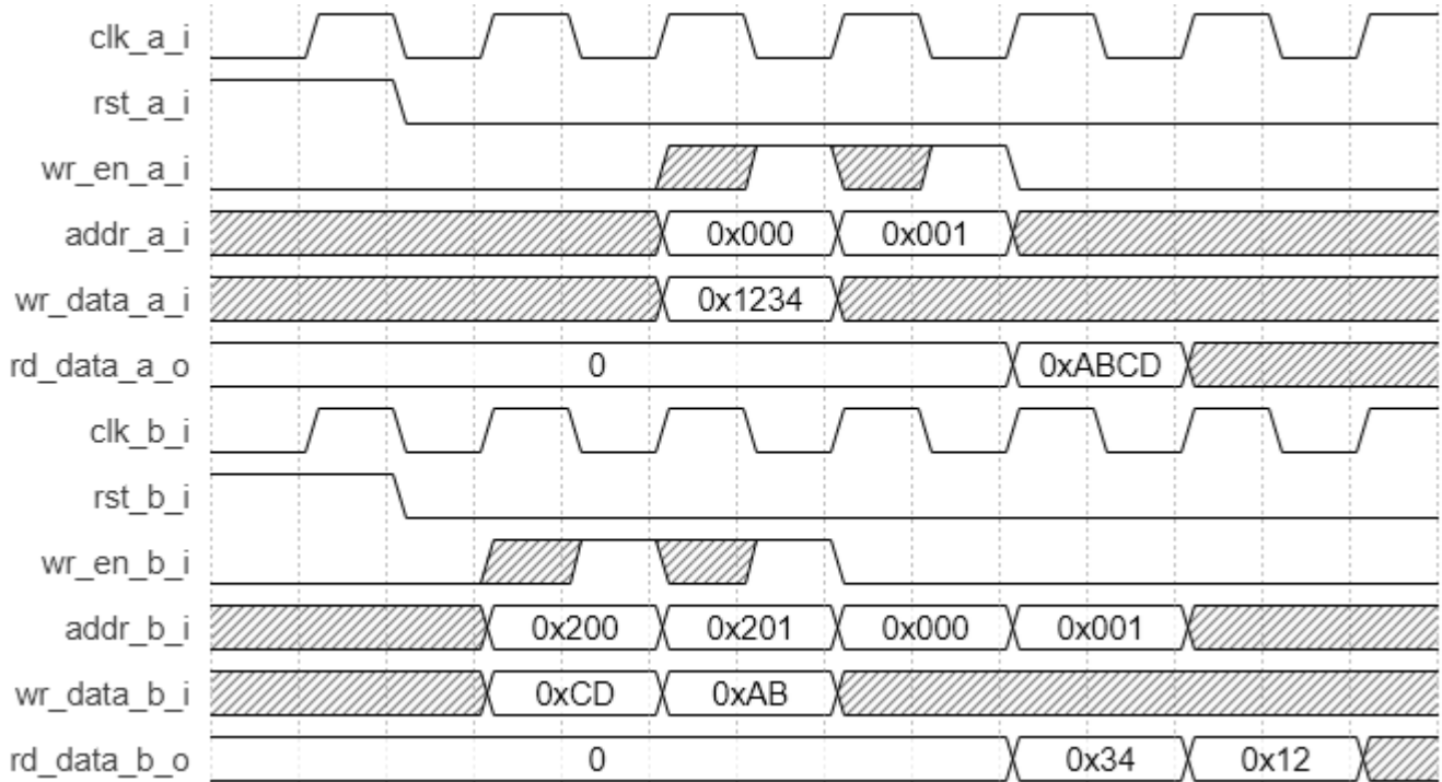
Figure 2.11. TRUE DUAL PORT RAM Timing Diagram, Mixed Width Without Output Registers
