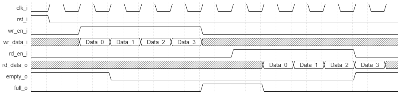
Figure 2.25. FIFO Single Clock Without Output Registers
