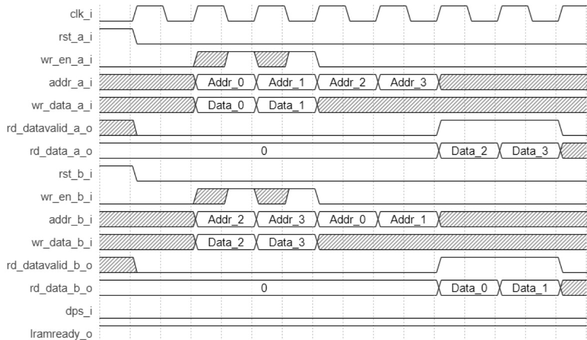
Figure 2.49. True Dual-Port Large RAM Timing Waveform in NORMAL Mode, With Output Registers
