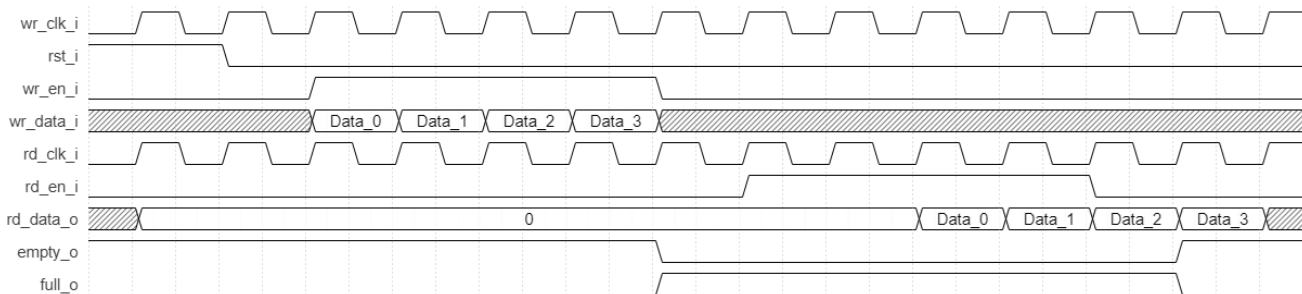
Figure 2.29. FIFO Dual Clock Module With Output Registers and Synchronous Reset
