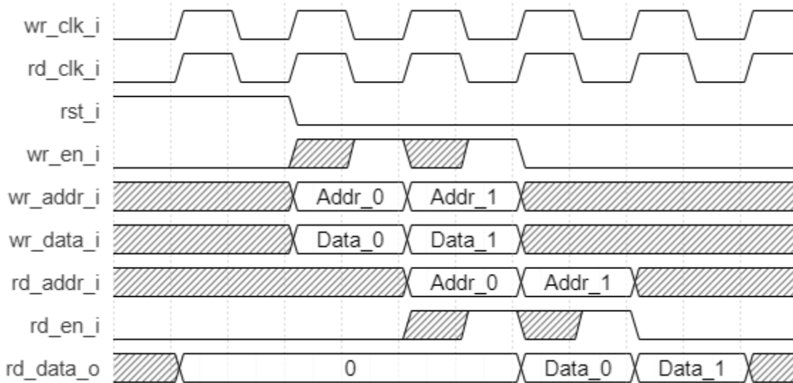
Figure 2.17. Distributed PSEUDO DUAL PORT RAM Timing Diagram, With Output Registers and Synchronous Reset
