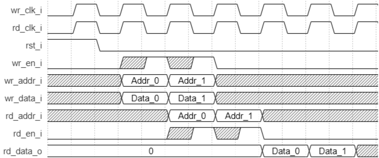
Figure 2.6. PSEUDO DUAL PORT RAM Timing Diagram, With Output Registers
