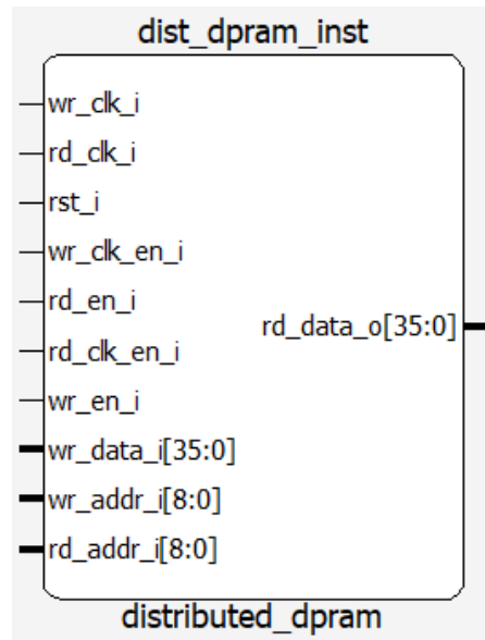
Figure 2.15. Distributed Pseudo Dual Port Module Generated by Module/IP Block Wizard
