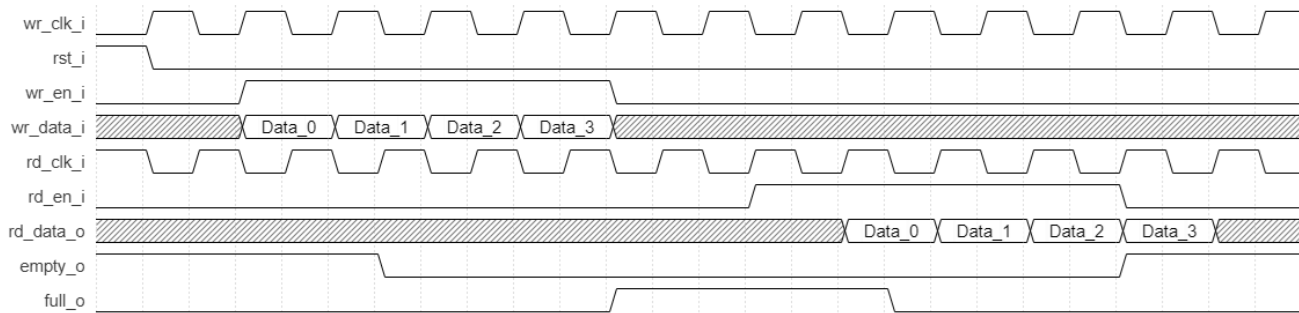
Figure 2.32. Hard Controller FIFO Dual Clock Module Without Output Registers Operating in Asynchronous Clocks
