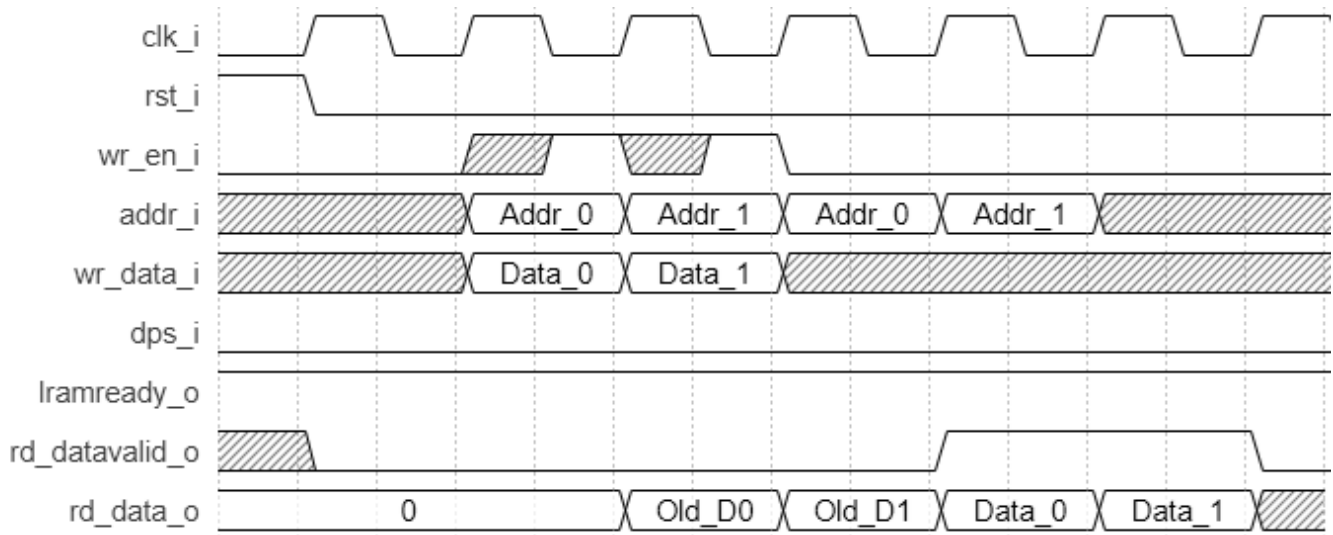
Figure 2.43. Single Port Large RAM Timing Waveform in Read-Before-Write Mode, Without Output Registers
