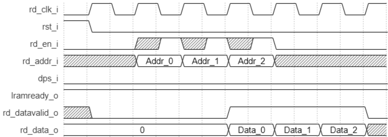
Figure 2.53. Large ROM Timing Diagram, With Output Registers
