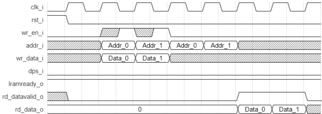
Figure 2.41. Single Port Large RAM Timing Waveform in NORMAL Mode, With Output Registers
