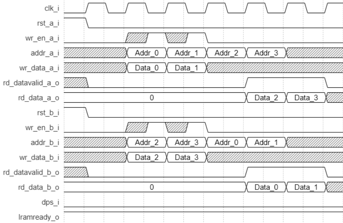
Figure 2.48. True Dual-Port Large RAM Timing Waveform in NORMAL Mode, Without Output Registers
