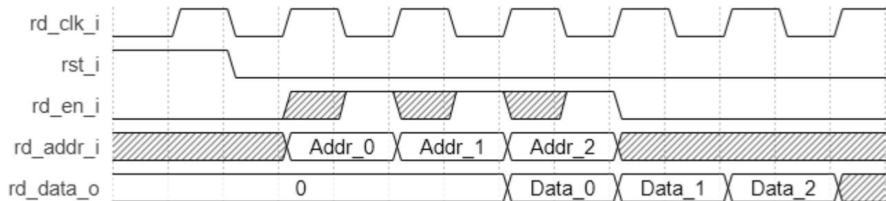
Figure 2.14. ROM Timing Diagram, With Output Registers
