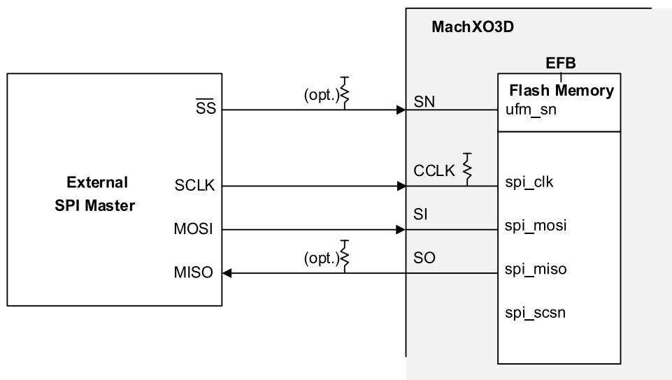
Figure 5.5. External Master SPI Device Accessing the MachXO3D Configuration Logic
