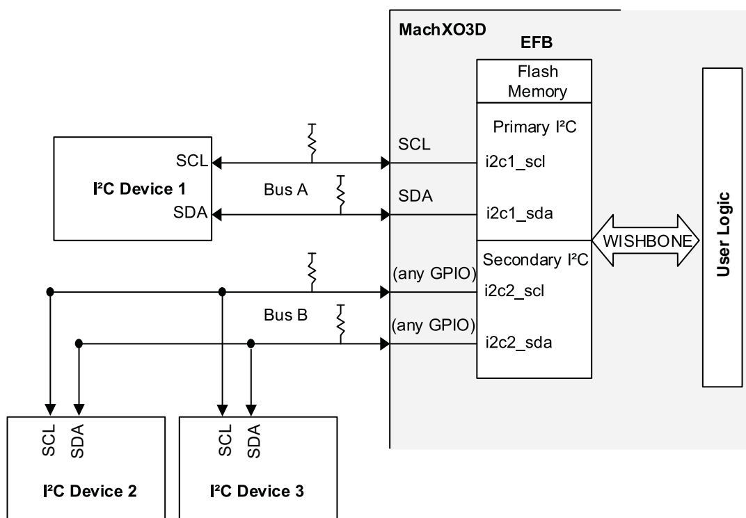
Figure 4.5. I 2 C Circuit
