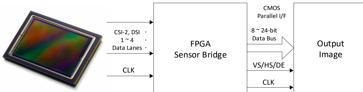
Figure 1.1. CMOS Sensor Bridge Model
