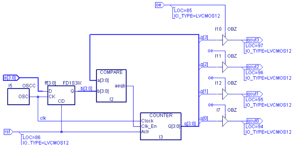
Figure 42: Complex Schematic Sample
