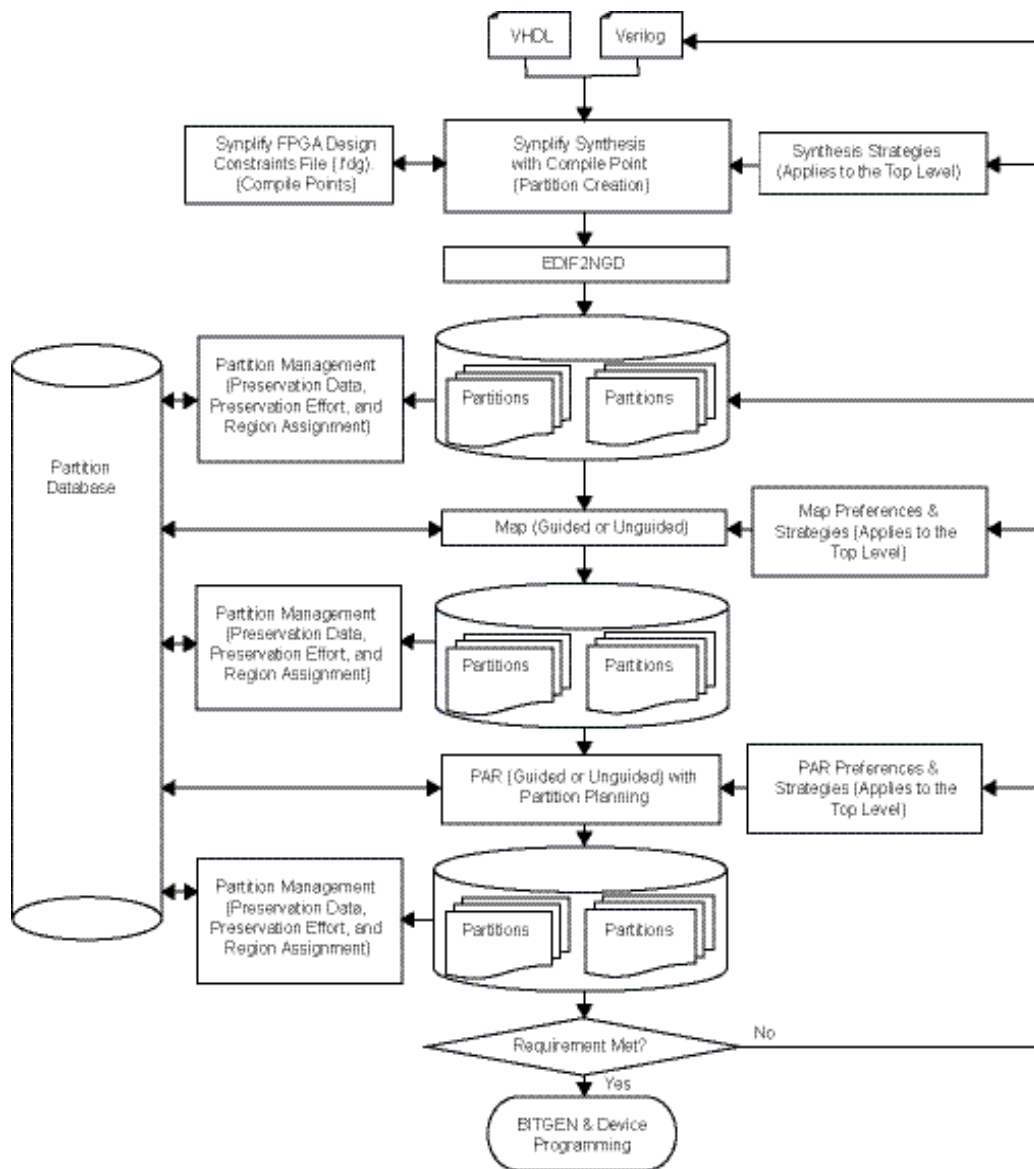
Figure 1: Incremental Design Data Flow
