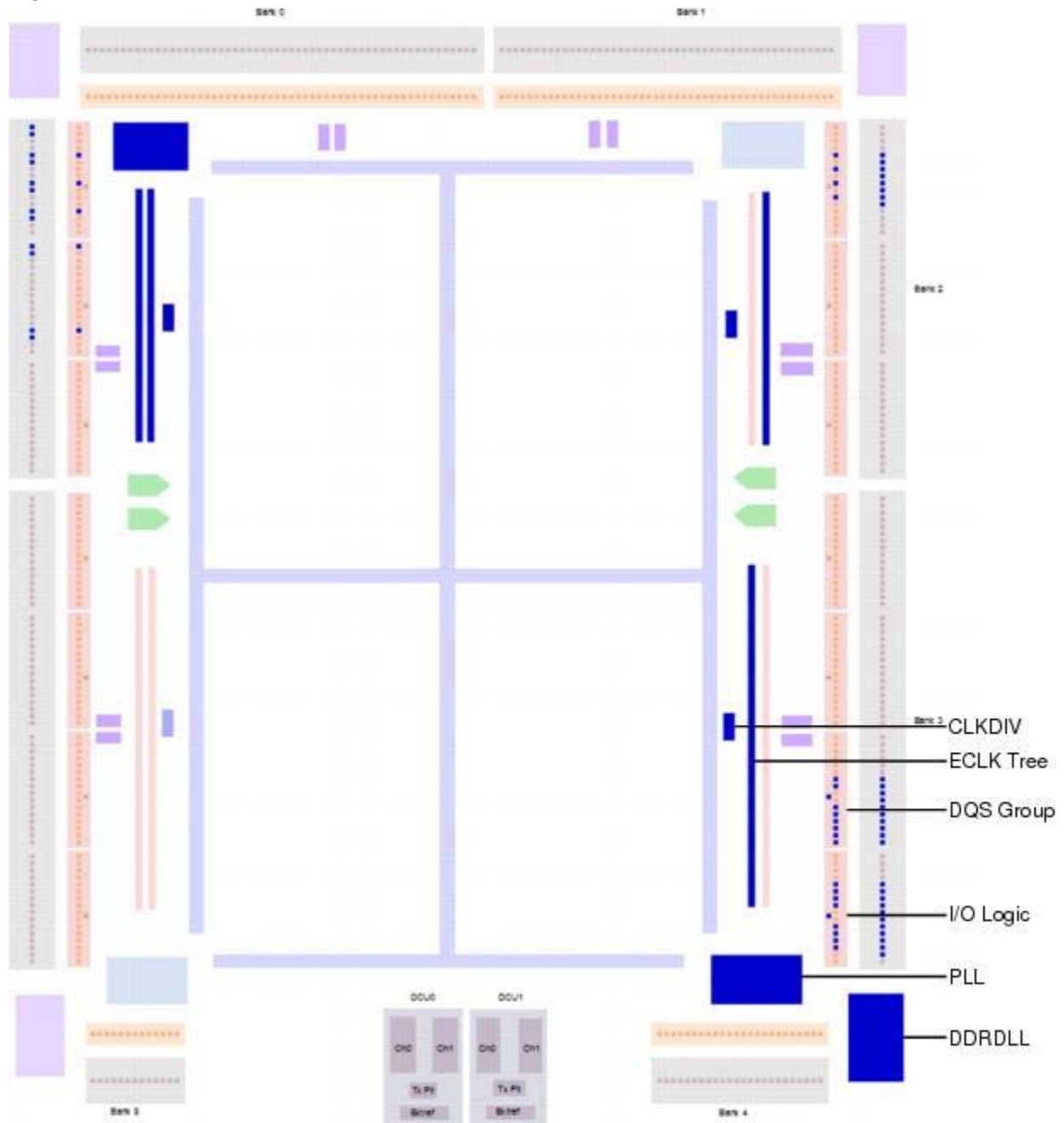
Figure 38: DDR Resources in the Planner View
