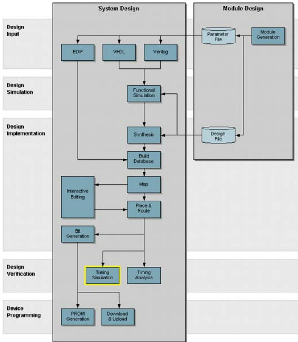
Figure 46: Timing Simulation Flow Chart
