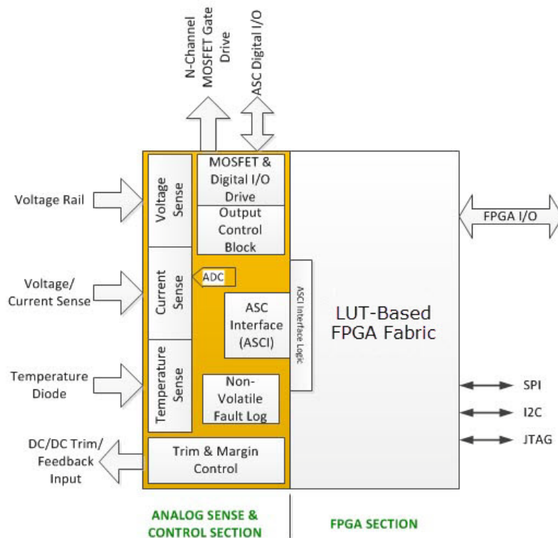
Figure 2: Platform Manager 2 Block Diagram
