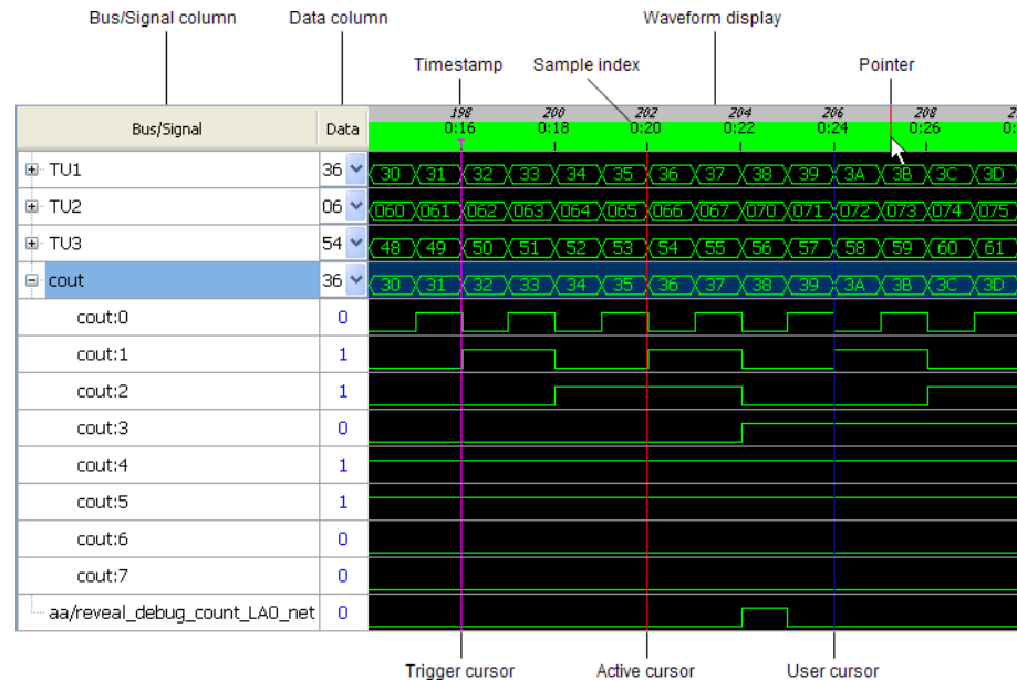
Figure 12: Elements of the LA Waveform View
