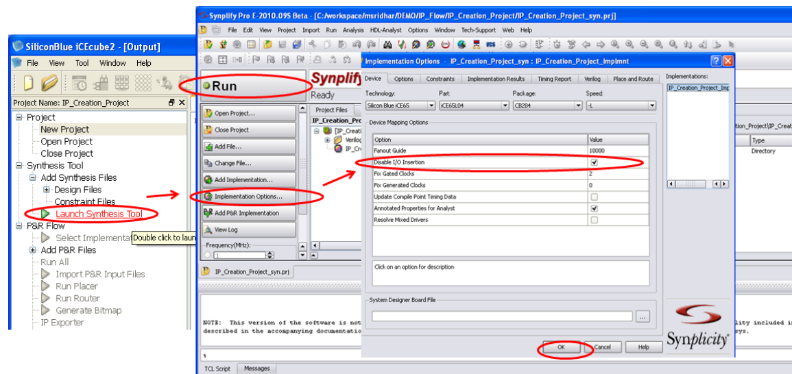
Figure 8-3 Run Synthesis
