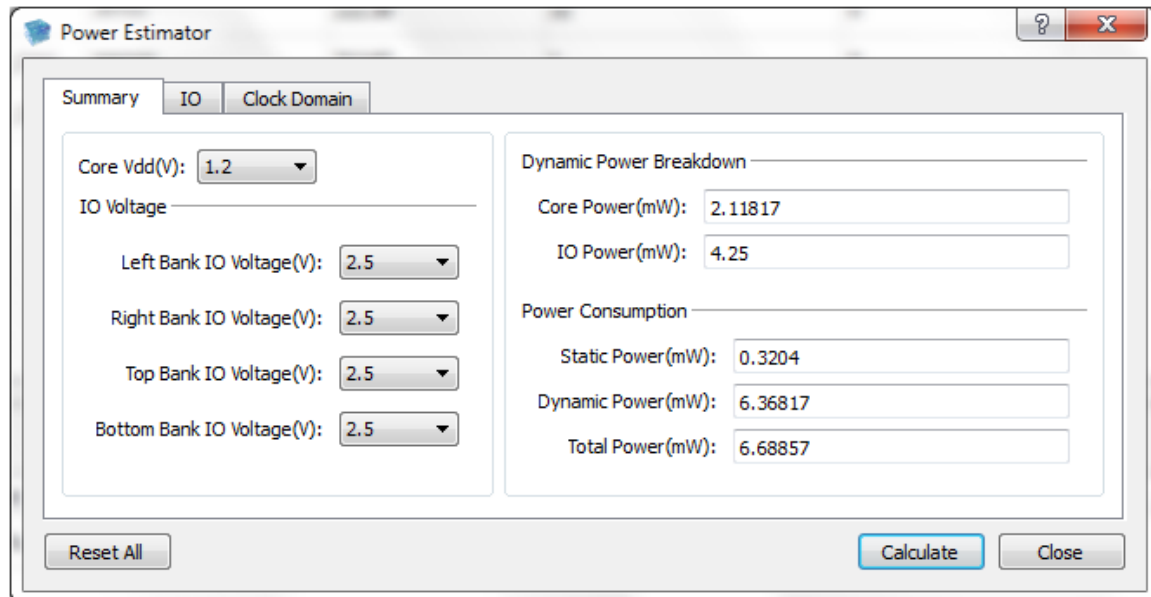
Figure 2-19: Power Estimator
