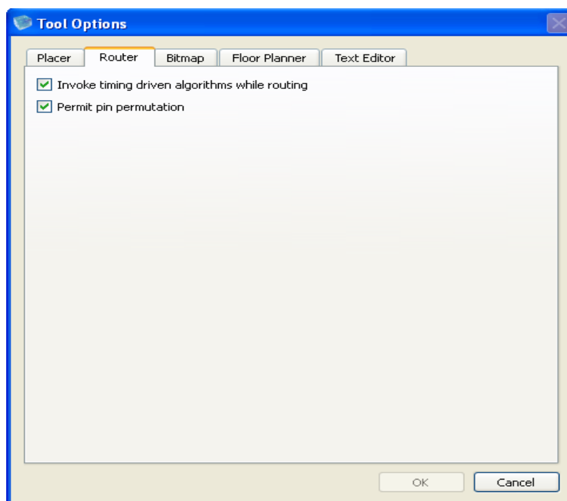
Figure 5-2 : Router Options
