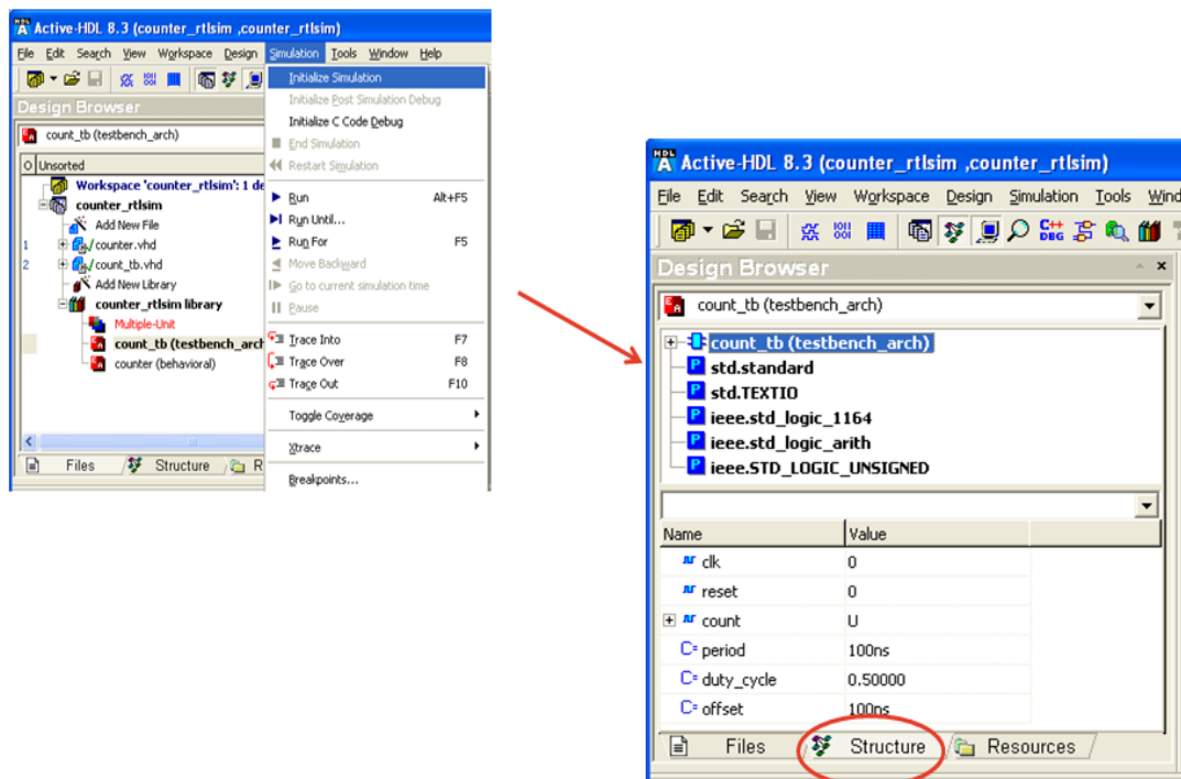
Figure 10-11 : Initialize Simulation.
