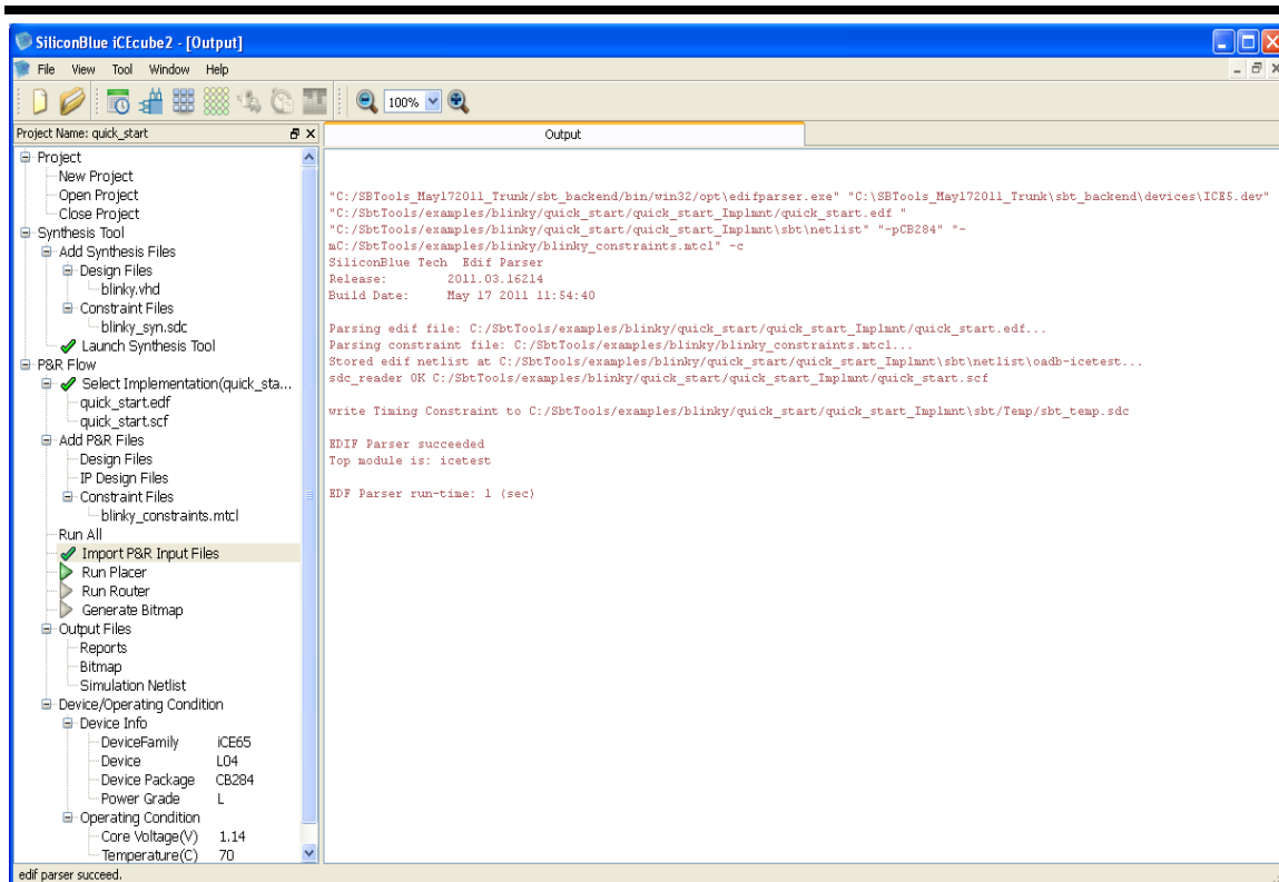
Figure 2-29: Successful Import of P & R Input Files
