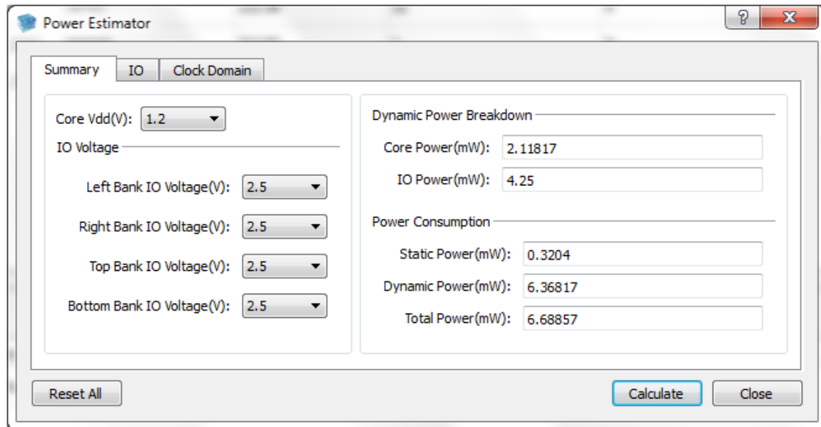
Figure 2-19: Power Estimator
