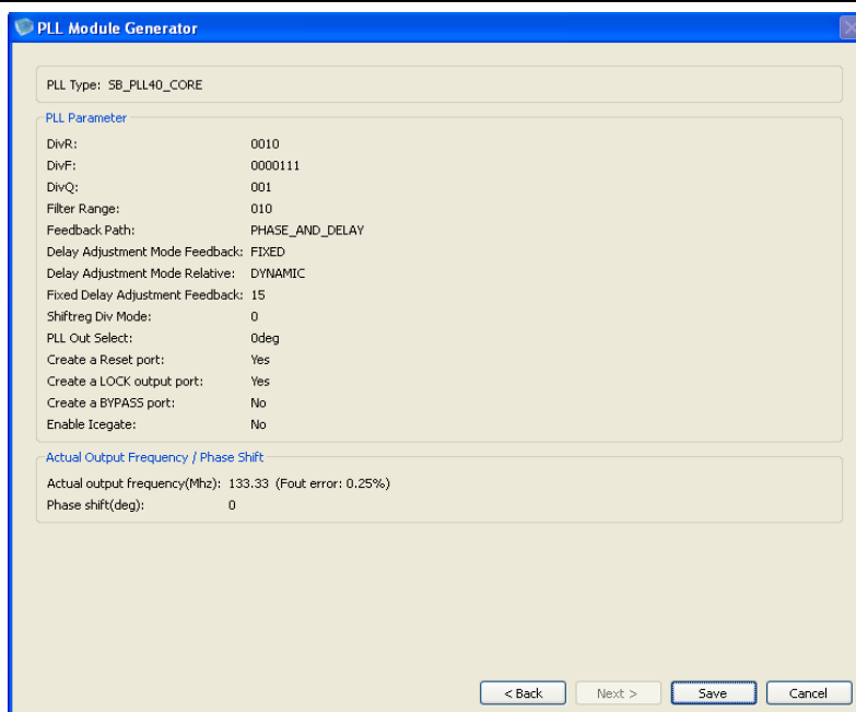
Figure 3-21 : PLL Summary
