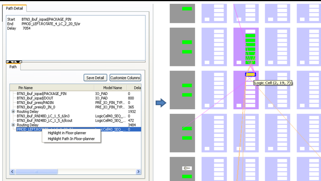
Figure 6-27: Pin Corss Probing between the Timer and Floor Planner
