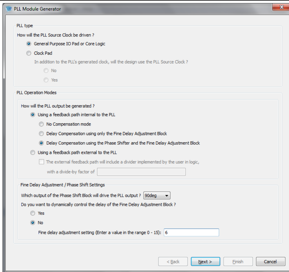
Figure 3-15: Selecting the PLL Type and Operation Mode
