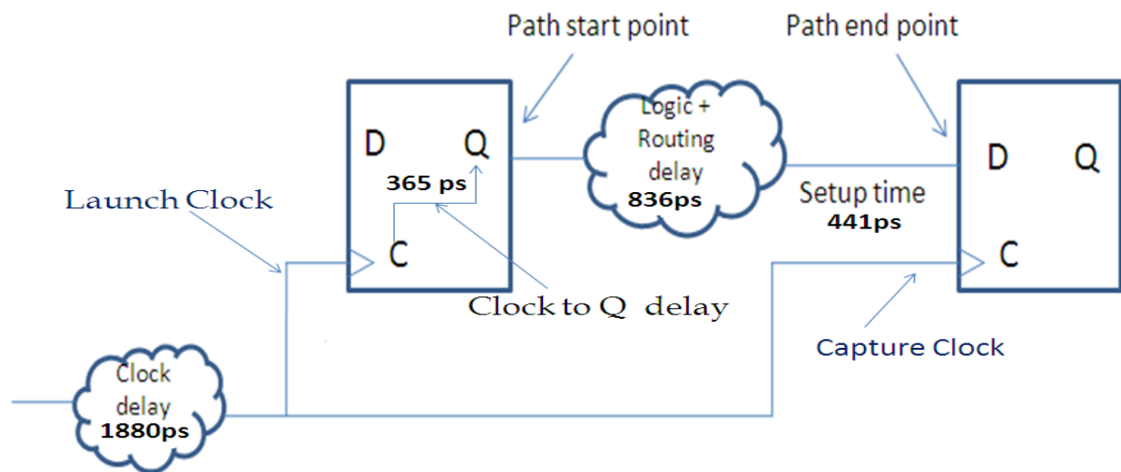
Figure 6-29: Flop to Flop Path
