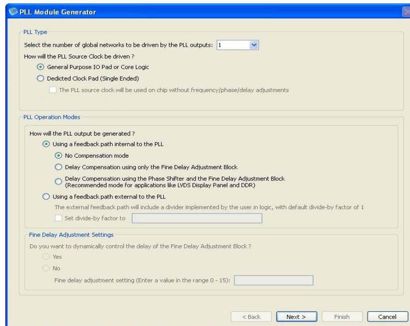
Figure 3-18: iCE40 PLL - Selecting PLL Type and Operation Modes
