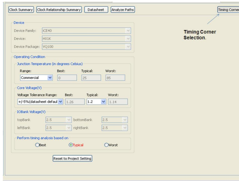
Figure 6-26: Changing the Timing Corner in the Timing Viewer
