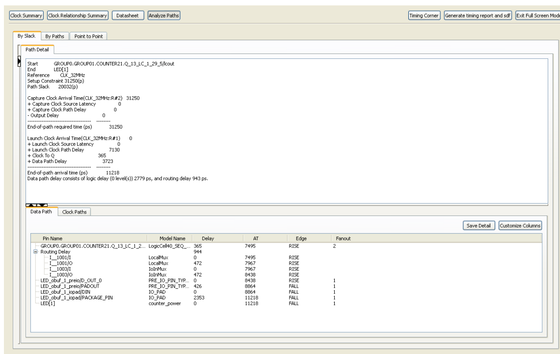
Figure 6-21: Detailed Path Report of the Selected Path
