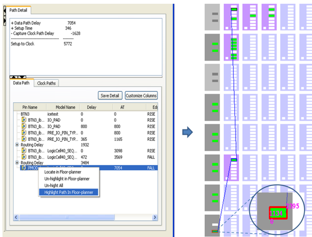
Figure 6-28: Path Cross Probing between the Timer and Floor Planner
