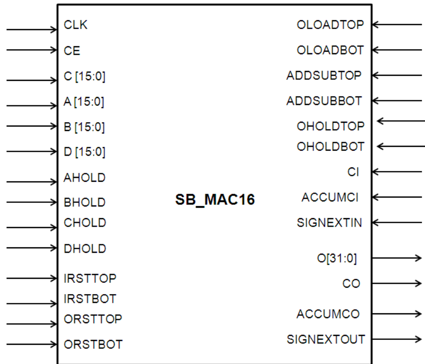
SB_MAC16 Interface Diagram
