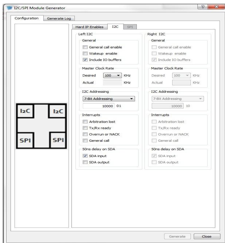
Figure 3-26: Configure Left/Right I2C hard IP.
