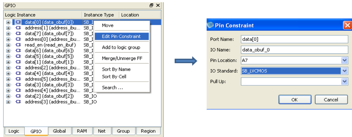
Figure 7-2 Absolute Placement of IOs
