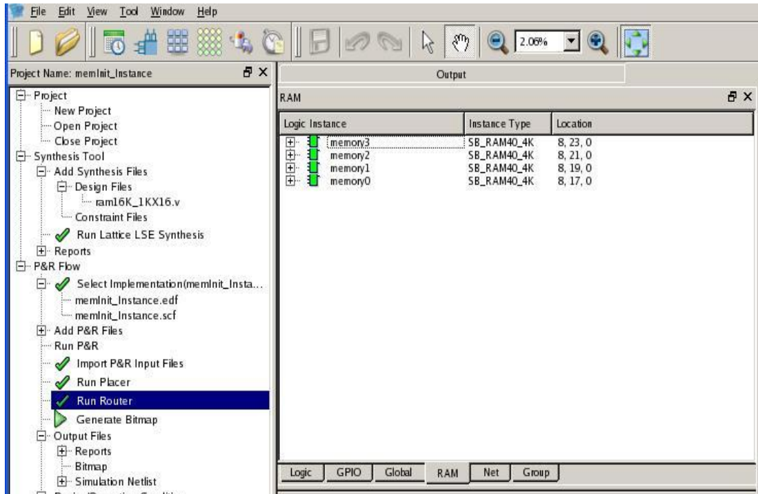
Figure 5-25 : Floorplanner view – BRAM logical instances
