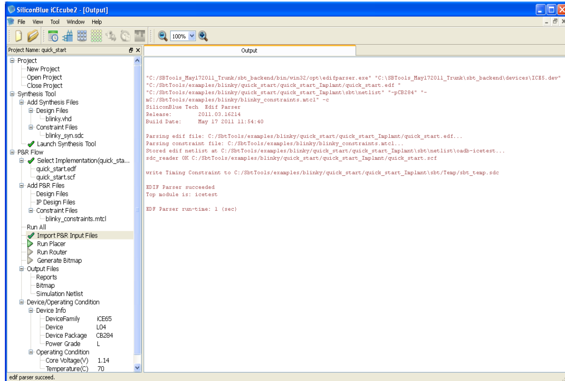
Figure 2-29: Successful Import of P & R Input Files
