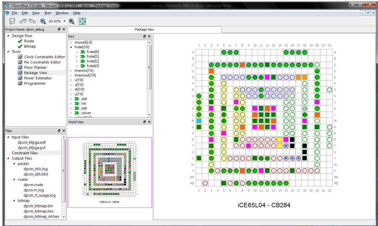
Figure 5-13 : Package View
