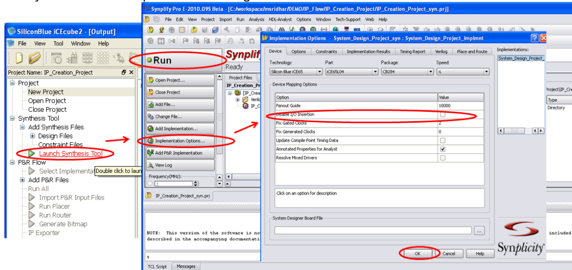
Figure 8-9 Run Synthesis
