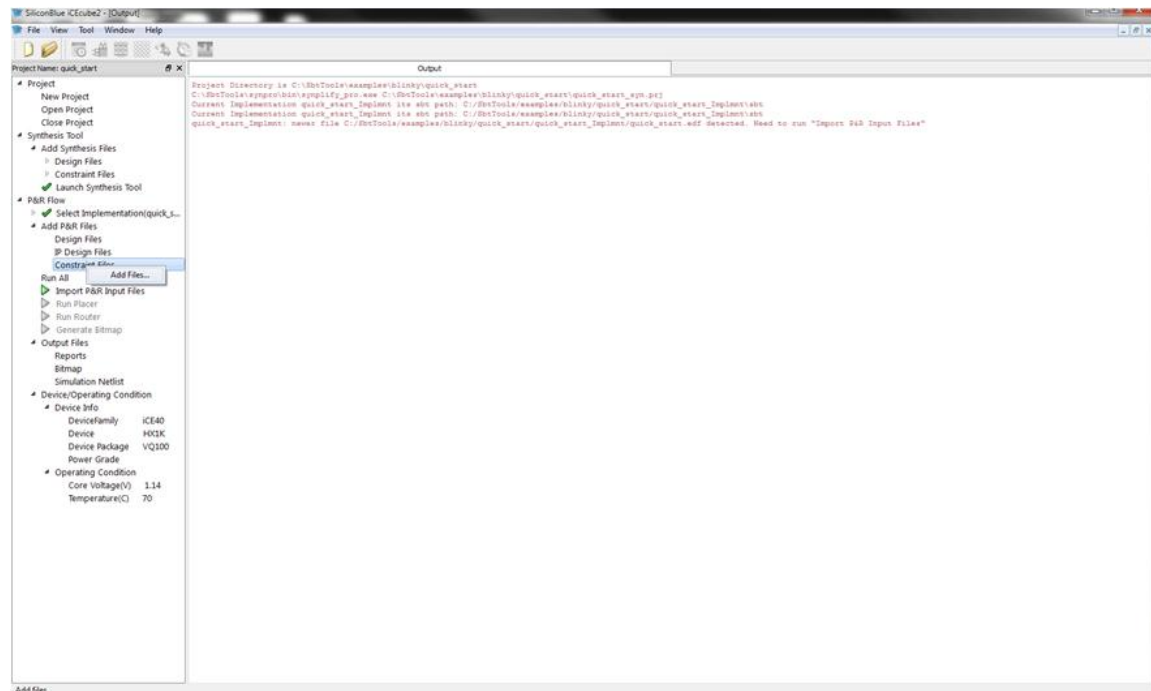
Figure 2-11: Add Constraints Files for Place and Route
