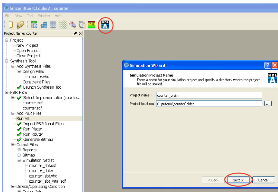
Figure 10-14 : Launch Simulation Wizard and Specify Simulation Project name.
