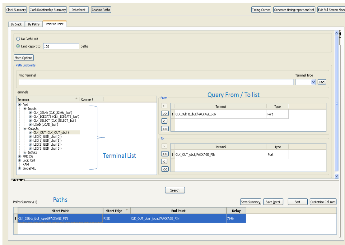
Figure 6-24: Analyzing Point to Point Delays
