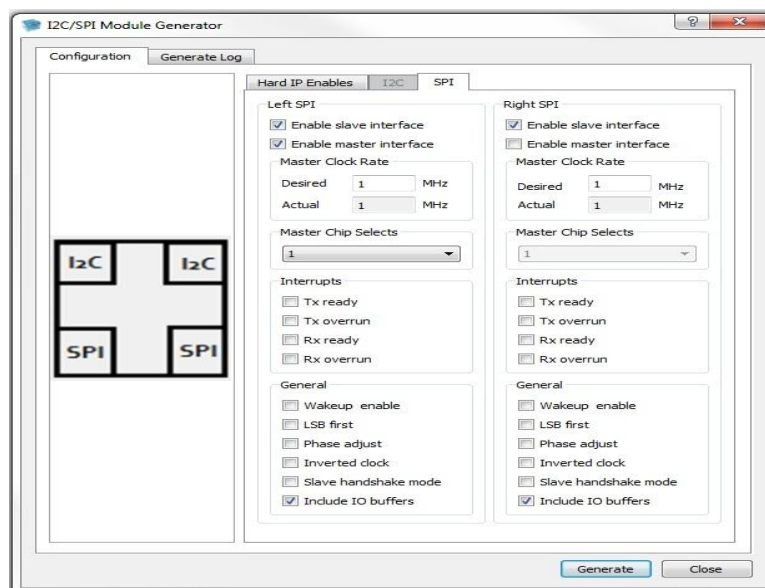
Figure 3-27: Configure Left/Right SPI hard IP.
