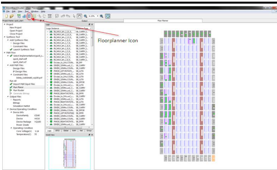
Figure 2-16: Floorplanner View
