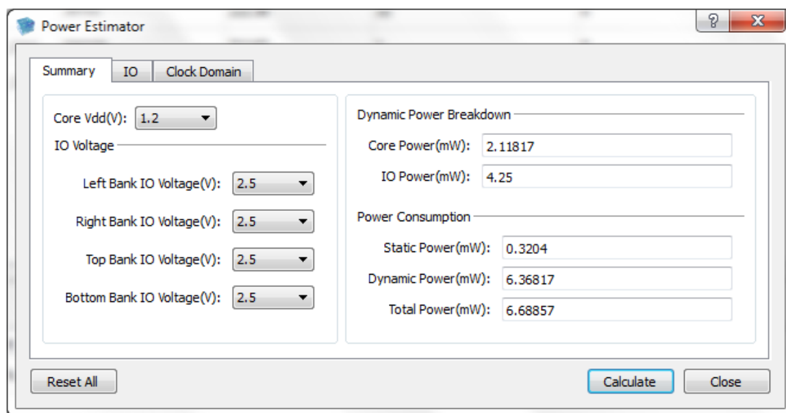
Figure 2-19: Power Estimator
