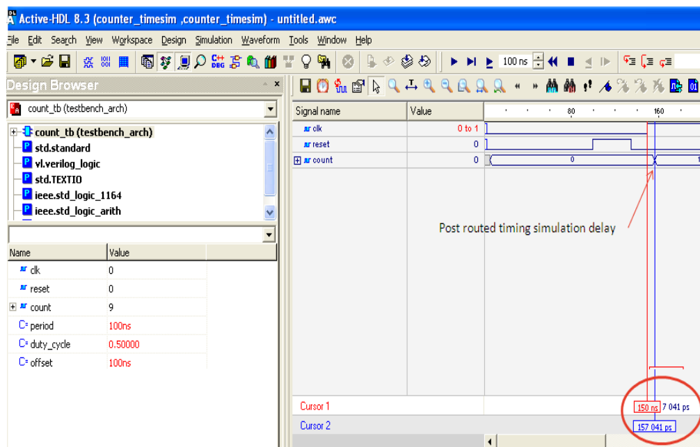
Figure 10-26: Timing Simulation Waveform
