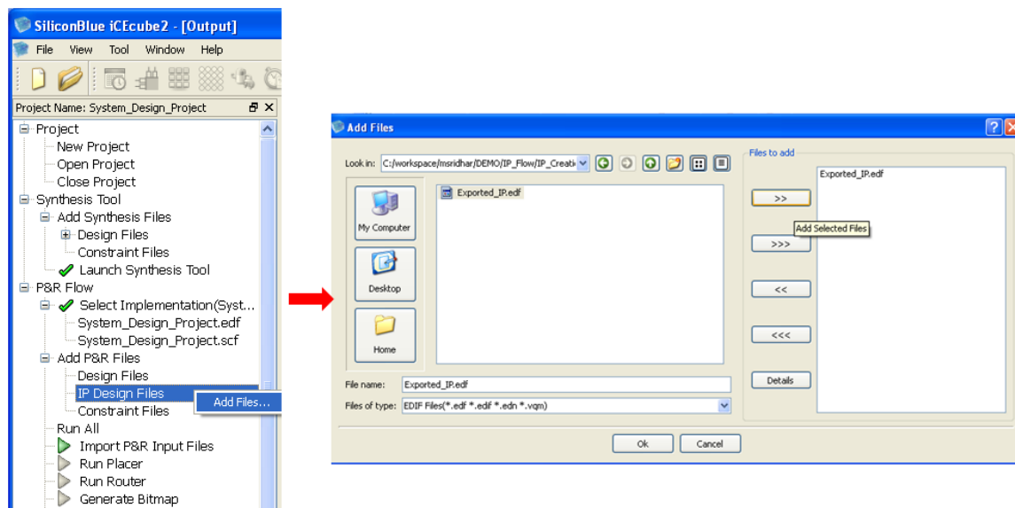
Figure 8-10 Add IP File for performing P&R
