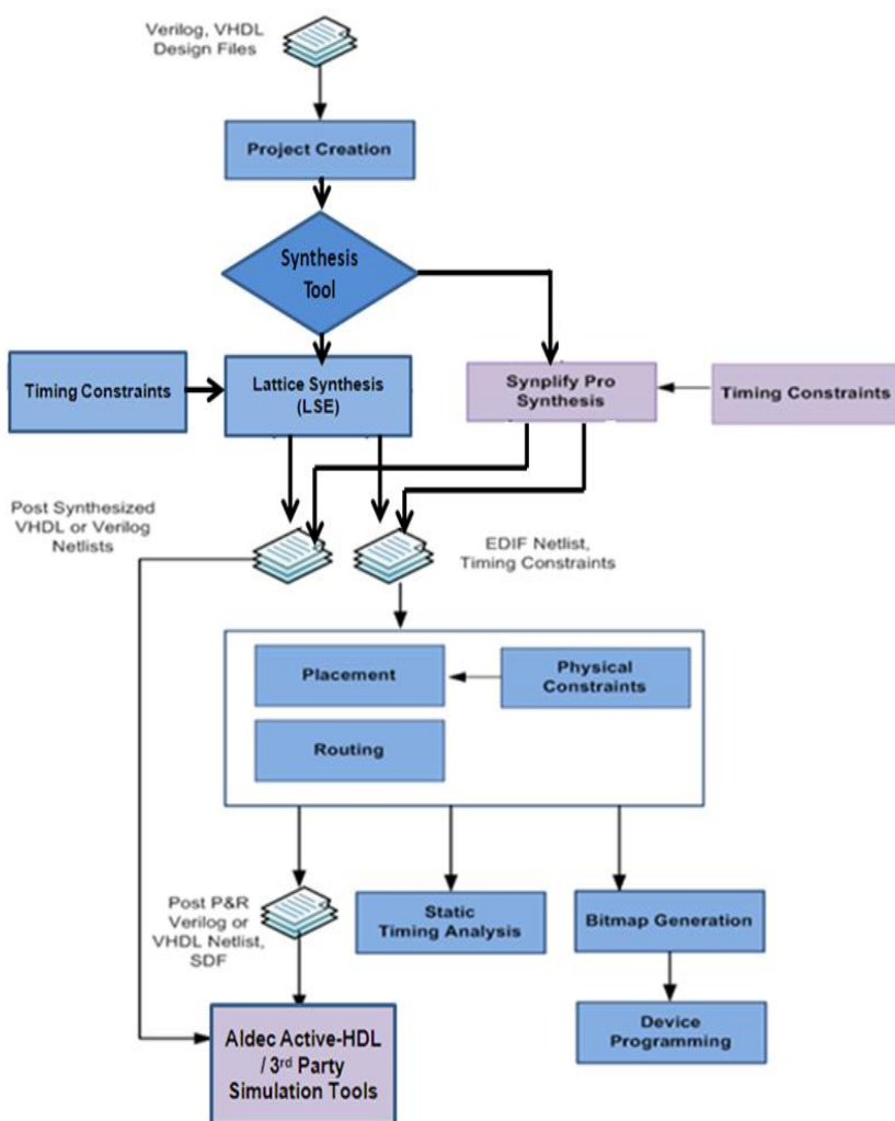
Figure 1-1: The iECube2 Design Flow
