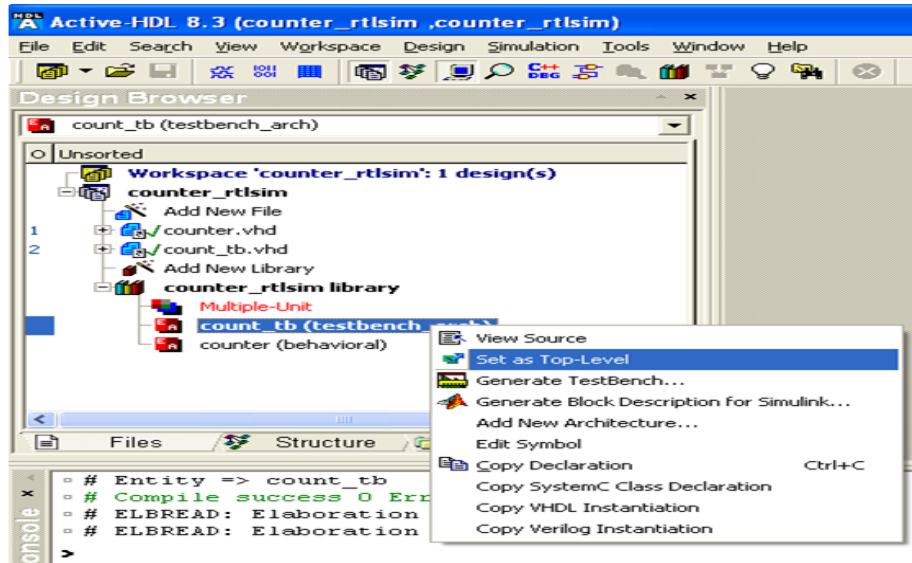
Figure 10-9 : Set Top-Level Entity.
