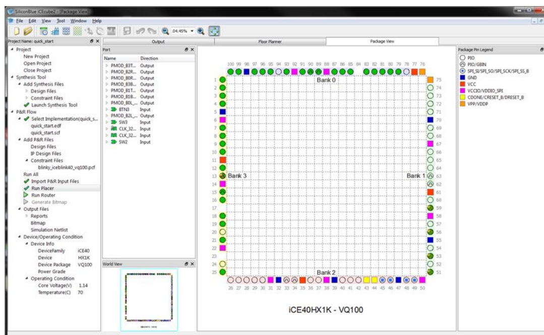
Figure 2-17: Package View
