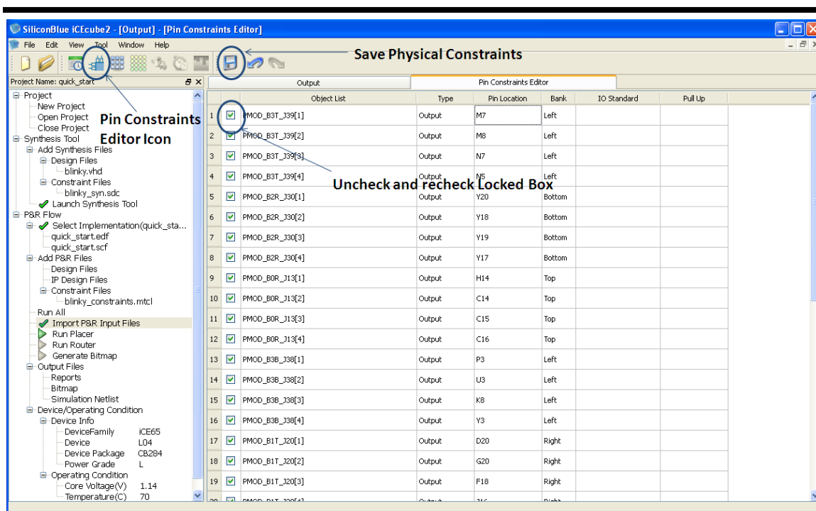
Figure 2-30: Pin Constraints Editor
