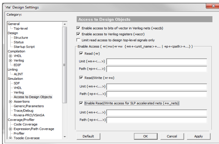
Figure 10-22 : Set Signal Access
