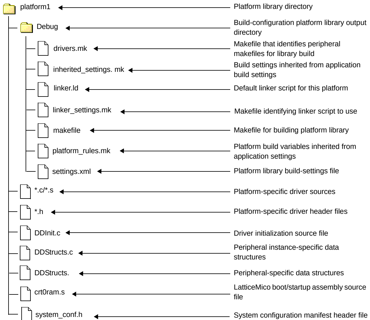
Figure 34: LED_Versal\Platform1 Library Directory Structure
