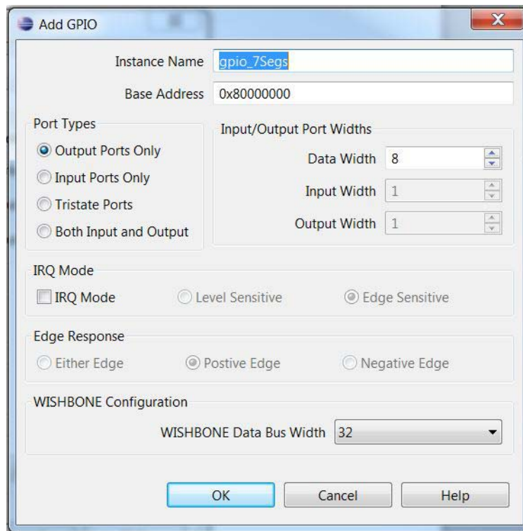
Figure 18: Add GPIO Dialog Box - Second Instance
