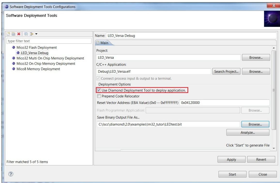
Figure 58: Main Tab of the Software Deployment Tools Configuration Dialog Box with Use Diamond Deployment Tool to Deploy Application Enabled
