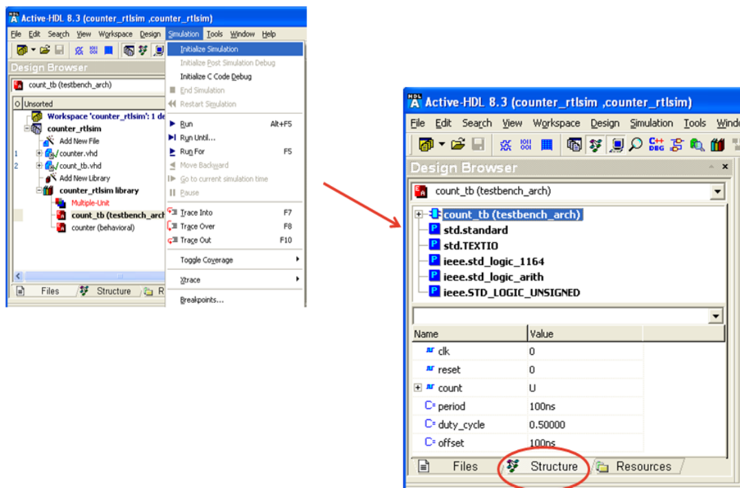
Figure 10-10 : Initialize Simulation.
