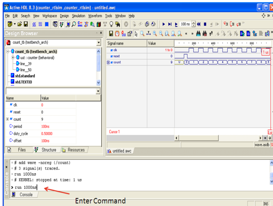
Figure 10-12: View Simulation Results.
