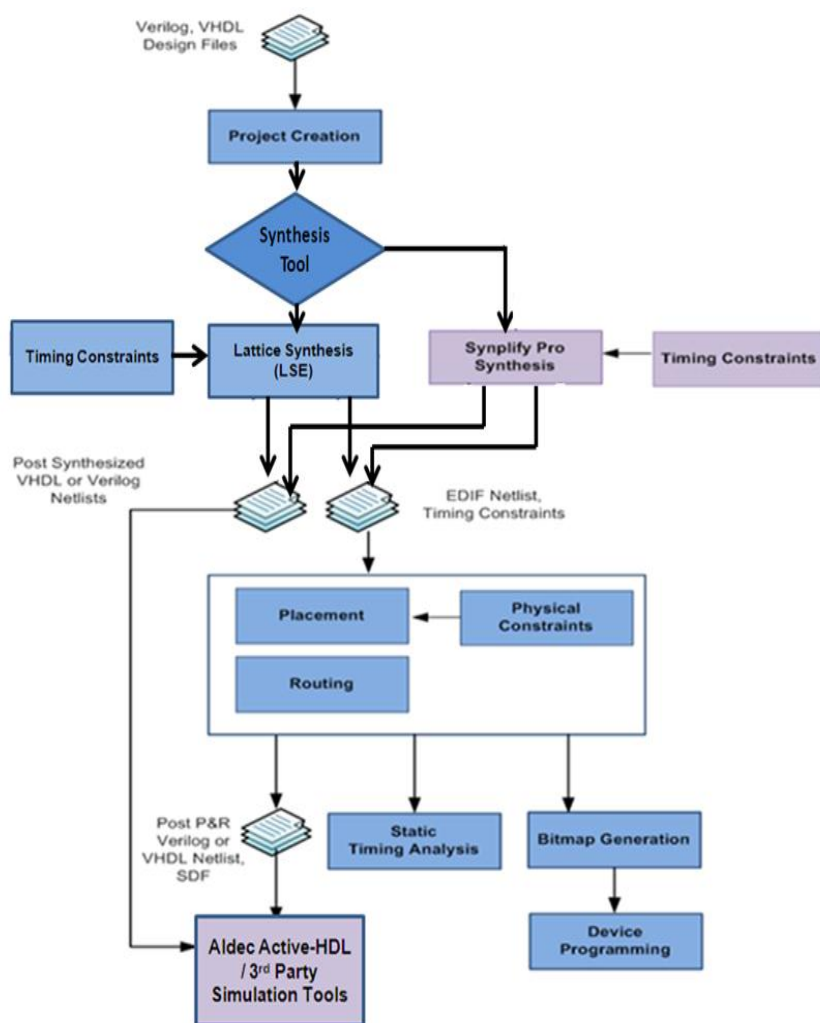
Figure 1-1: The iCEcube2 Design Flow
