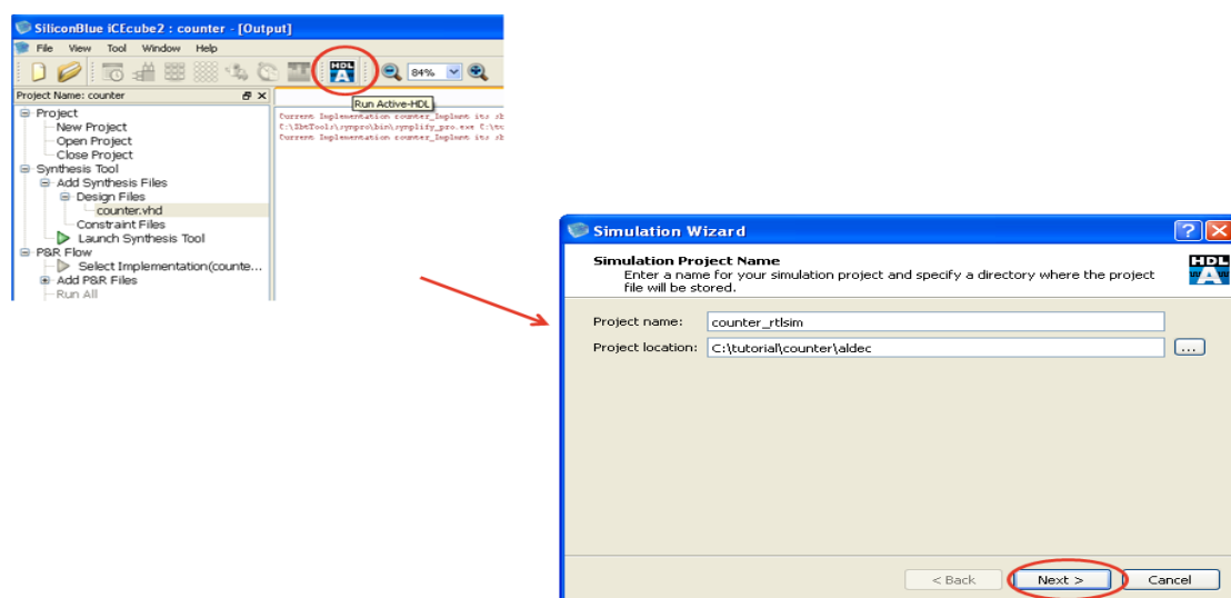
Figure 10-3: Launch Simulation Wizard and Specify Simulation Project name.
