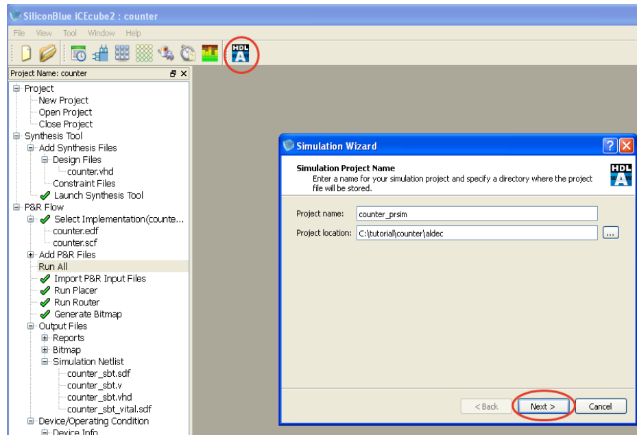
Figure 10-13 : Launch Simulation Wizard and Specify Simulation Project name.
