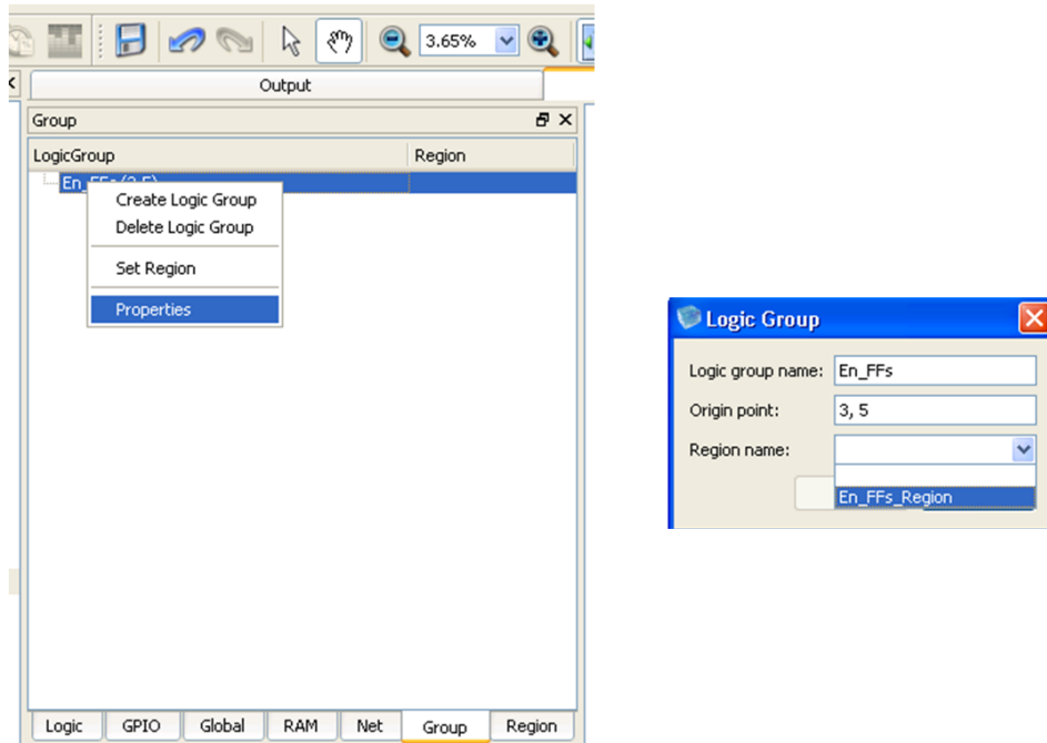
Figure 7-7 Set group to a region
