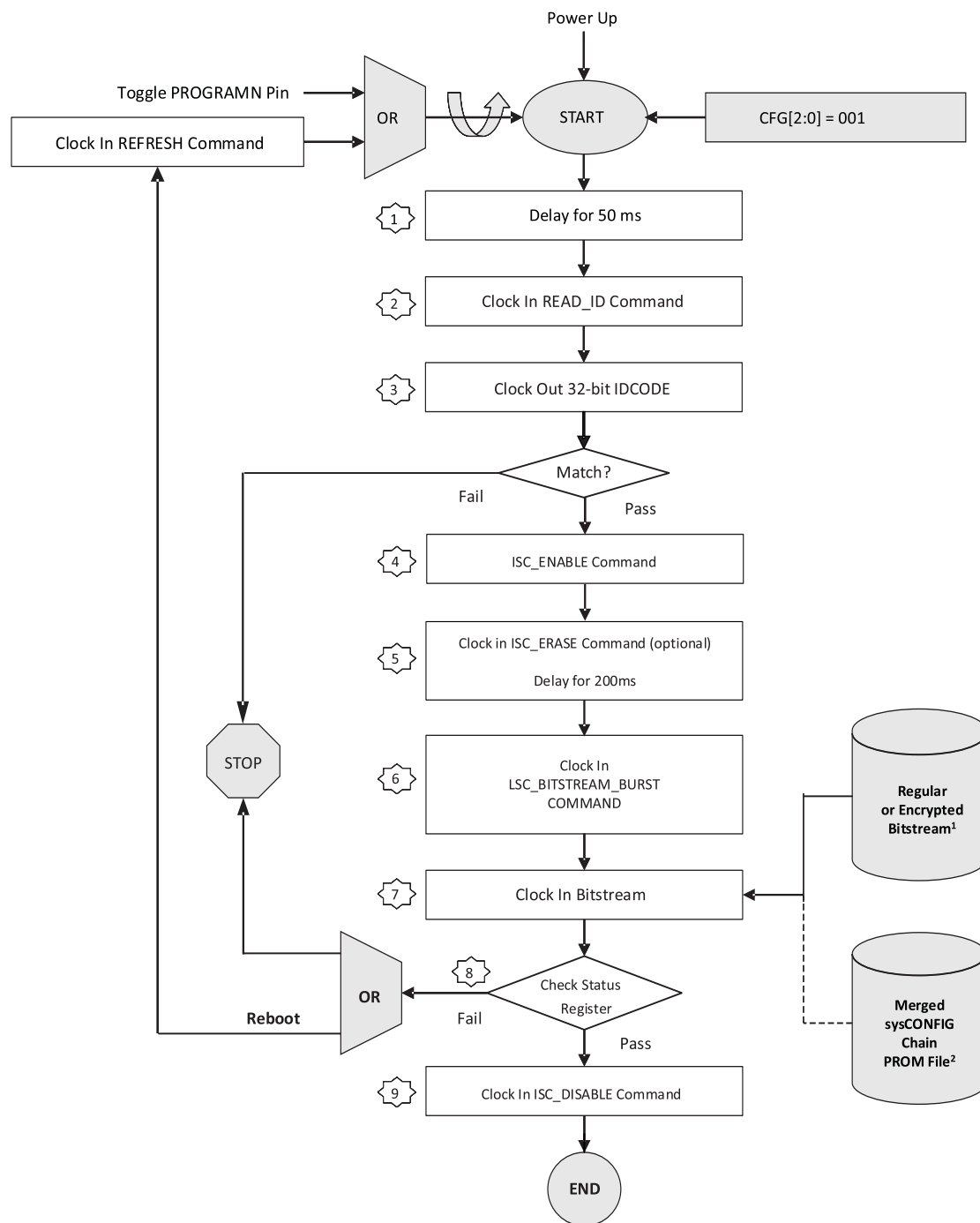
Figure 6.10. Slave SPI Configuration Flow
