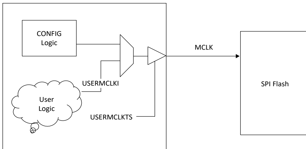
Figure 6.2. MCLK Connection
