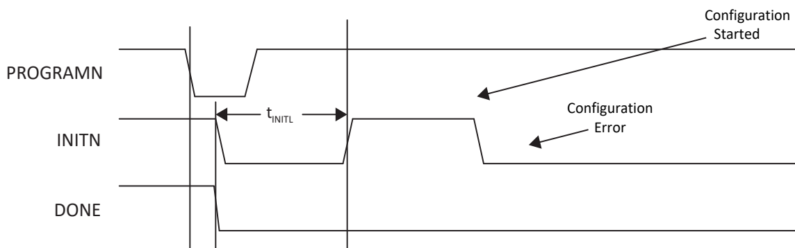
Figure 4.2. Configuration Error Notification
