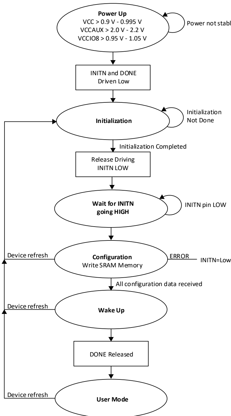
Figure 5.1. Configuration Flow
