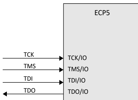
Figure 4.3. JTAG Port
