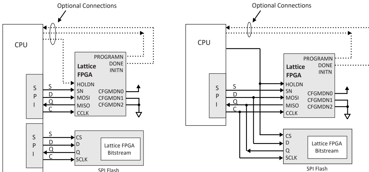
Figure 6.6. ECP5 and ECP5-5G Slave SPI Port with SPI Flash
