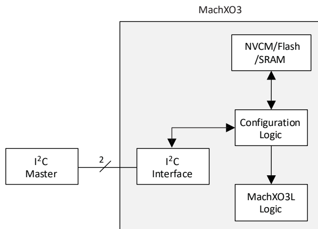
Figure 5.4. I 2 C Configuration Logic
