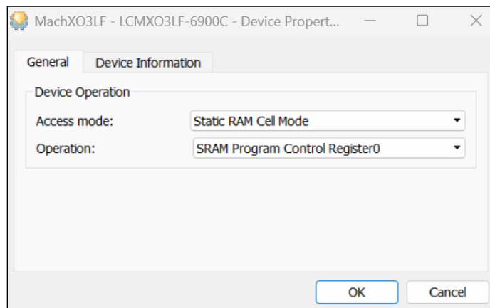
Figure 8.12. Device Properties – SRAM Program Control Register0
