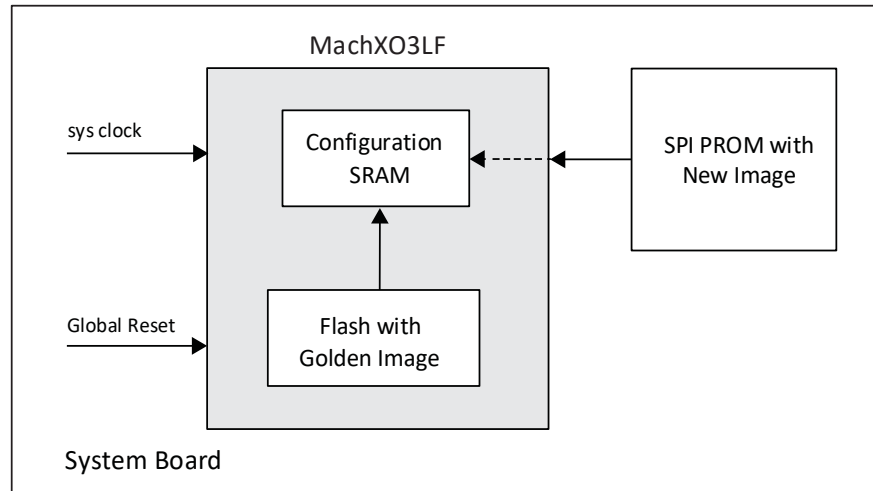
Figure 5.7. Bitstream Update Using TransFR
