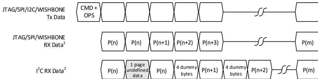
Figure 8.7. Retrieval Delay Timing Requirement for Single-Page Reads
