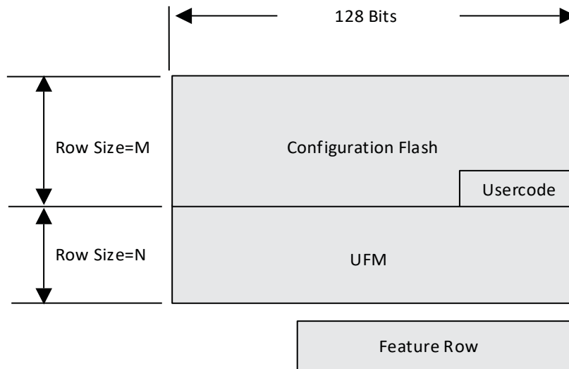
Figure 4.3. Flash Memory Space of a MachXO3LF Device
