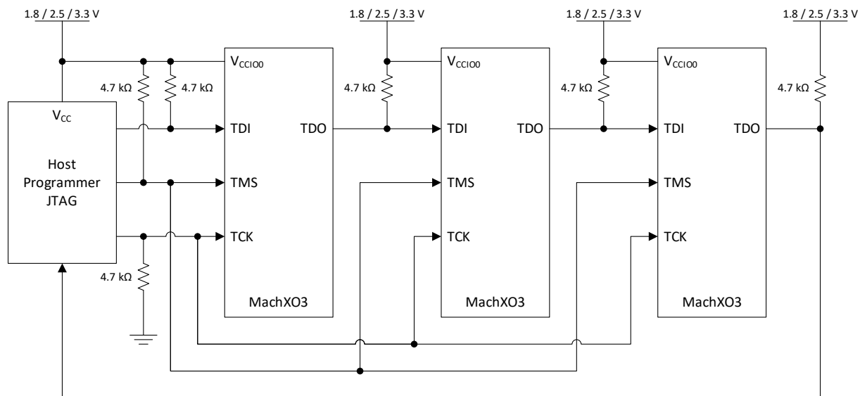
Figure 5.6. JTAG Daisy Chain Example
