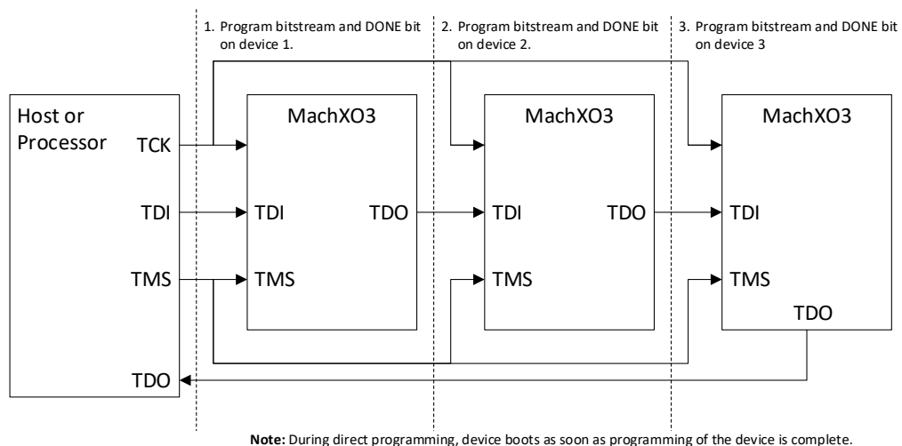
Figure 8.16. Sequential Mode Programming
