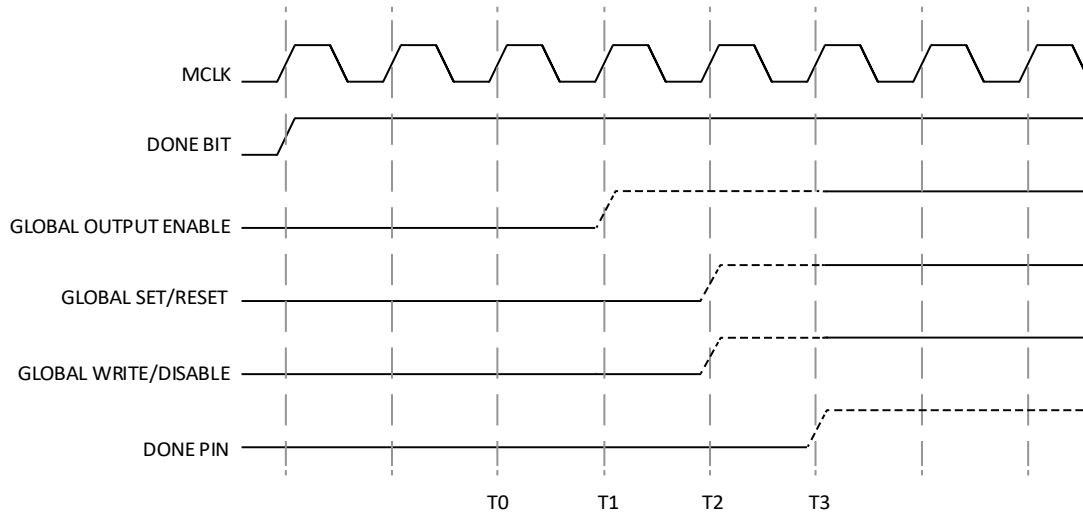
Figure 7.1. Wake-up Sequence Using Internal Clock
