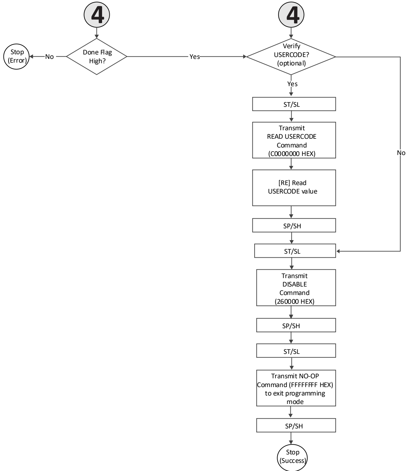
Figure 8.3. MachXO3 Slave SPI/I 2 C SRAM Configuration Flow
