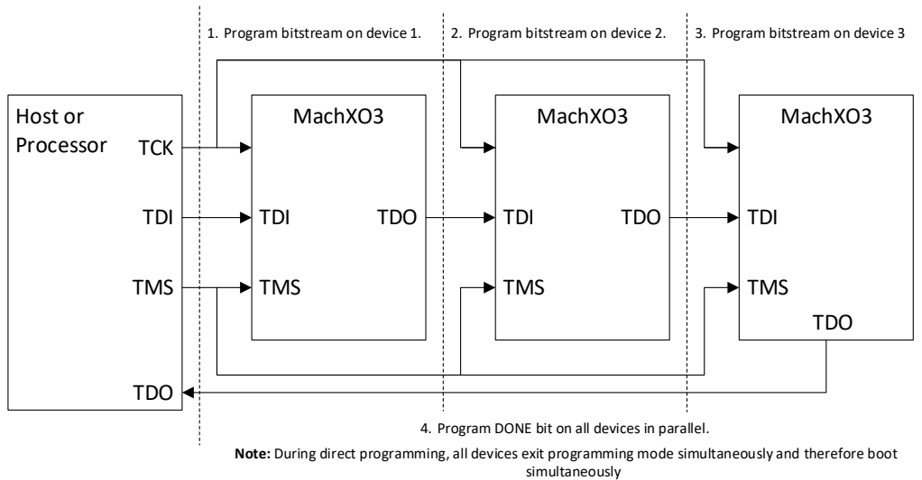
Figure 8.17. Turbo Mode Programming
