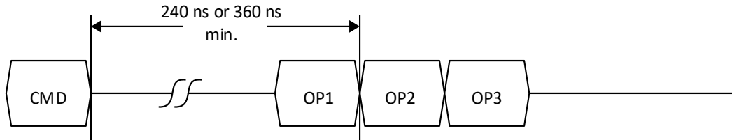
Figure 8.7. Retrieval Delay Timing Requirement for Single-Page Reads
