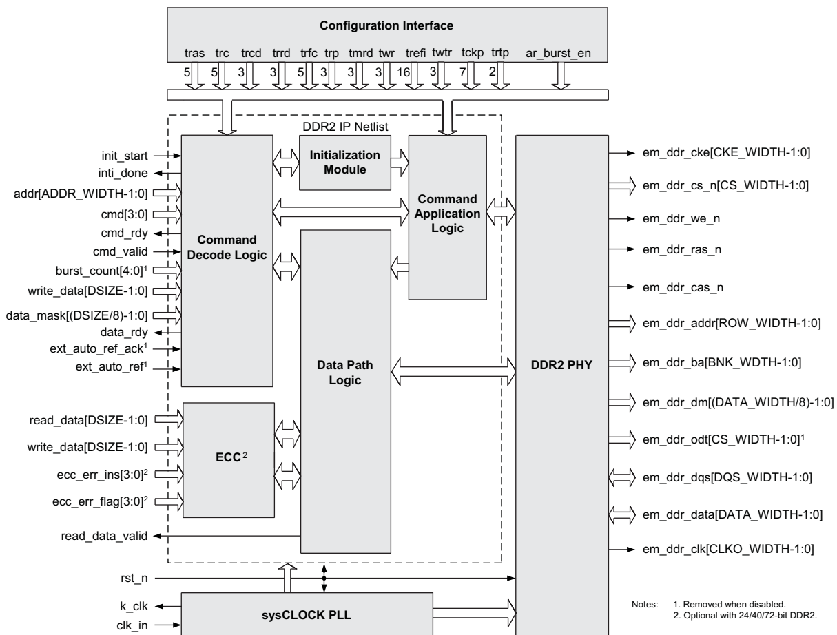
Figure 2-1. DDR2 SDRAM Controller Block Diagram
