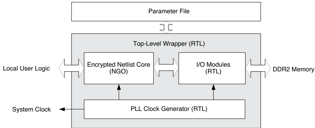
Figure 4-4. Structure of the DDR2 SDRAM Controller IP Core
