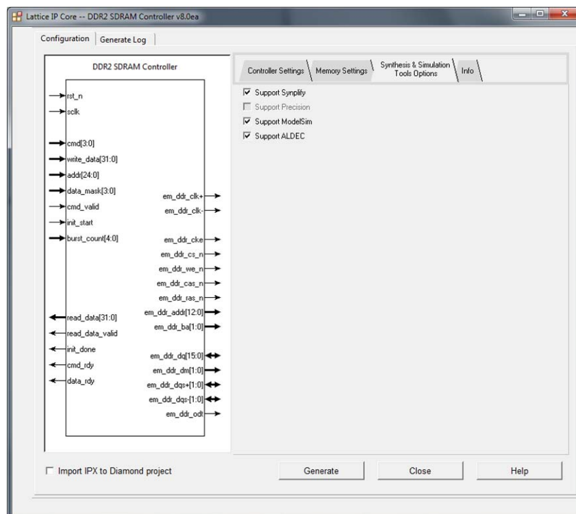
Figure 3-3. Synthesis & Simulation Tools Option Tab
