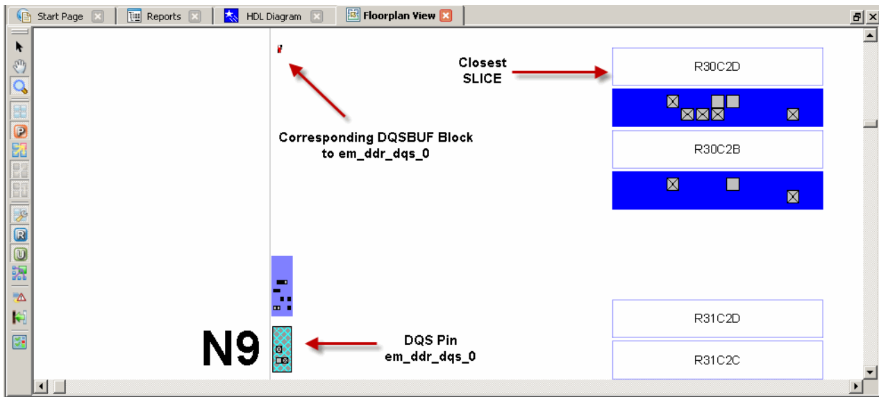
Figure 5-2. Diamond Floorplan View
