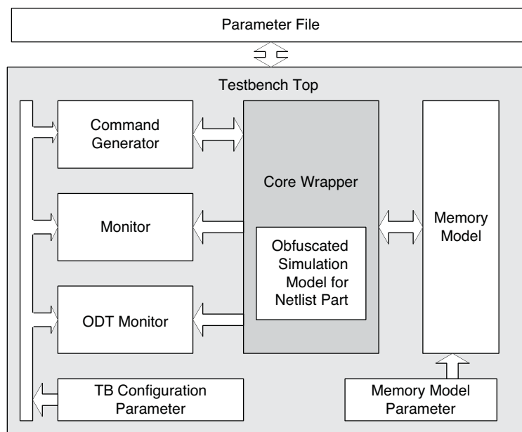
Figure 4-5. Simulation Structure for DDR2 SDRAM Controller IP Core Evaluation
