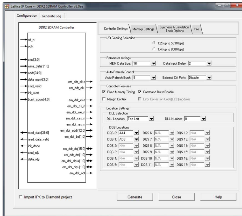
Figure 3-1. DDR2 SDRAM Controller IP Core Controller Settings
