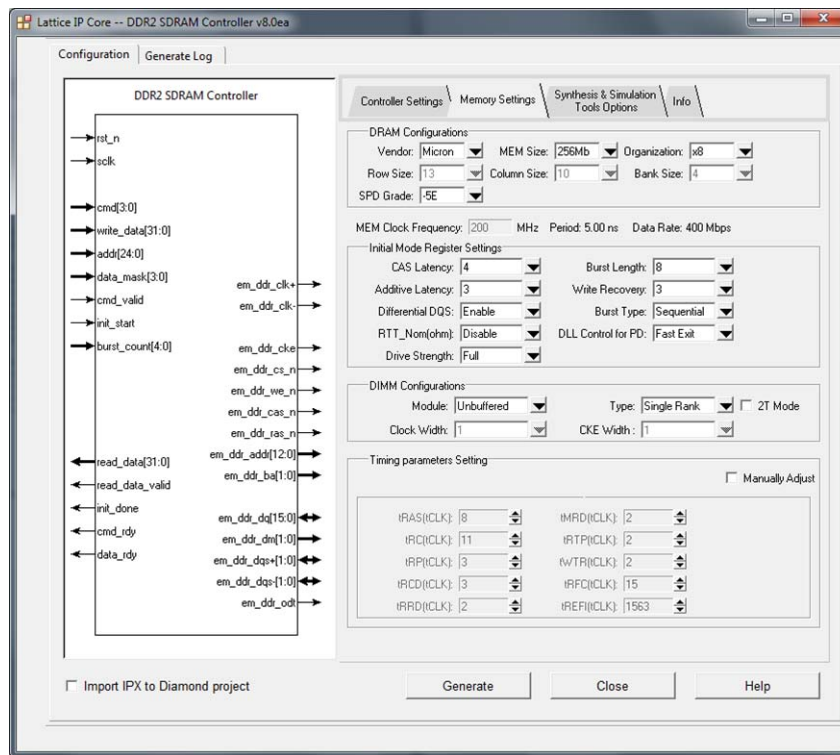
Figure 3-2. DDR2 SDRAM Controller IP Core Memory Settings
