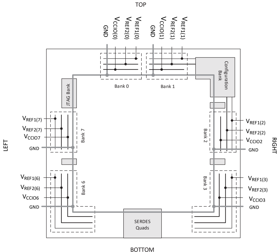
Figure 3.7. LatticeECP3 Banks
