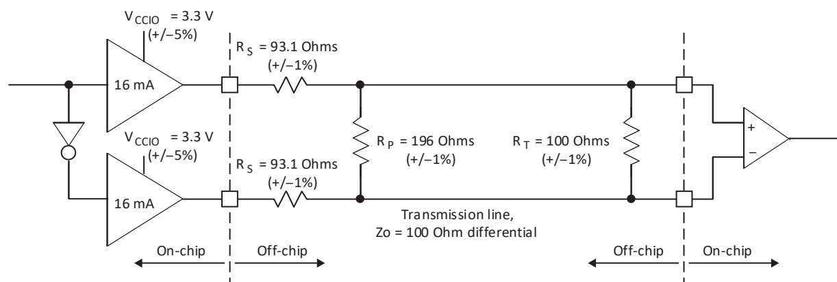
Figure 4.3. Differential LVPECL33
