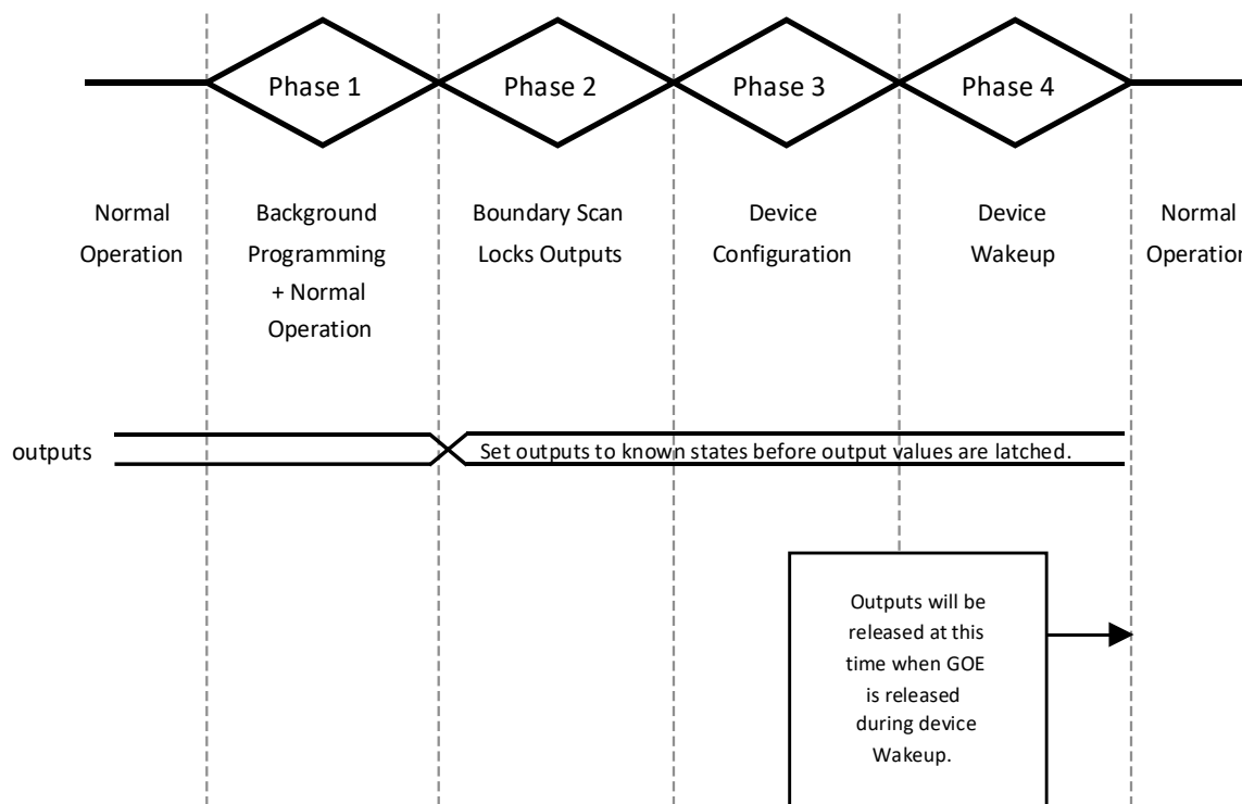
Figure 4.3. Example Non-JTAG Mode TransFR Sequence
