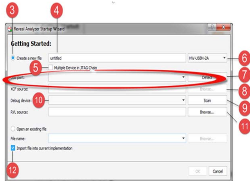
Figure 2: Startup Wizard with Steps for a New File
