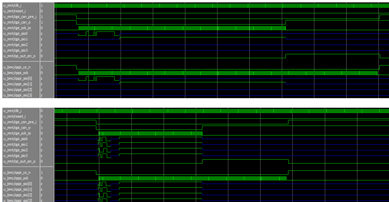
Figure 2.6. Illegal Read Command (3-Byte Address, Incremental Address Overflow)
