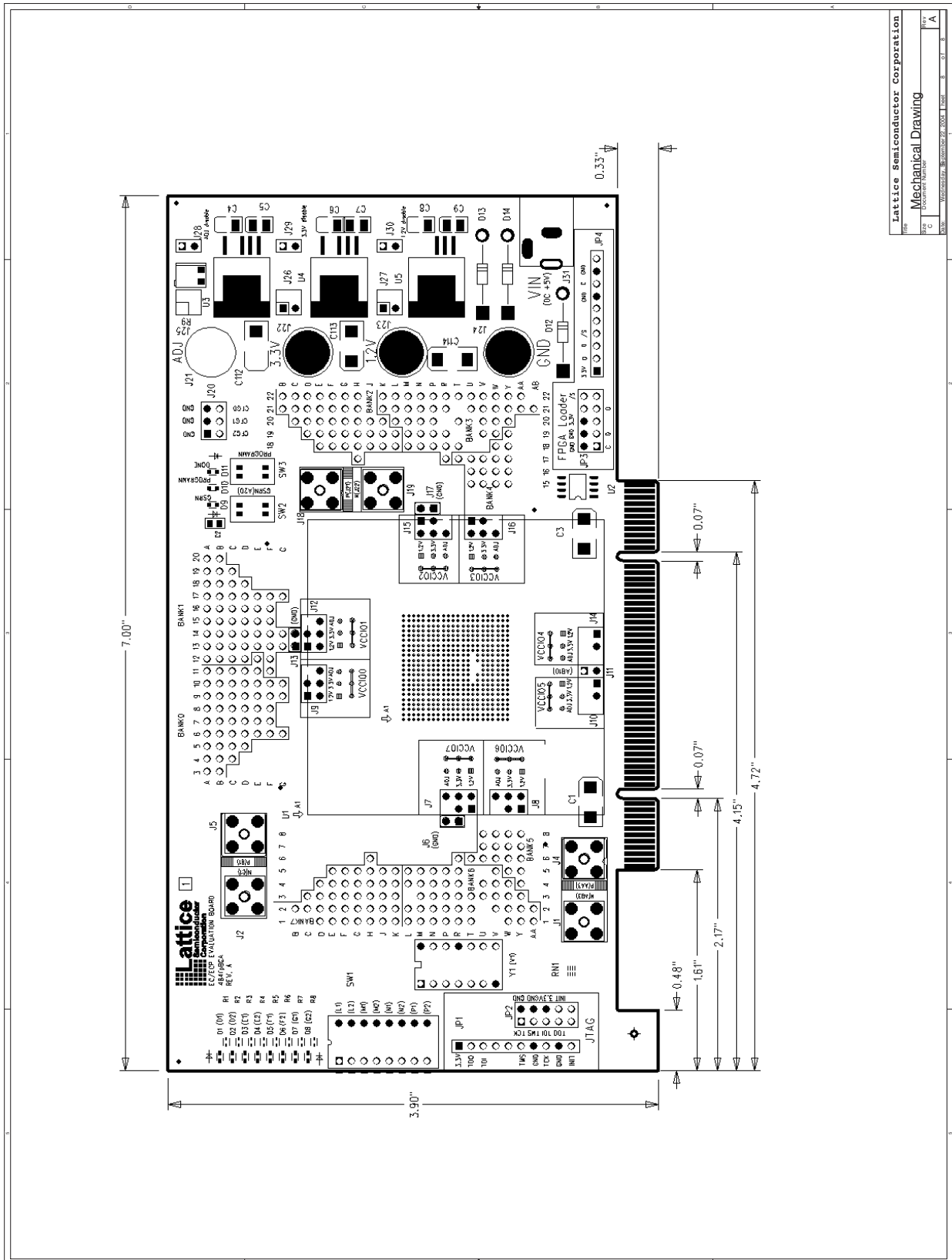
Figure 15. Mechanical Drawing
