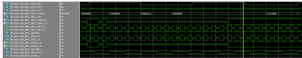
Figure 3.6. Simulation Waveform
