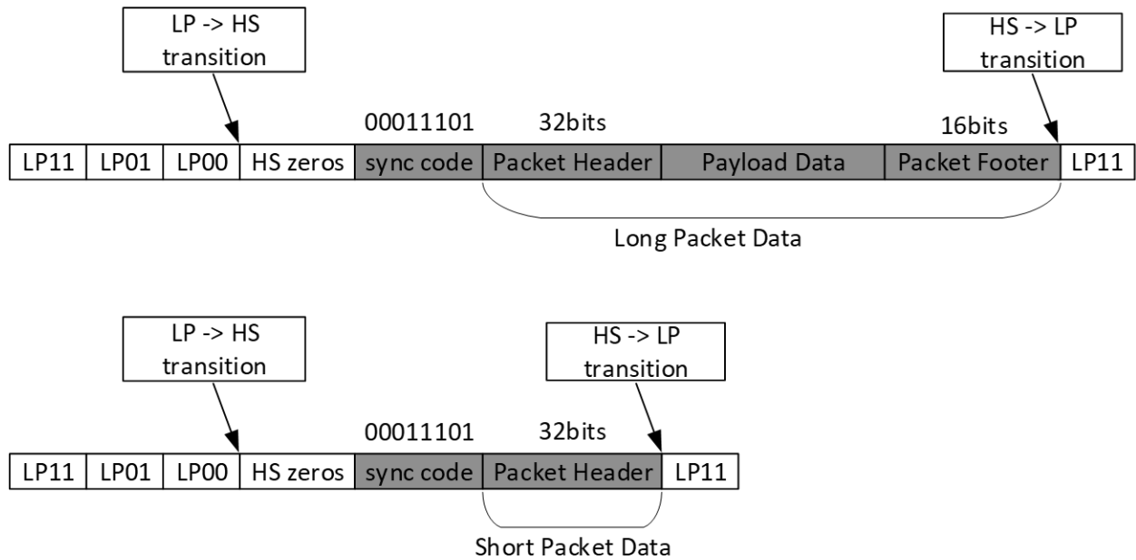
Figure 2.2. High-Speed Entry Sequence and Payload Data Transmission Cycle on Data Lanes
