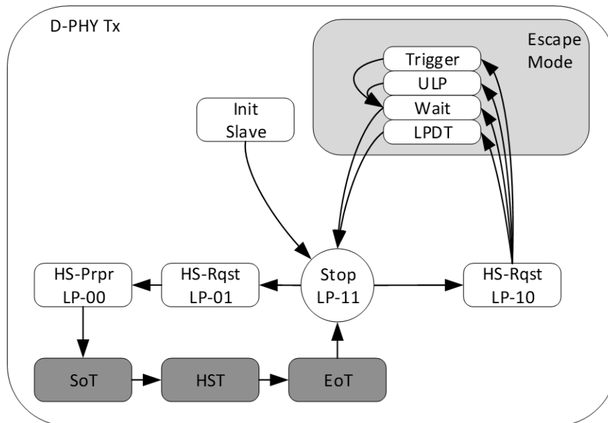
Figure 2.1. MIPI D-PHY Tx LP to HS Transition Flow Diagram on Data Lanes
