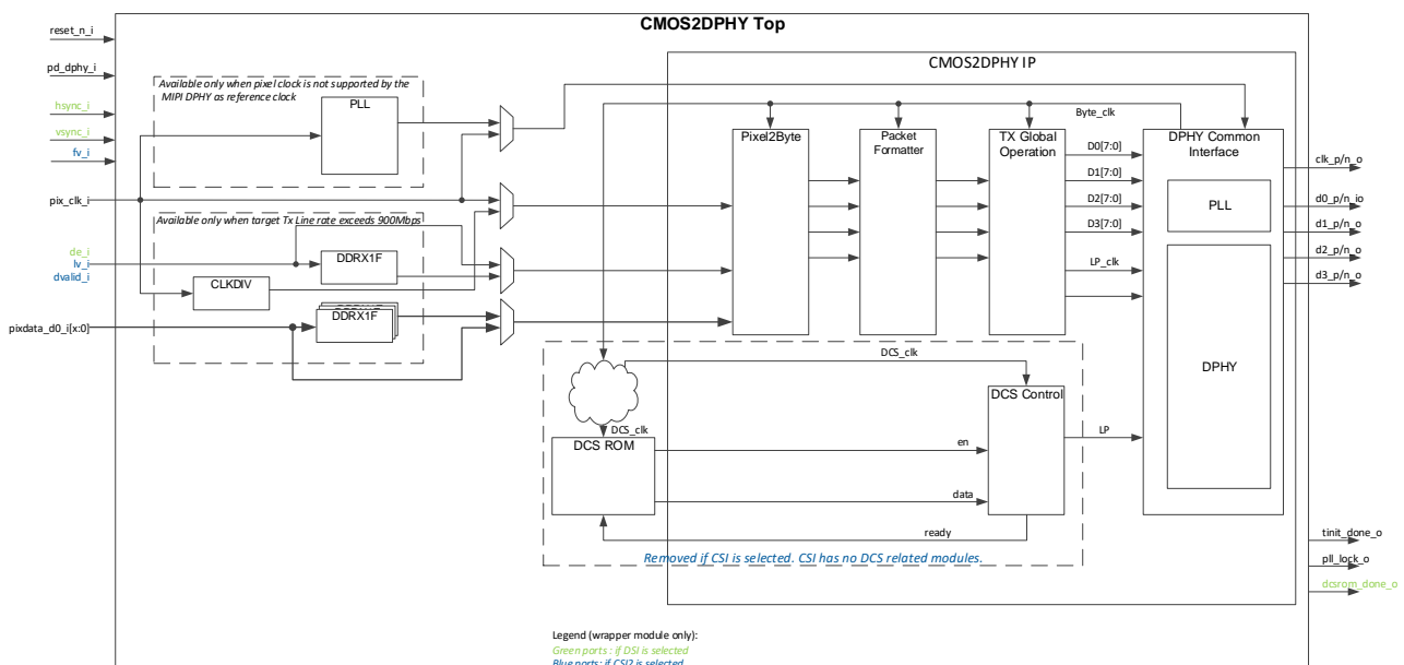
Figure 2.3. Top Level Block Diagram
