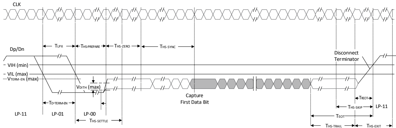
Figure 2.4. High-Speed Data Transmission Timing Diagram
