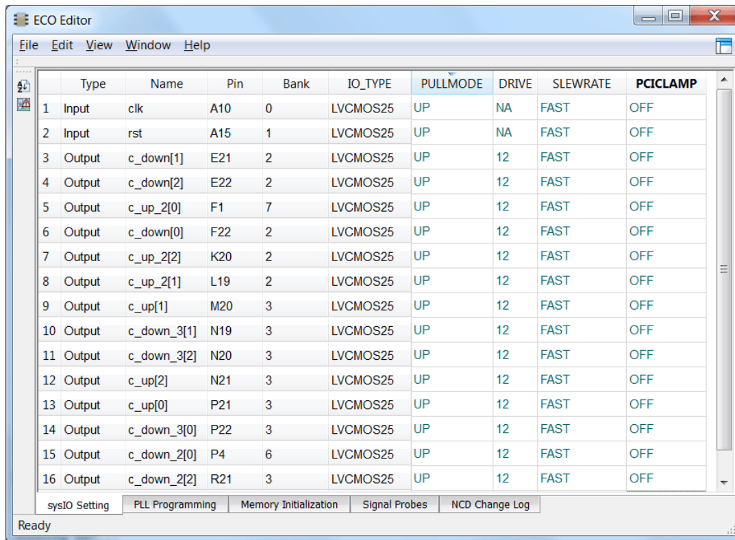
Figure 118: ECO Editor
