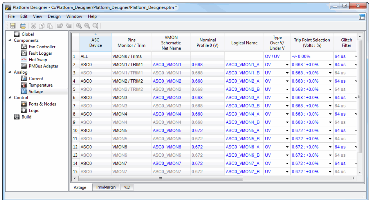
Figure 94: Platform Designer
