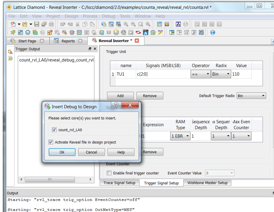
Figure 98: Insert Debug
