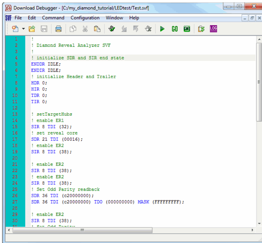
Figure 122: Download Debugger
