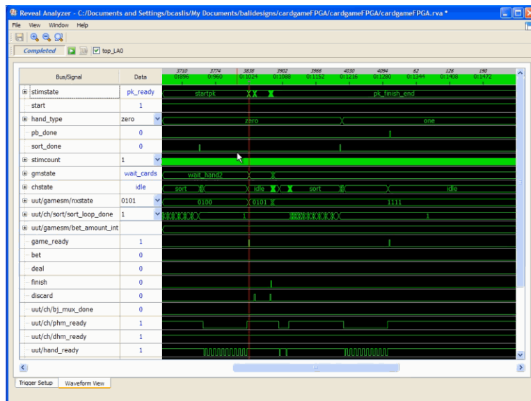
Figure 101: Reveal Analyzer Waveform View
